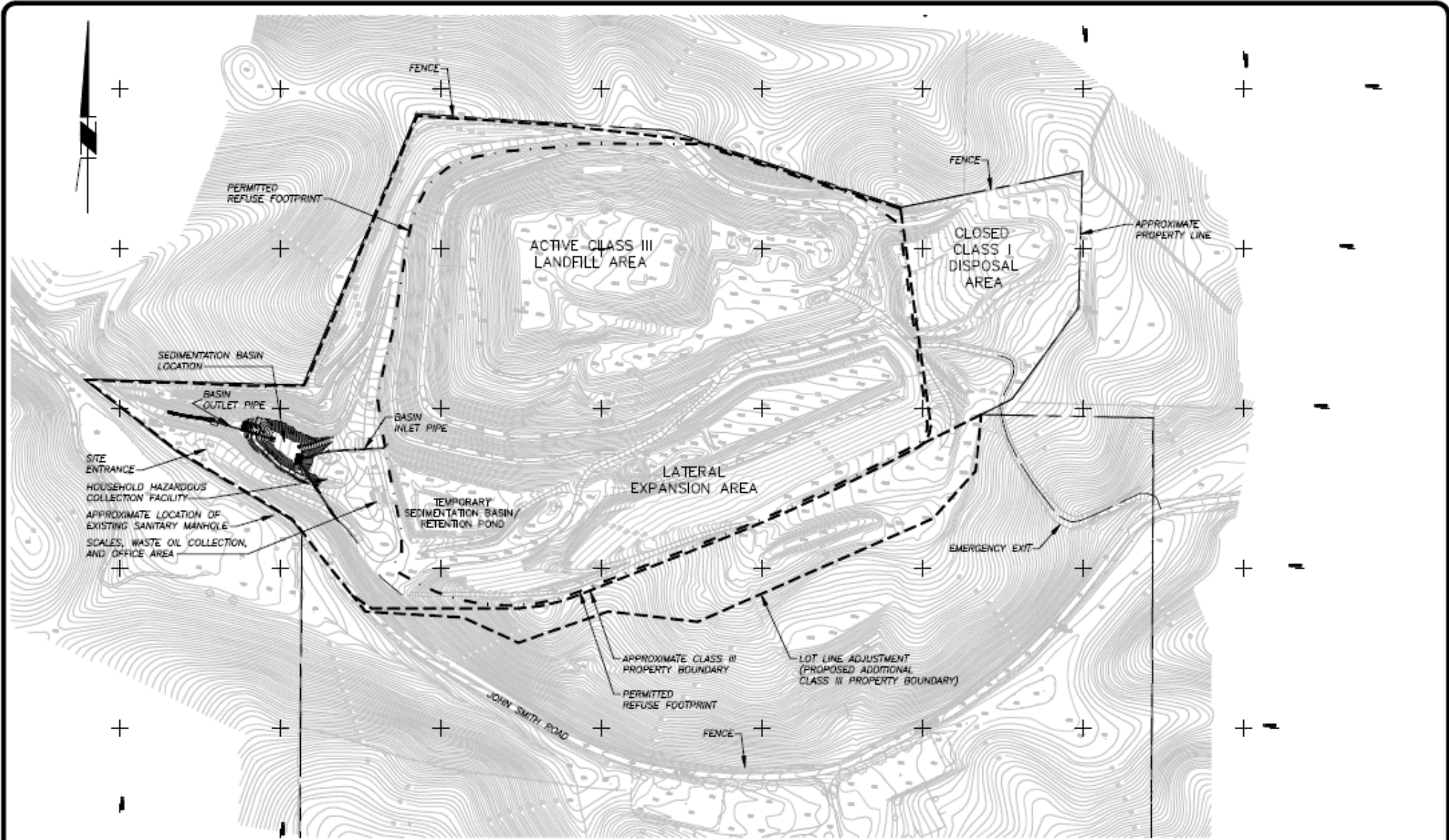
Figure 2 Landfill Permitted Refuse Footprint
