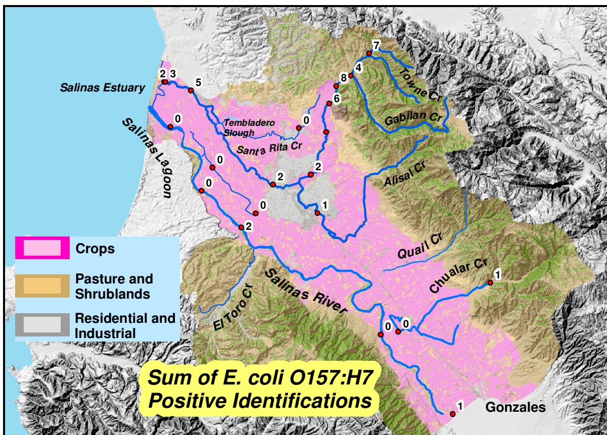
Figure 3-5. Sum of E. coli O157:H7 positives.
