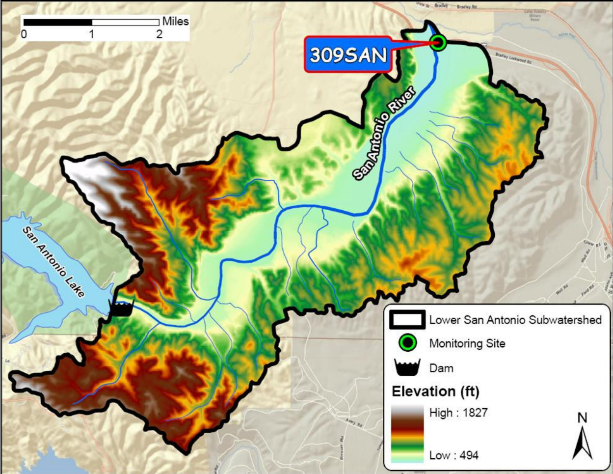
Figure 2-1. Lower San Antonio River subwatershed relief map.
