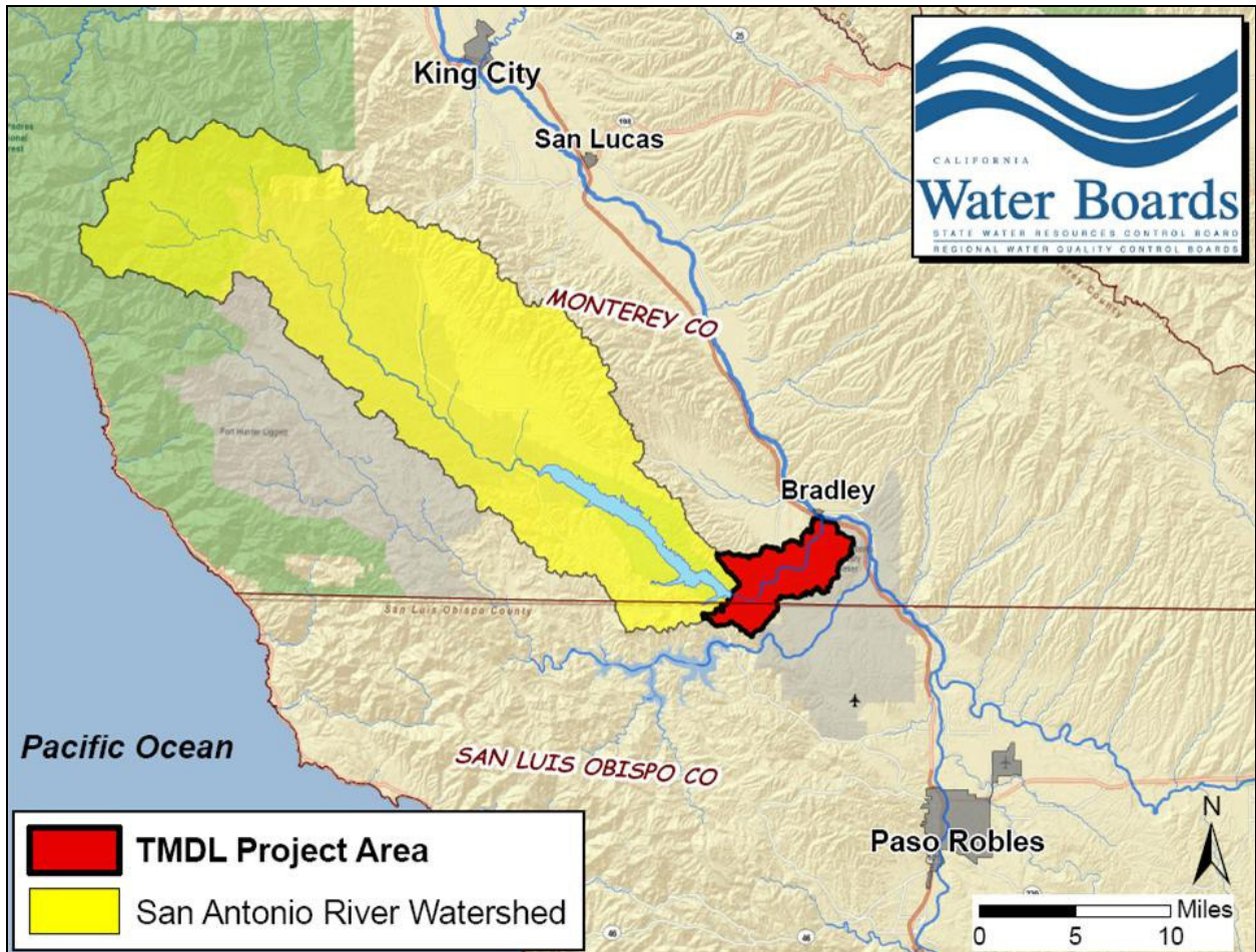
Figure 1-1. TMDL Project Area – Lower San Antonio River subwatershed.
