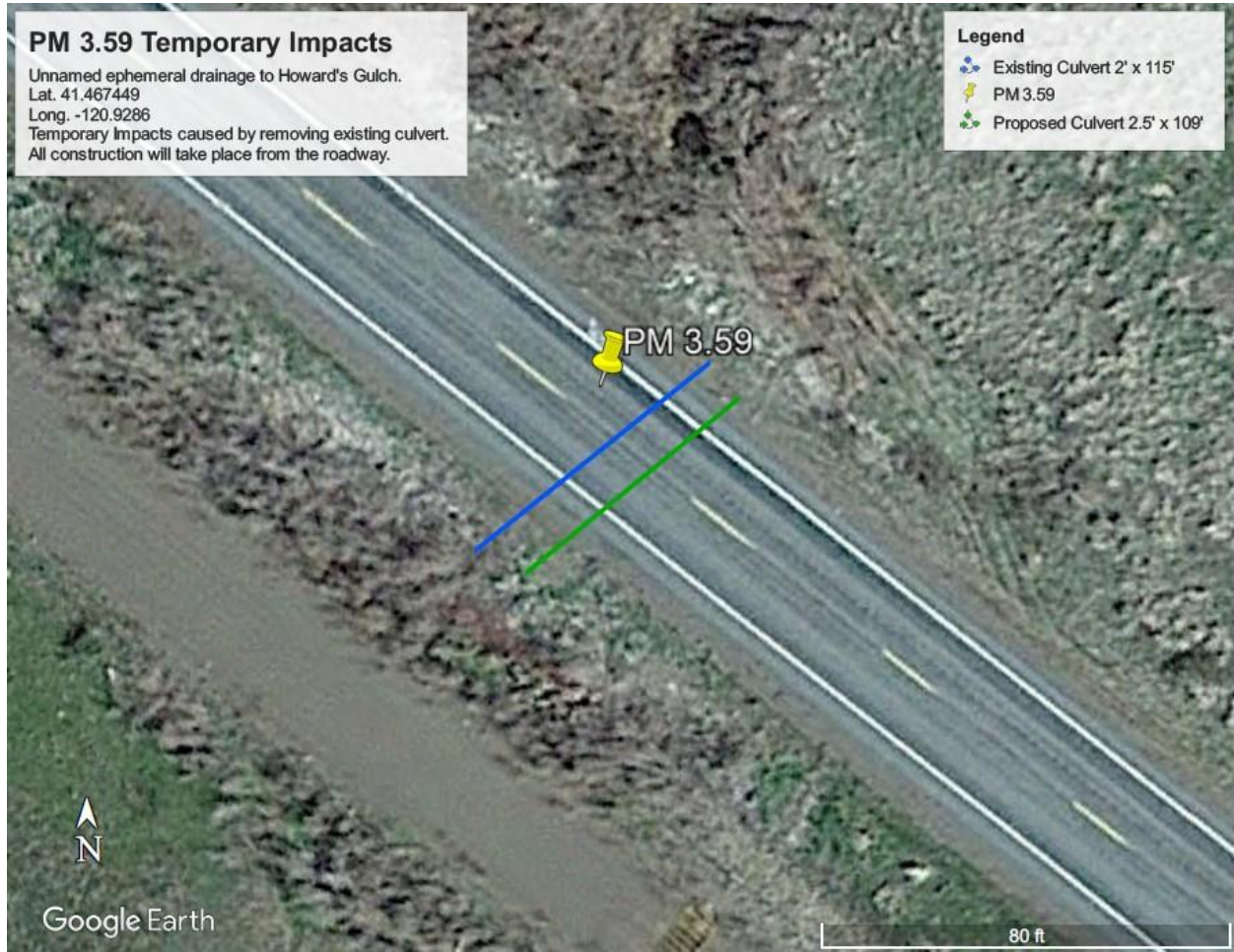
Figure 2. Culvert 1 Impacts Map
