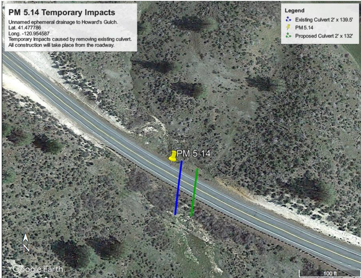
Figure 3. Culvert 3 Impacts Map
