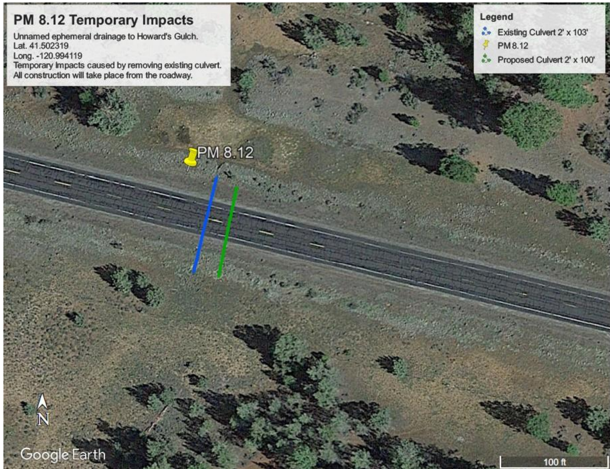
Figure 5. Culvert 5 Impacts Map
