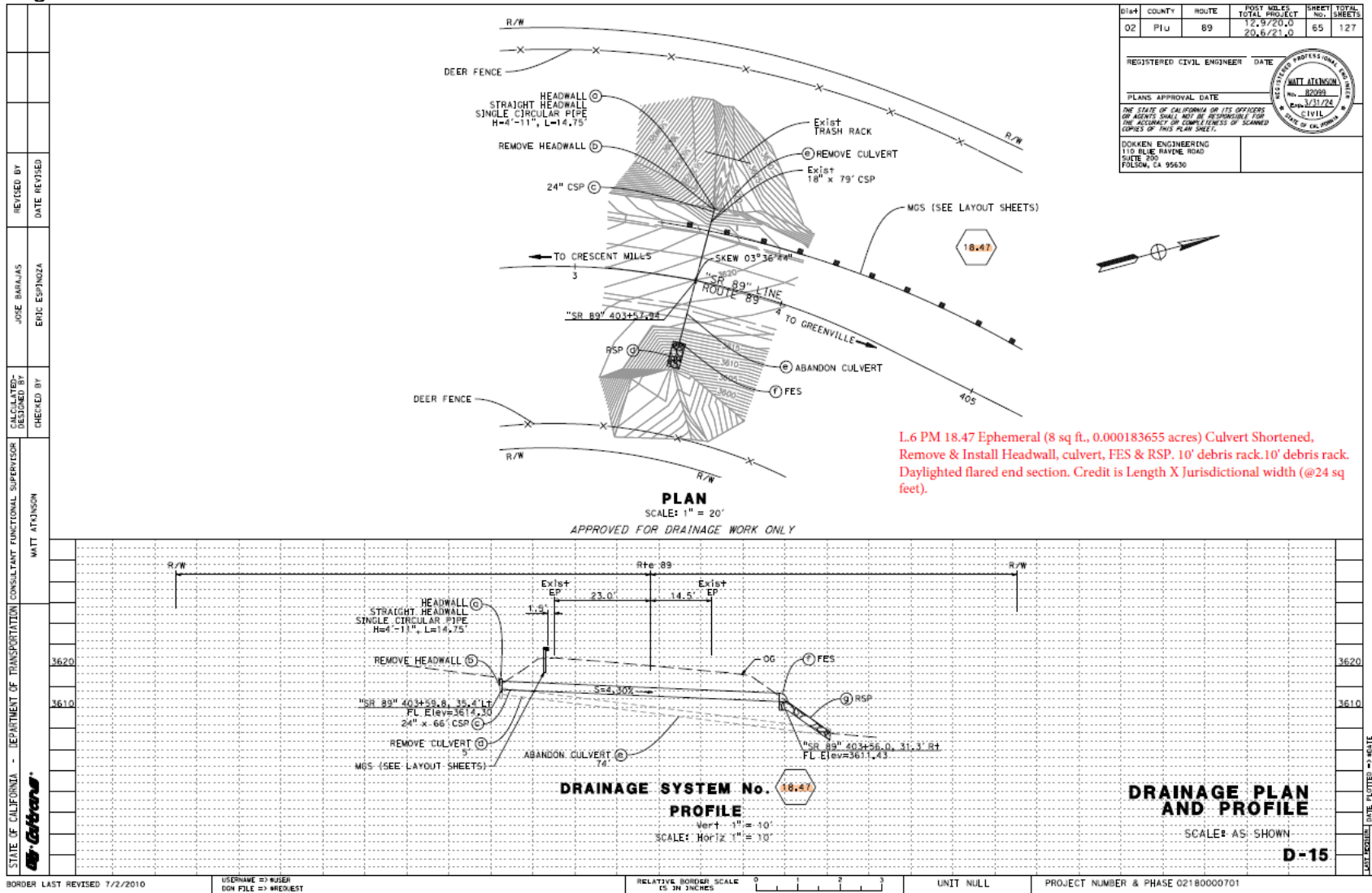
Figure 7: Culvert PM 18.47 Location
