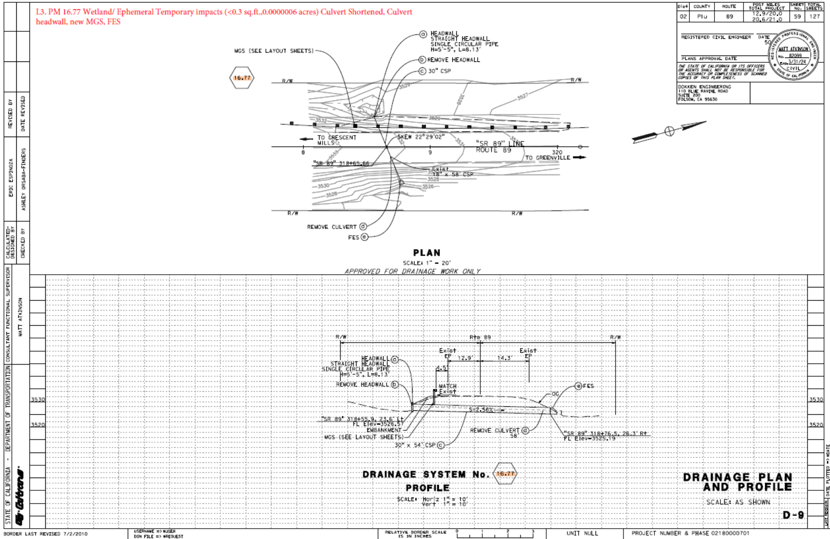
Figure 4: Culvert PM 16.77 Location
