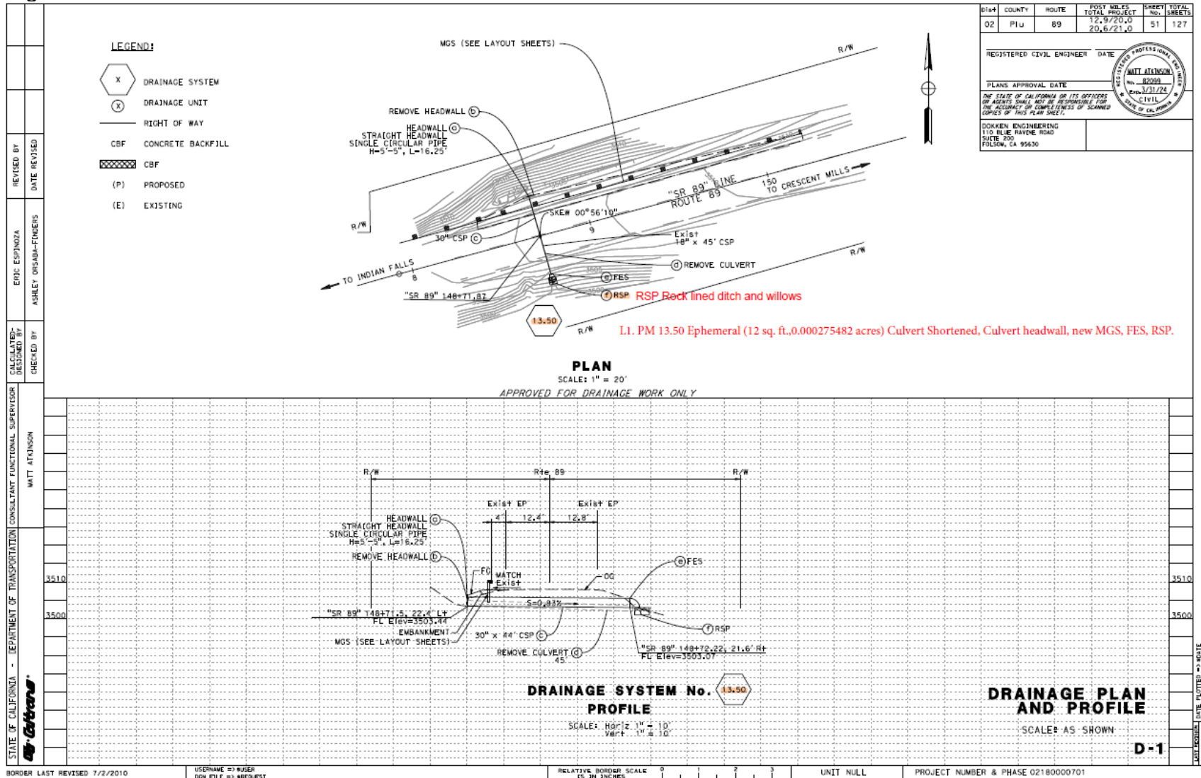
Figure 2: Culvert PM 13.50 Location
