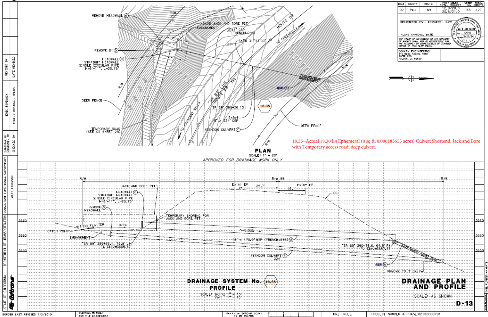
Figure 5: Culvert PM 18.30 Location
