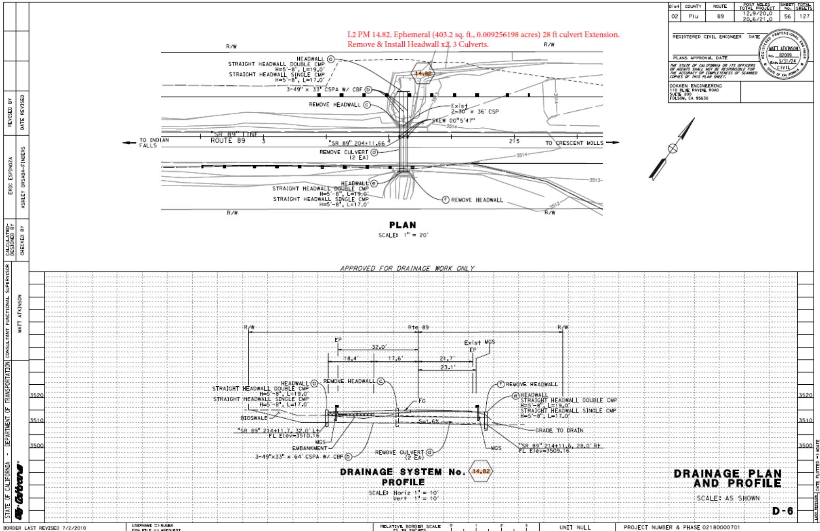
Figure 3: Culvert PM 14.82 Location
