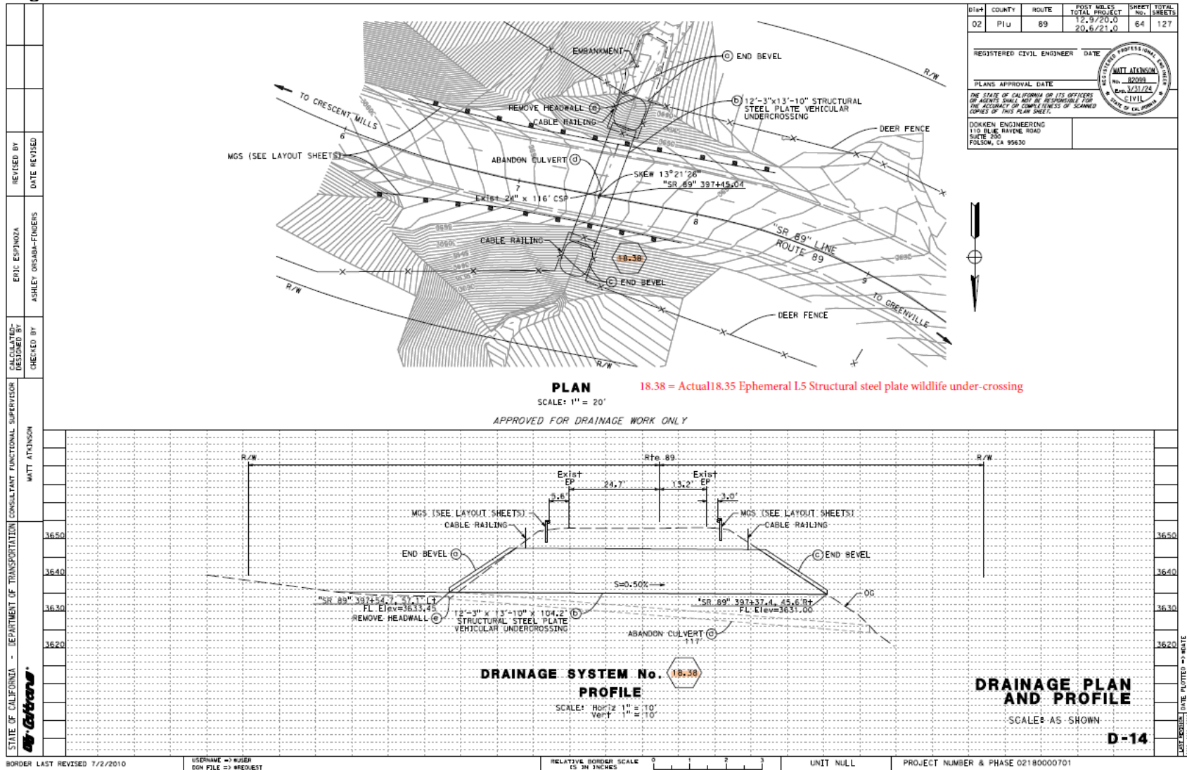
Figure 6: Culvert PM 18.35 Location
