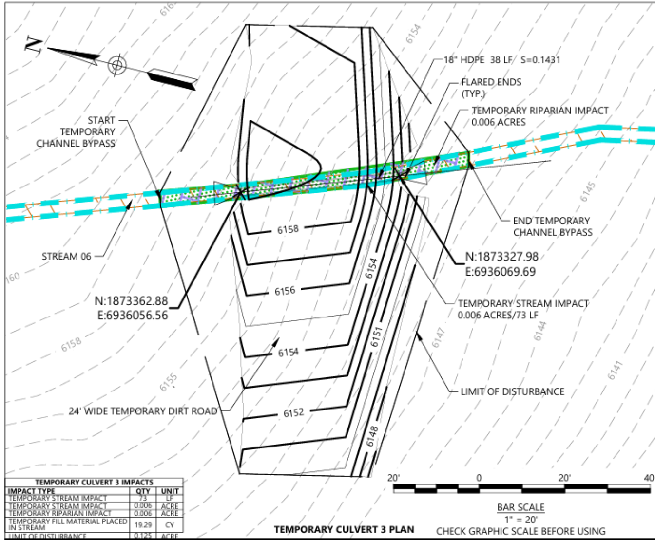
Figure 6. Temporary Culvert 3 Location and Impacts
