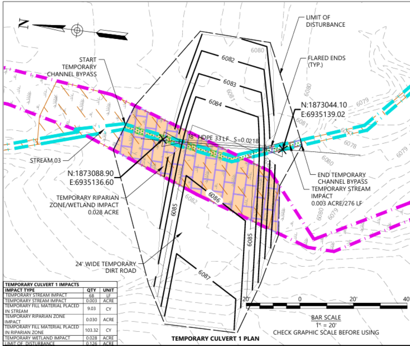
Figure 4. Temporary Culvert 1 Location and Impacts
