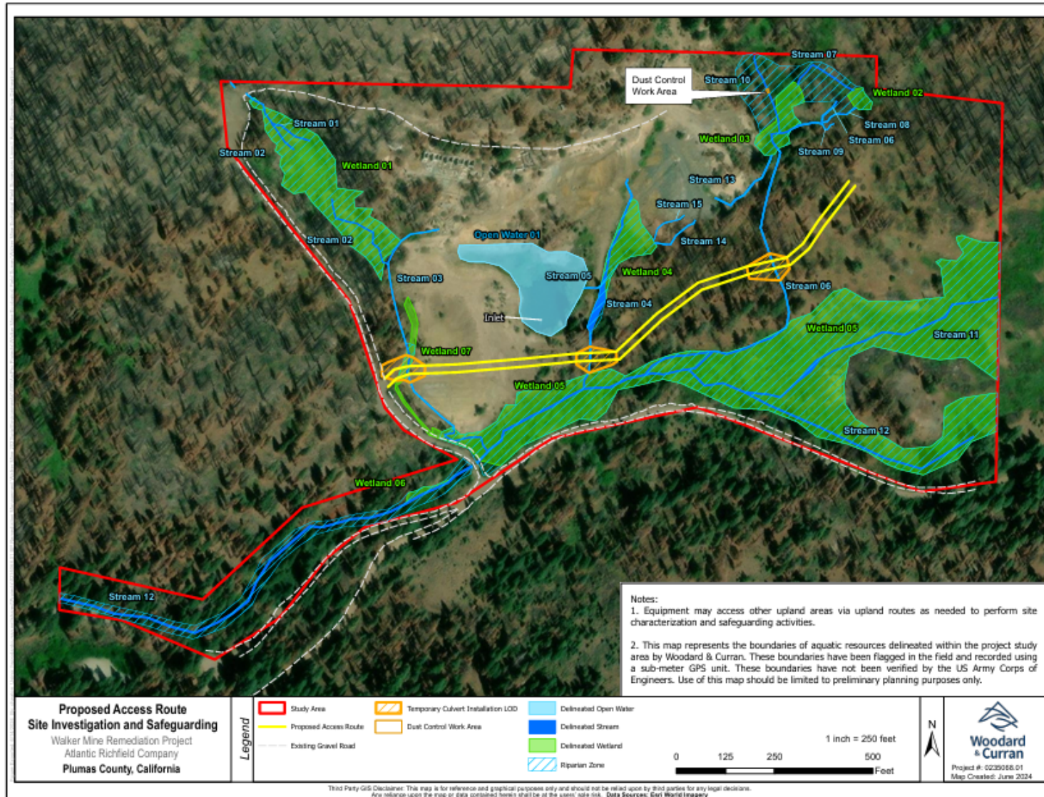
Figure 3. Temporary Impact Locations and Proposed Access Route
