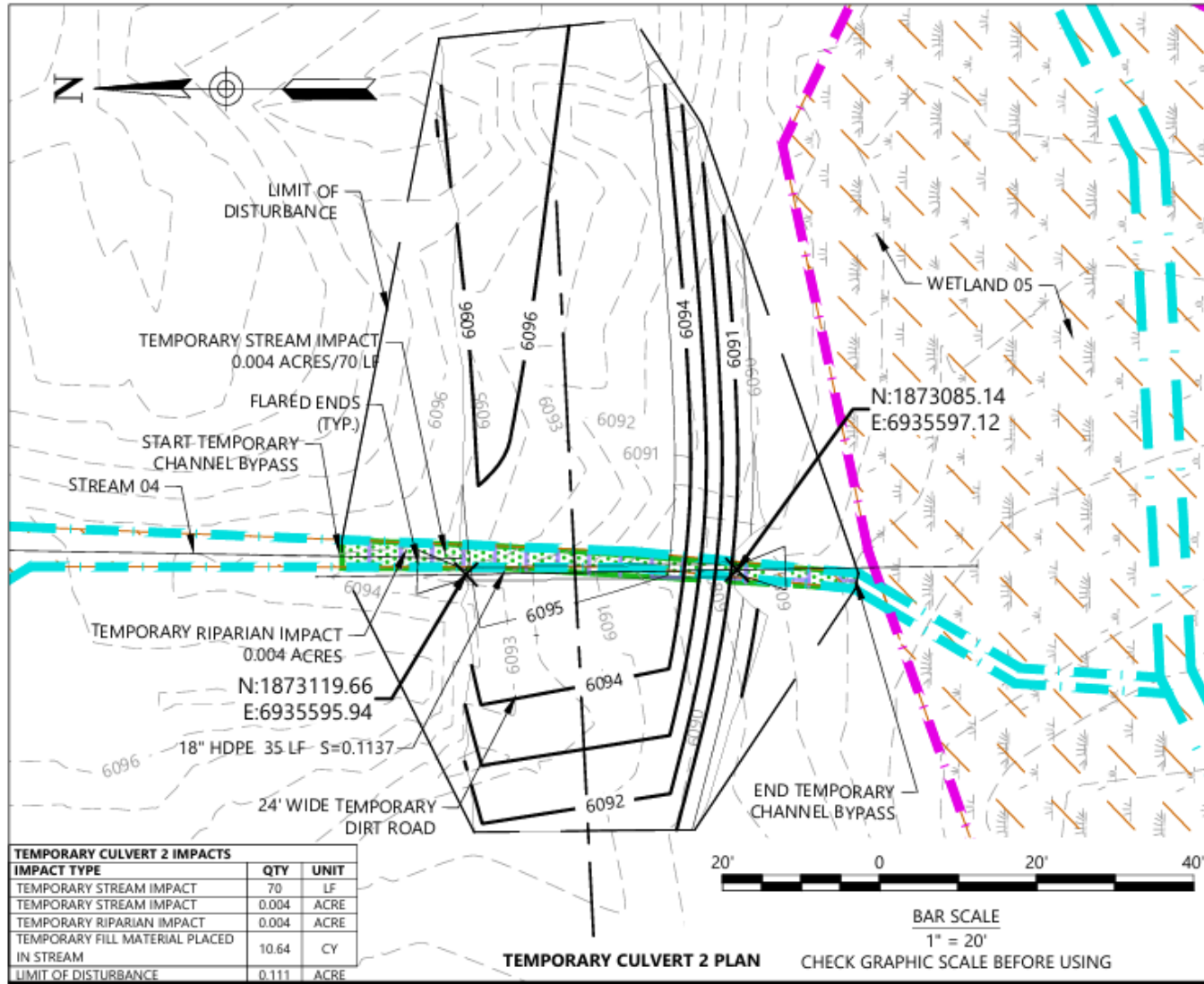
Figure 5. Temporary Culvert 2 Location and Impacts
