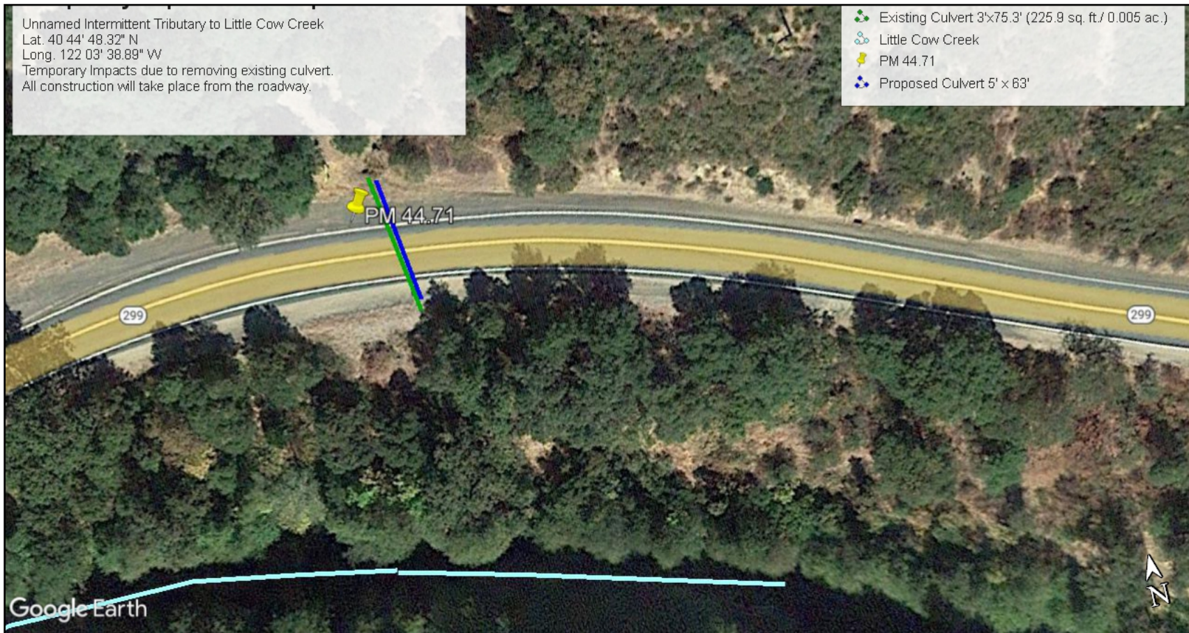
Figure 3. Impacts - Location 4 (PM 44.71).
