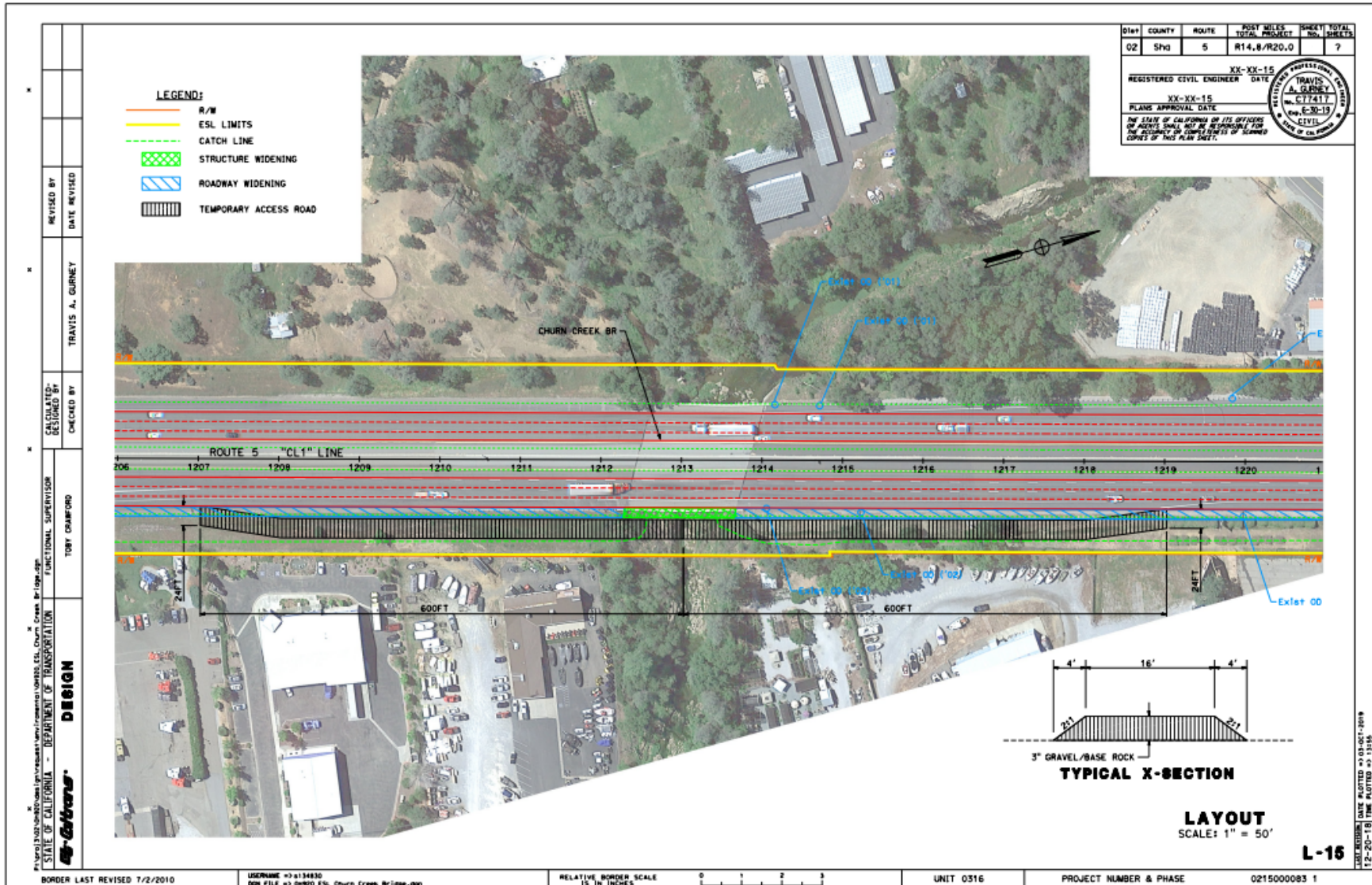
Figure 3: Churn Creek Bridge Layout
