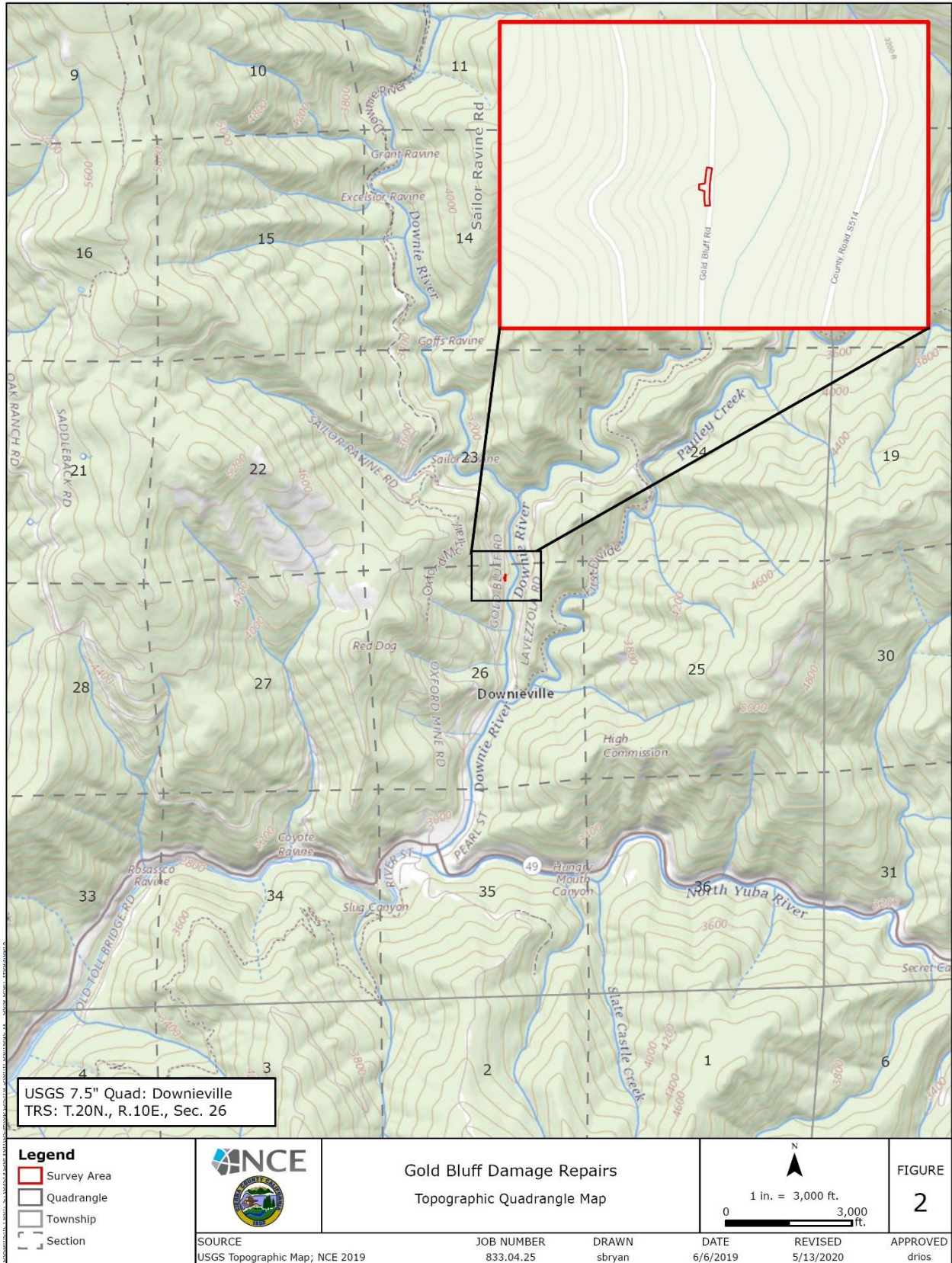
Figure 2 – Site Topographic Map
