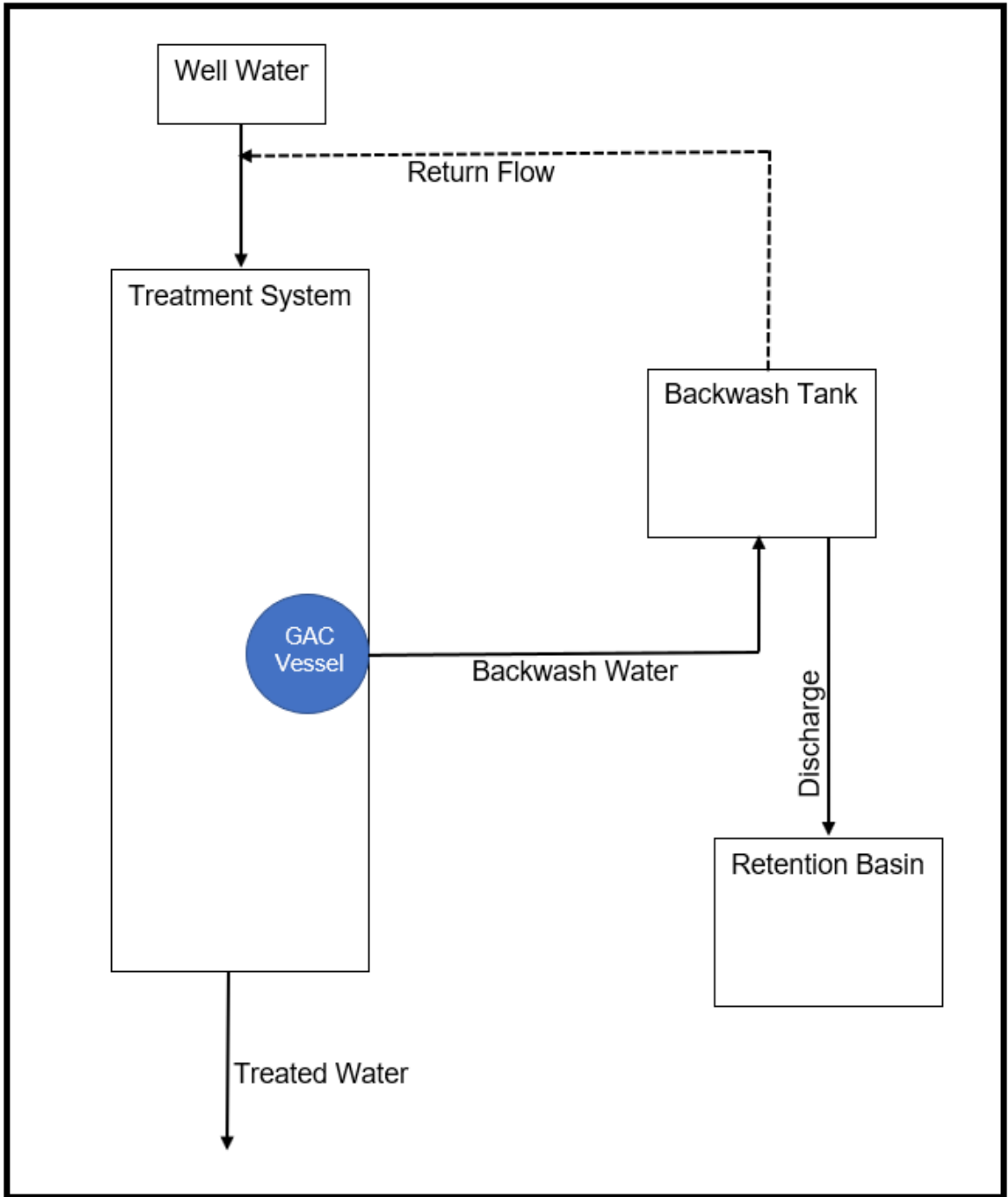
Design Reference: Conceptual representation of backwash cycle
