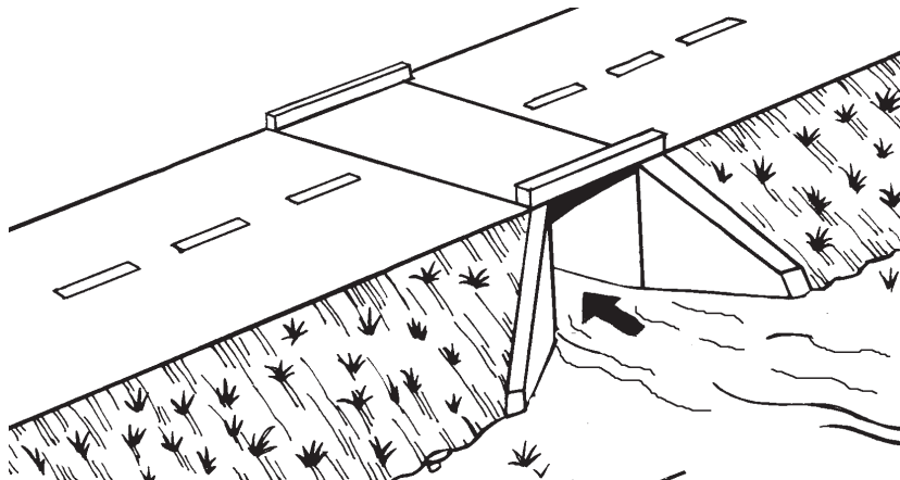
b. Concrete box culvert with concrete wingwalls for inlet/outlet protection and fill retention.
