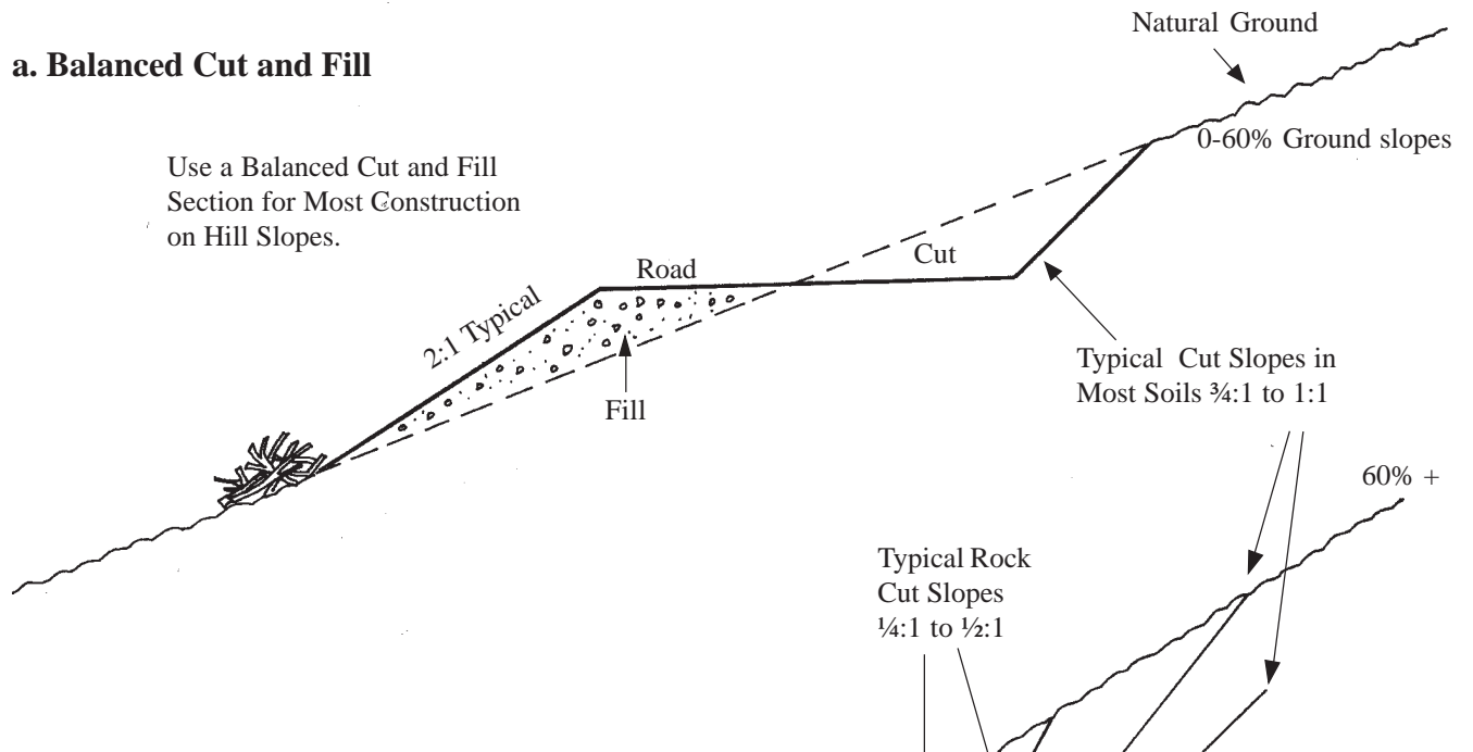
Figure 11.1 Cut slope design options.
