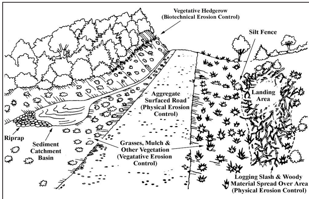
Figure (VI.1): Use of Vegetation, Woody Material and Rock for Erosion Control
