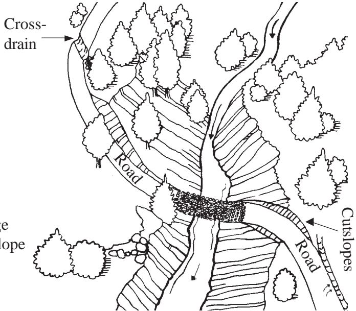
Drainage crossings perpendicular to the creek minimize the area of disturbance. Armor the stream crossing and roadway surface.
