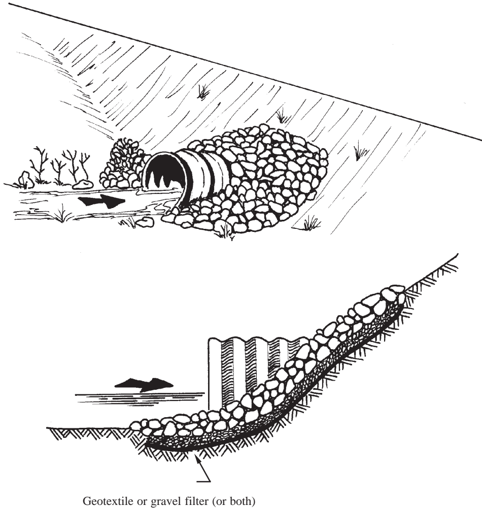
a. Normal metal culvert installation using riprap around the inlet and outlet of culverts. Also use geotextile (filter fabric) or gravel filter beneath the riprap for most installations. (Adapted from Wisconsin's Forestry Best Management Practice for Water Quality, 1995)
