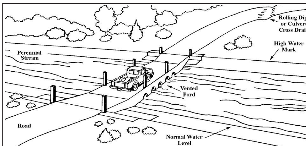
Figure (V.2) Improved, Vented Ford
