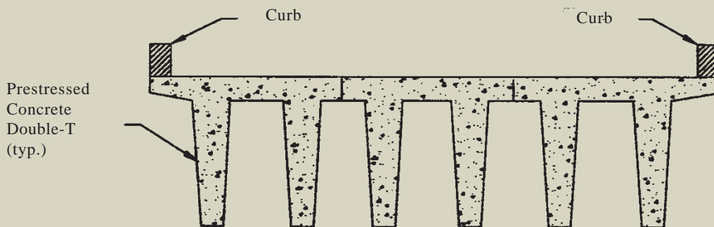
Prestressed Concrete Single or Double-T Bridge
