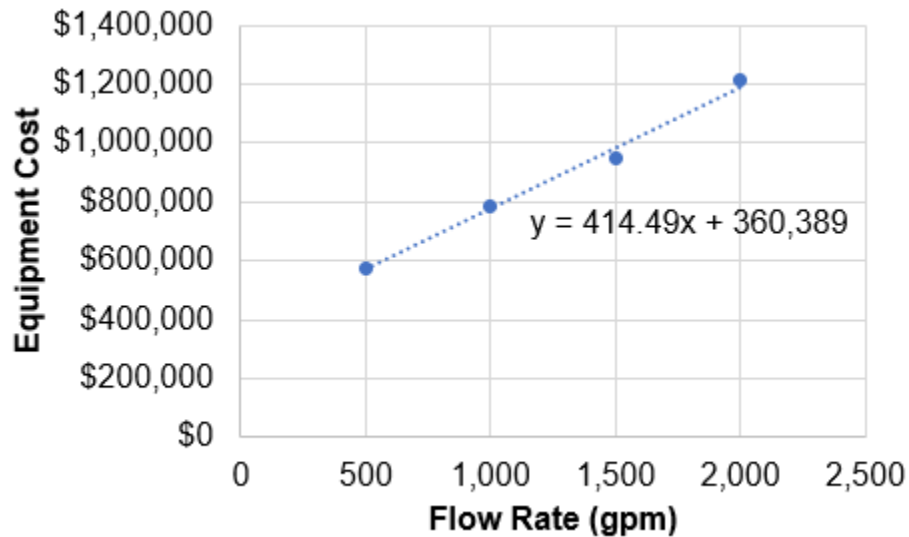
Figure 4: Arsenic Coagulation Filtration Capital Costs Regression
