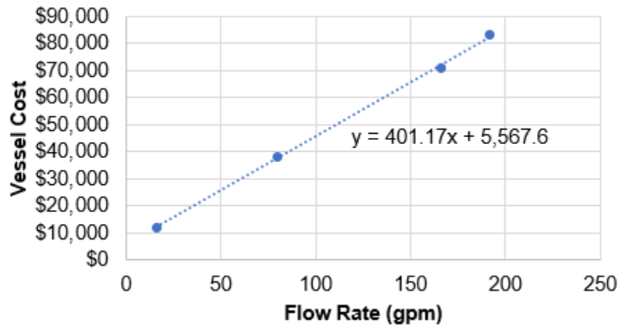
Equation 21: Filter Vessel Cost at a Given Flow Rate
