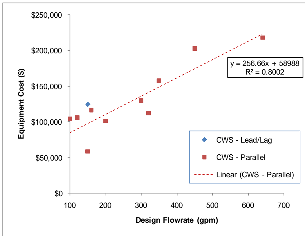
Figure 2-11. Equipment Costs of Larger AM Systems (≥100 gpm)
