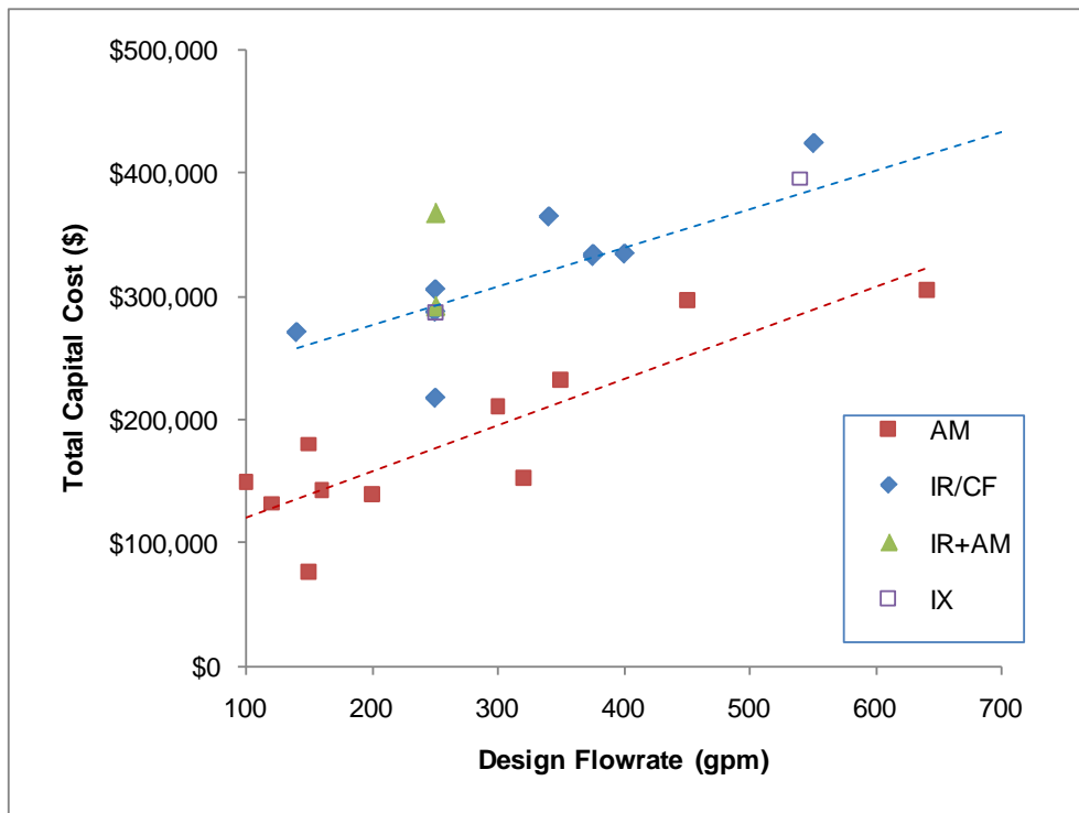
Figure 5-2. Total Capital Investment Costs of Larger AM, IR/CF, and IX Systems (≥100 gpm)
