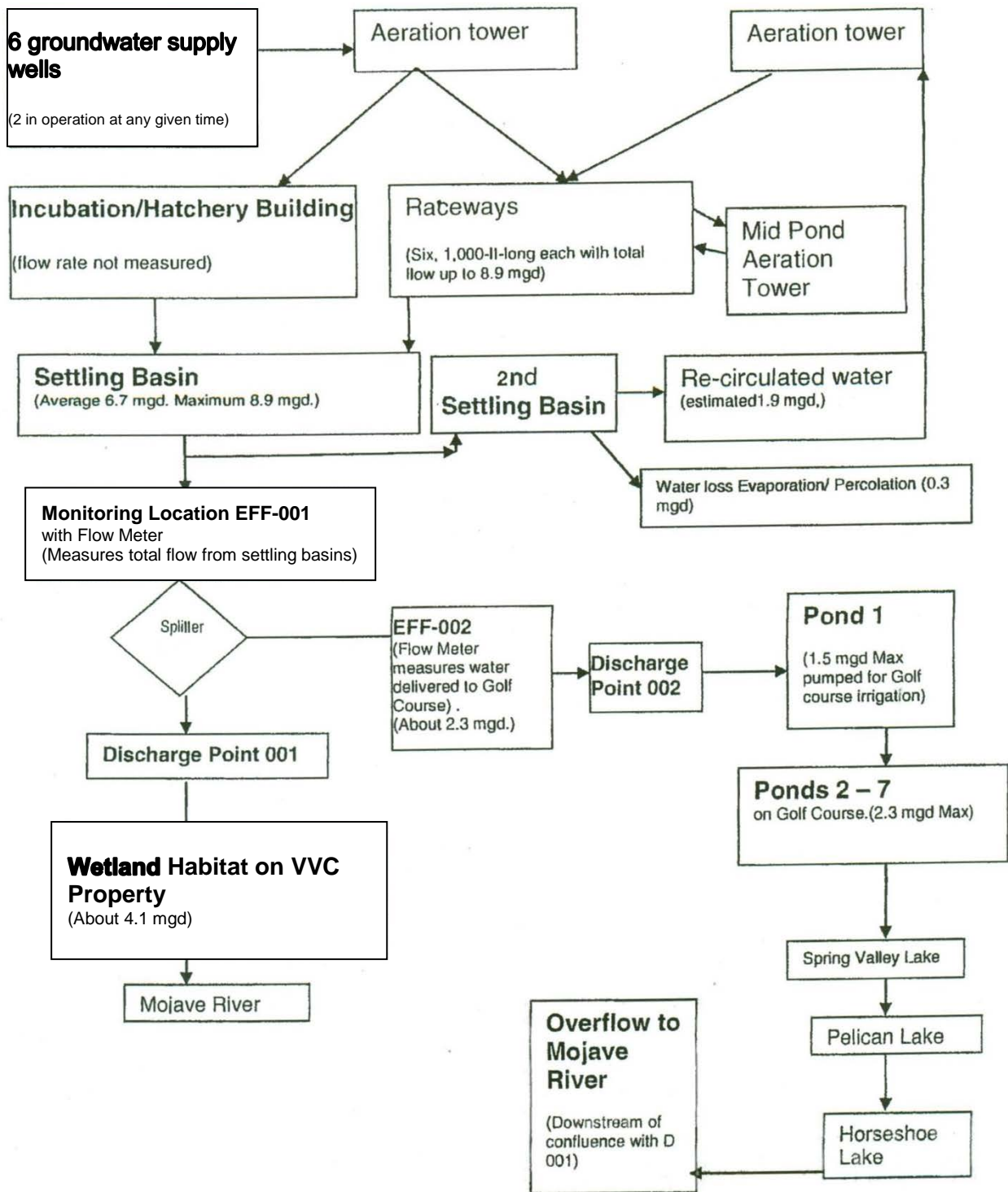
Figure C-2. Flow Diagram
