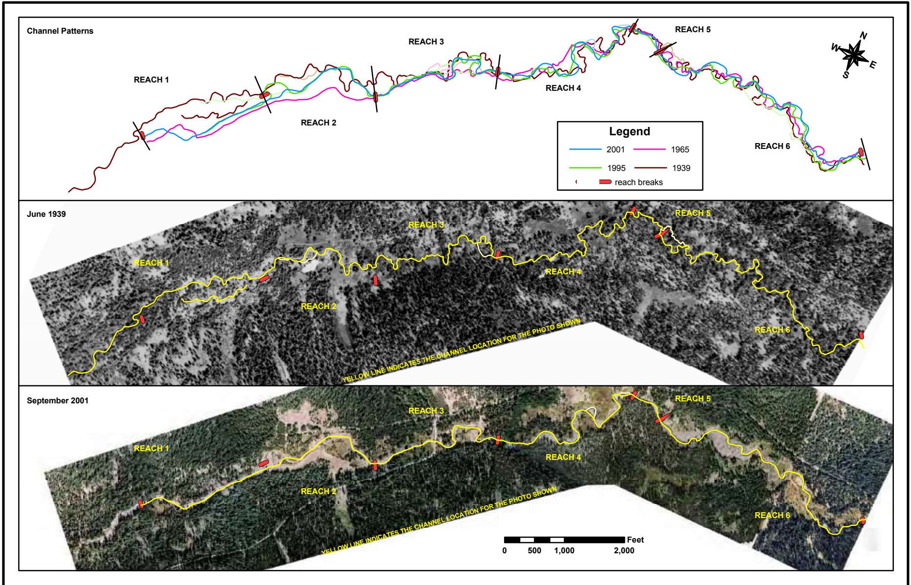
Figure 10 Historic and Current Channel Patterns of Blackwood Creek [Figure modified from Swanson (2003)]
