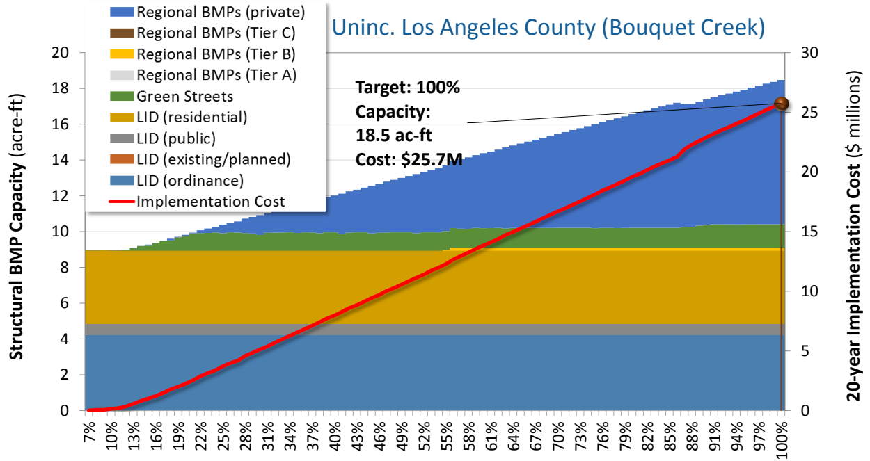
Figure C8- 7. BMP Capacities: Uninc. Los Angeles County (Bouquet Creek)
