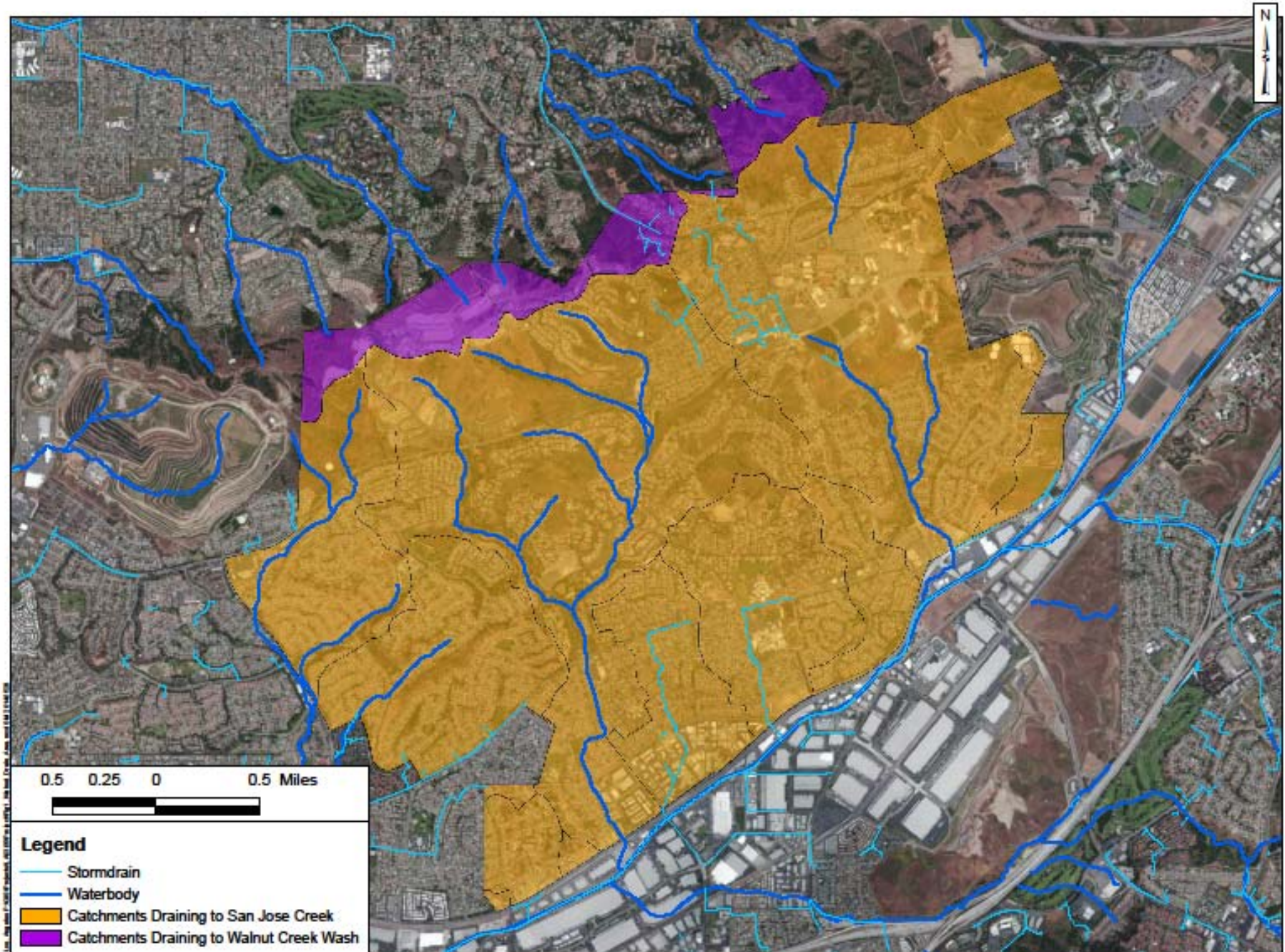
Figure 1-3: City of Walnut Drainage Areas
