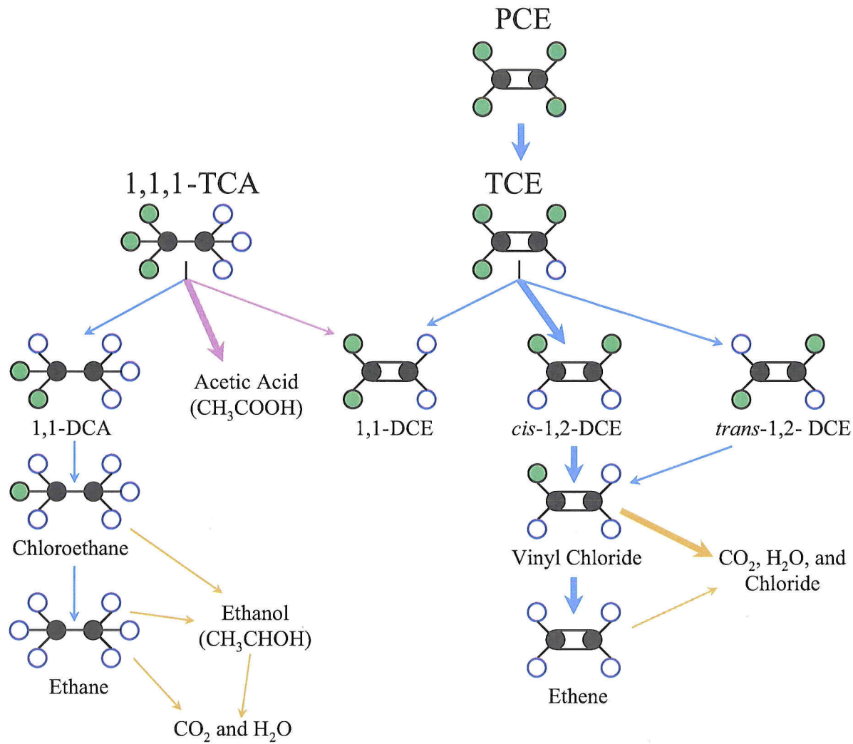
PRIMARY TRANSFORMATION PATHWAYS FOR TCA AND PCE
