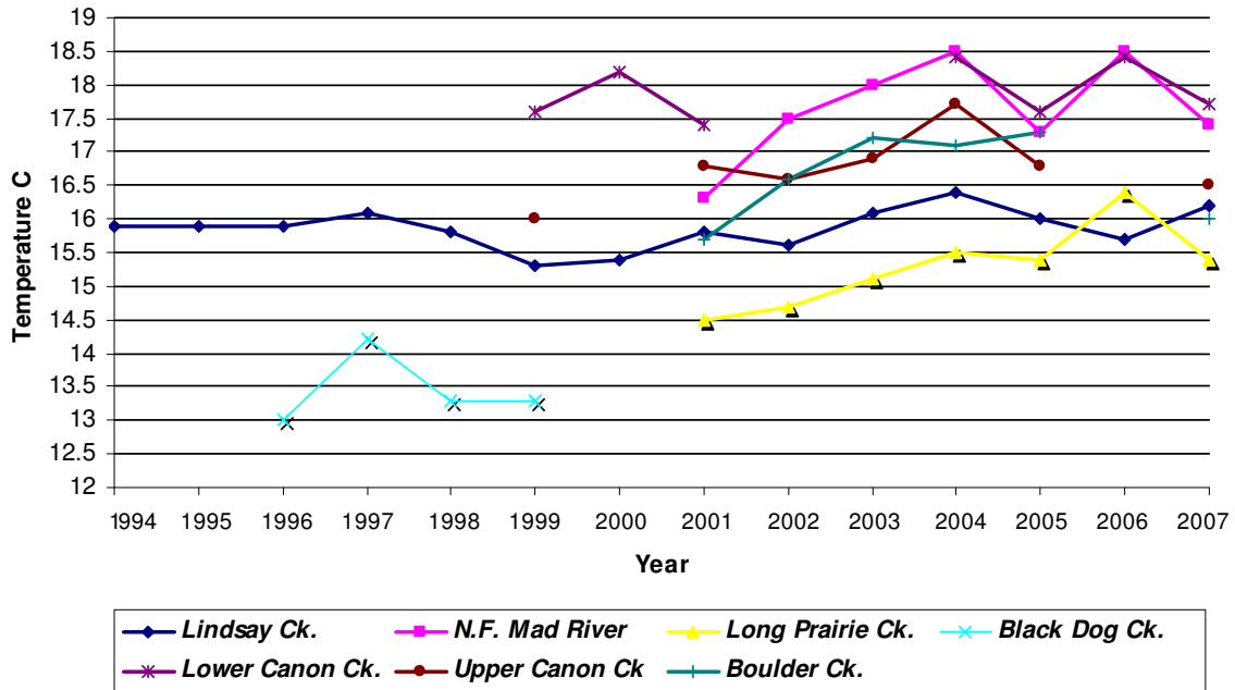
Figure 12. Maximum weekly average temperatures for selected streams within the Mad River basin.
