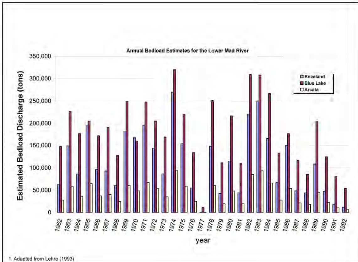
1. Adapted from Lehre (1993) Figure 4. Annual bedload estimates for the lower Mad River.
