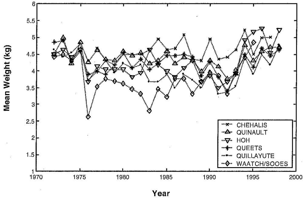
Figure A8. Mean weights of coho salmon from rivers on the outer coast of Washington State. Rivers are listed in order from south to north.
