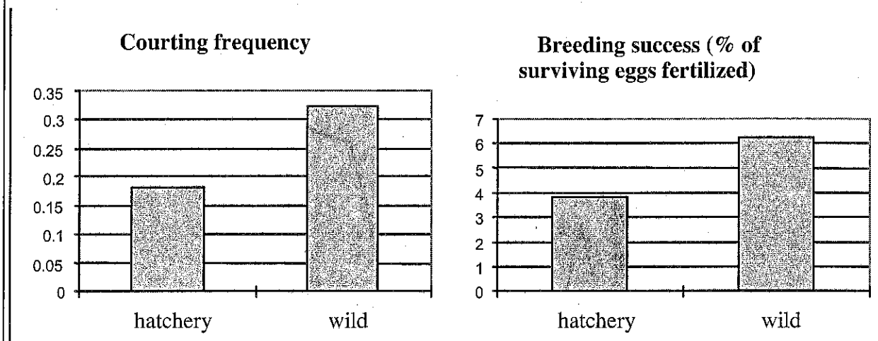
Figure A12-2b. (Data from Fleming and Gross 1993, Table 6.)
