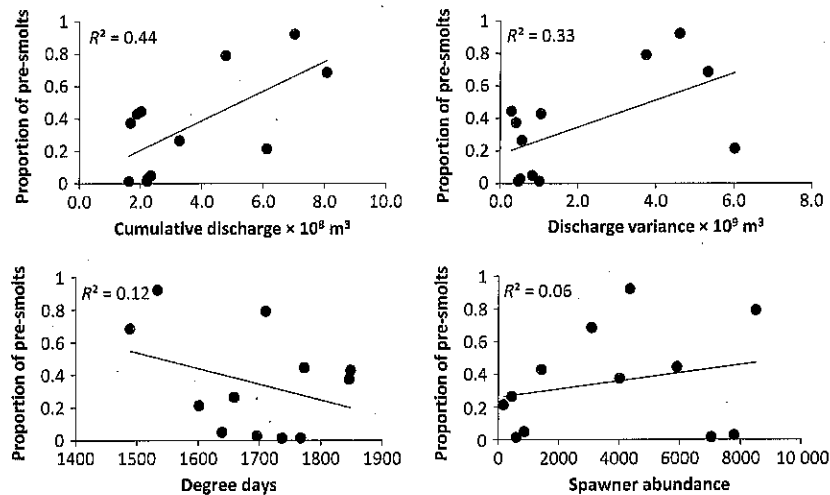
Figure 4. Relationships between the proportion of pre-smolt Chinook salmon migrants and four predictor variables.
