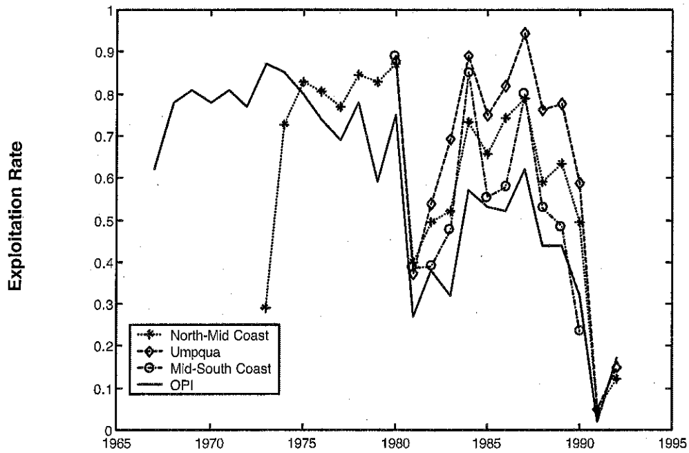
Figure A6. Estimates of exploitation rates for three GCGs (North-Mid Coast, Umpqua, Mid-South Coast) of Oregon coastal coho salmon ( Oncorhynchus kisutch ) and estimated total exploitation rate for coho salmon in the Oregon Production Index Area based on analyses of coded wire tag recoveries. Note the sharp decline in exploitation rate beginning in the late 1980's and extending through the early 1990's.
