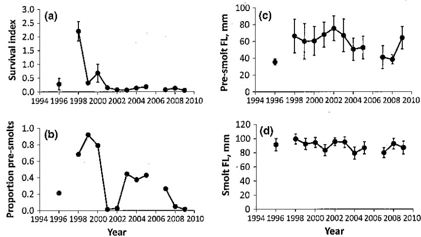
Figure 2. Demographic metrics (mean \pm SD) of the Stanislaus River juvenile Chinook salmon population during 1996–2009. (a) Survival index. (b) Proportion of migrants classified as pre-smolts. (c) Mean fork length (FL) of pre-smolt migrants. (d) Mean FL of smolt migrants.
