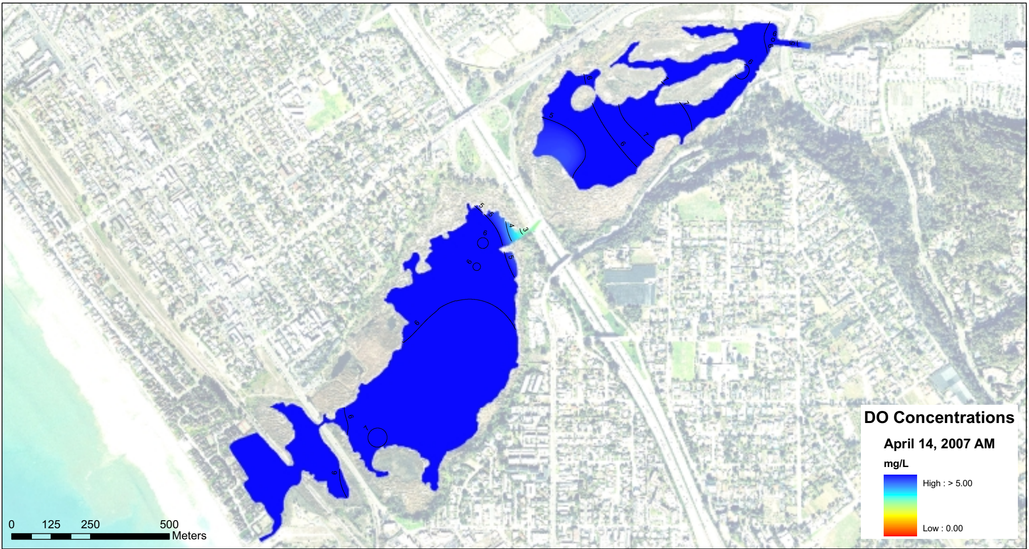
Buena Vista Lagoon Wastewater Spill Dissolved Oxygen Concentrations (mg/L) April 14, 2007 (AM)
