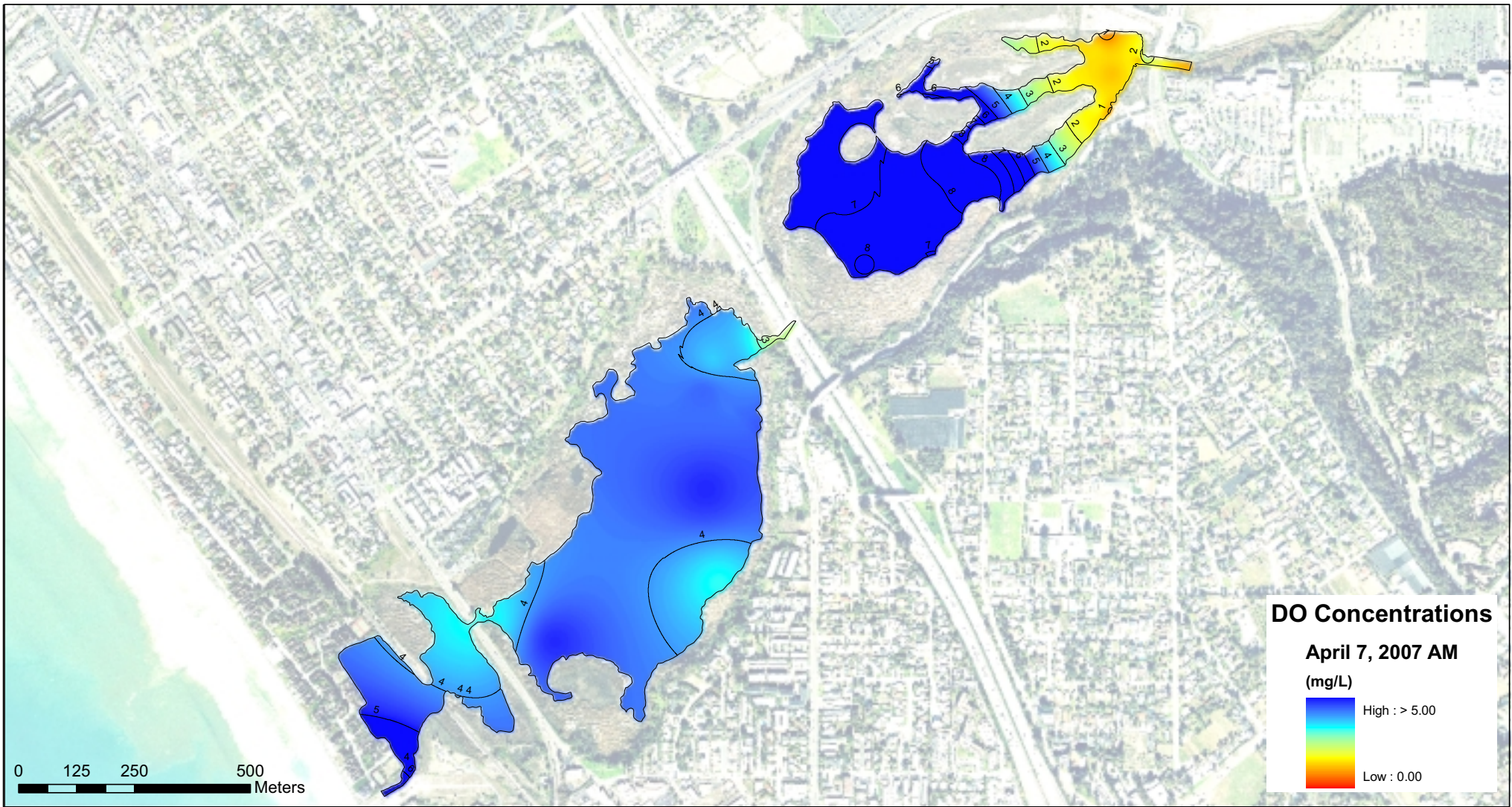
Buena Vista Lagoon Wastewater Spill Dissolved Oxygen Concentrations (mg/L) April 07, 2007 (AM)
