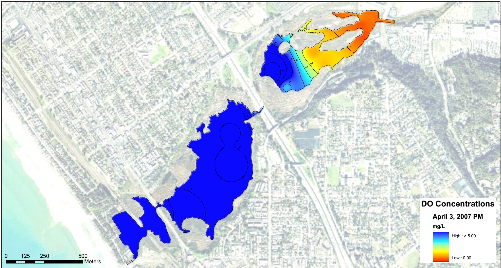
Buena Vista Lagoon Wastewater Spill Dissolved Oxygen Concentrations (mg/L) April 03, 2007 (PM)
