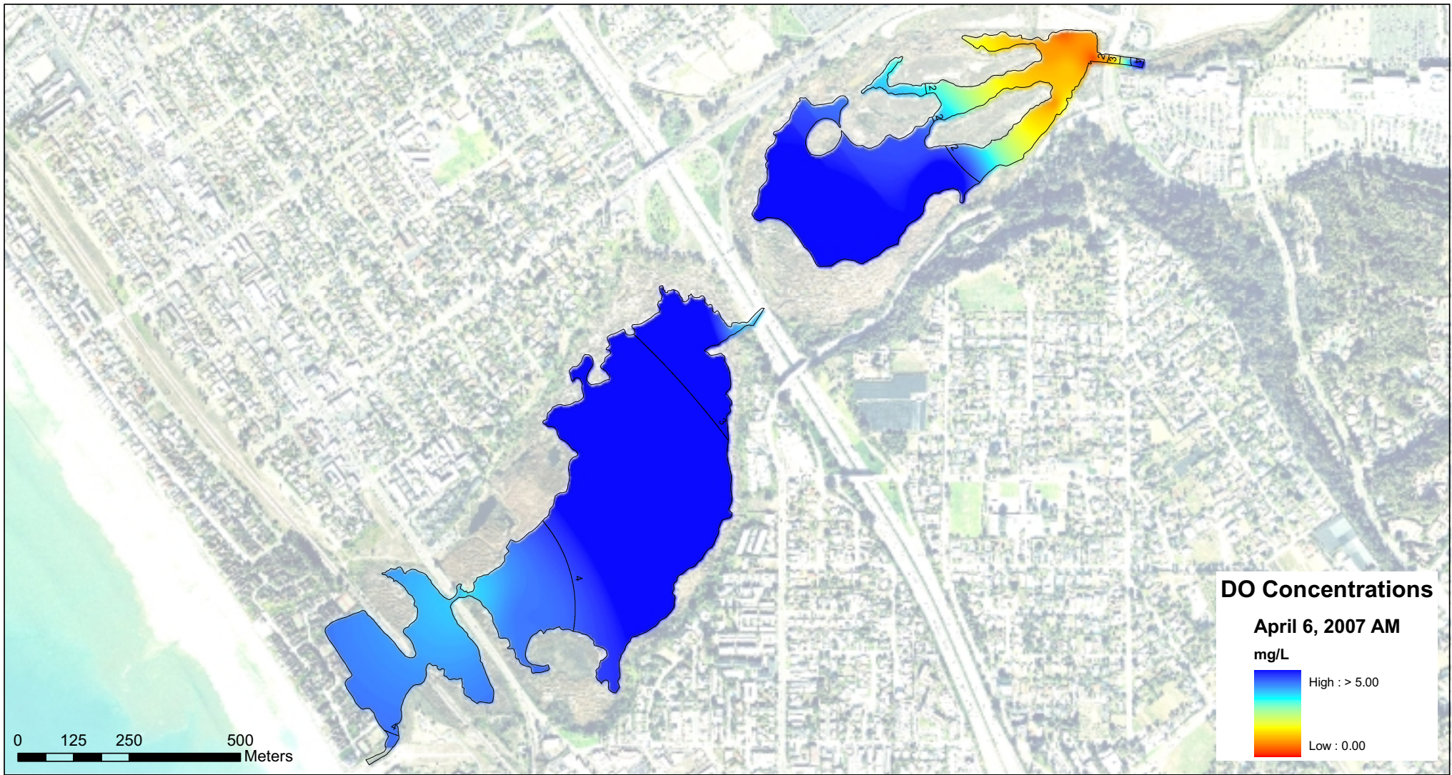
Buena Vista Lagoon Wastewater Spill Dissolved Oxygen Concentrations (mg/L) April 06, 2007 (AM)
