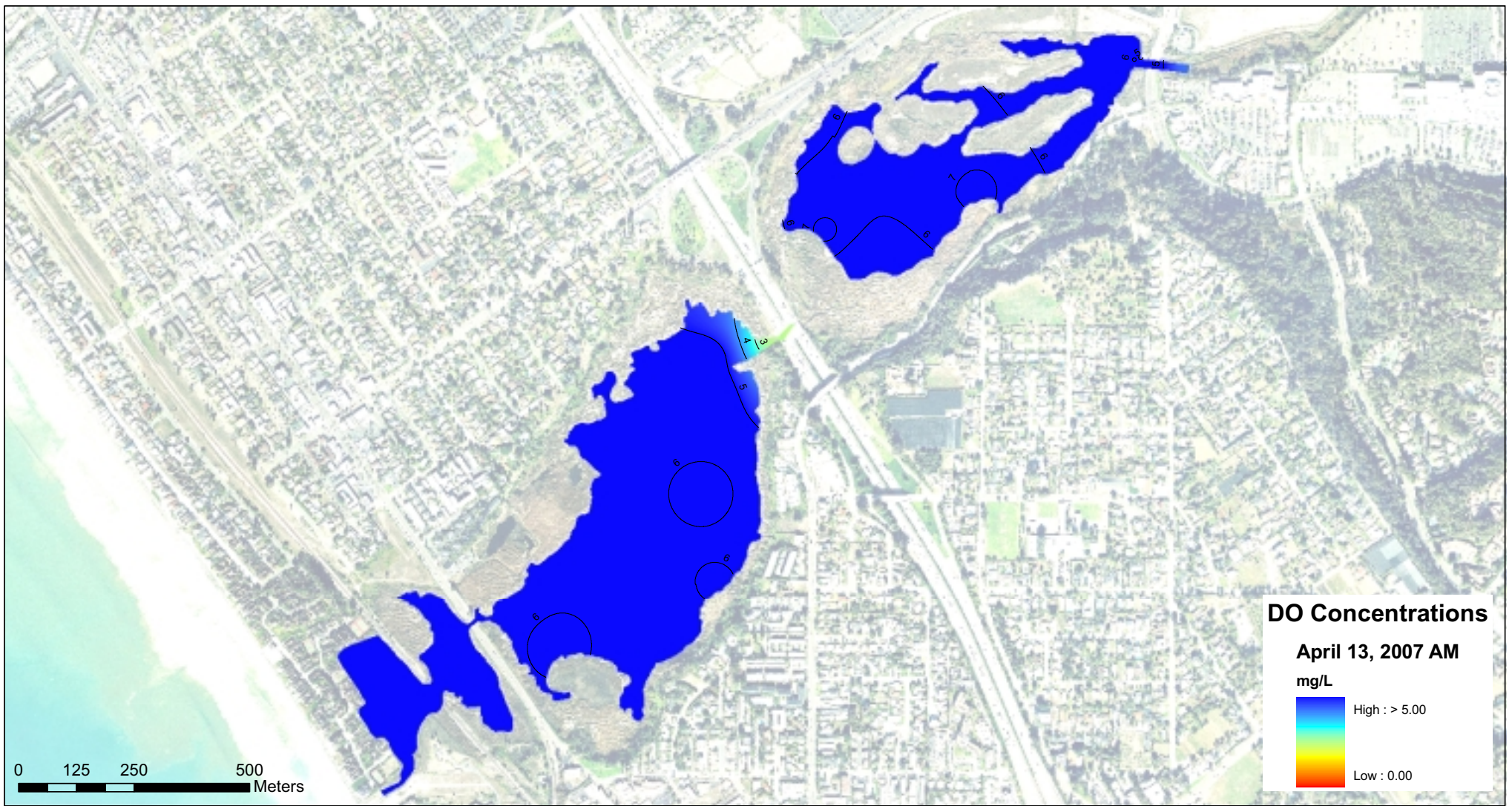
Buena Vista Lagoon Wastewater Spill Dissolved Oxygen Concentrations (mg/L) April 13, 2007 (AM)
