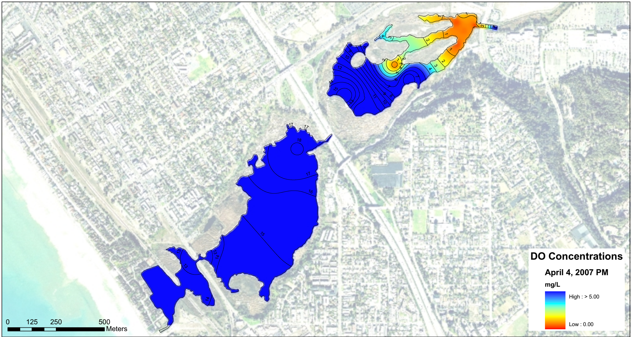
Buena Vista Lagoon Wastewater Spill Dissolved Oxygen Concentrations (mg/L) April 04, 2007 (PM)
