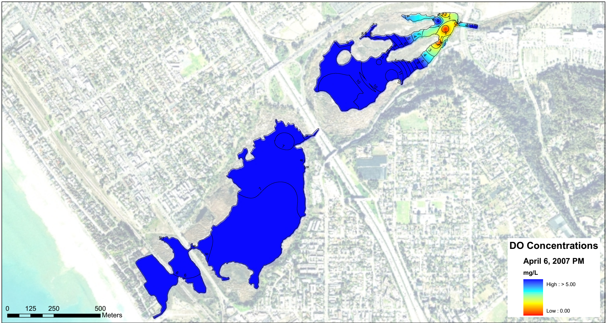
Buena Vista Lagoon Wastewater Spill Dissolved Oxygen Concentrations (mg/L) April 06, 2007 (PM)
