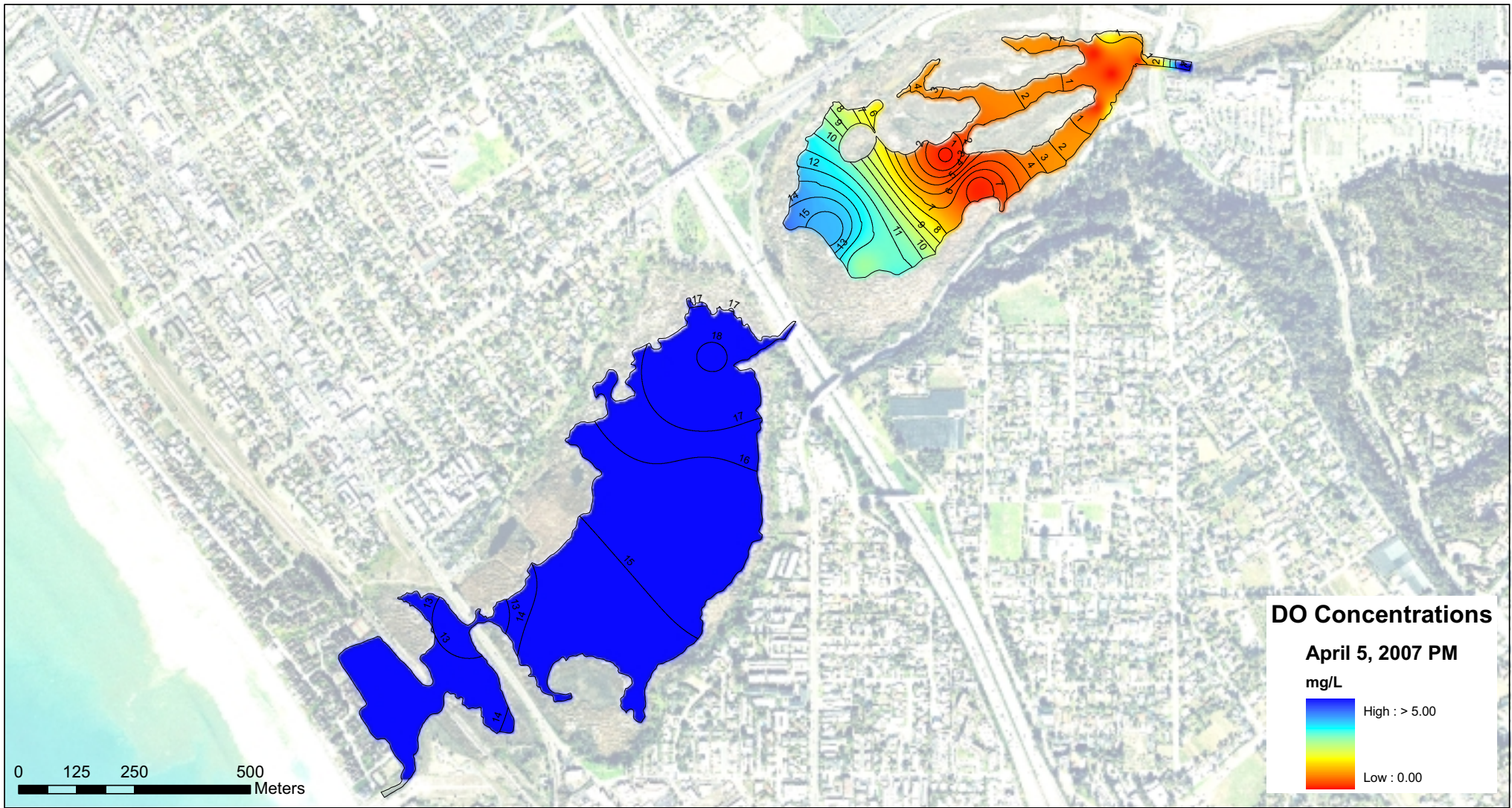
Buena Vista Lagoon Wastewater Spill Dissolved Oxygen Concentrations (mg/L) April 05, 2007 (PM)
