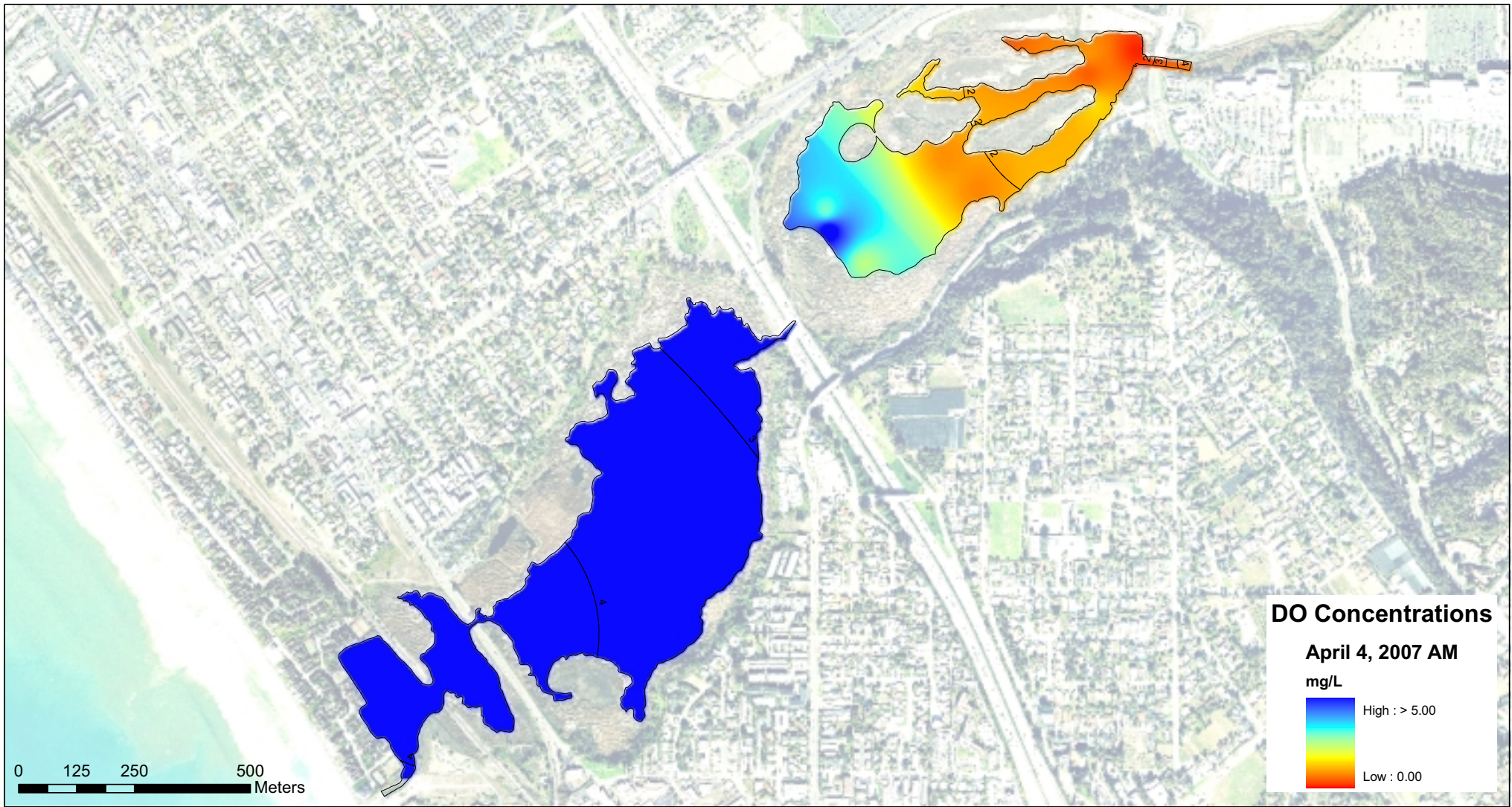
Buena Vista Lagoon Wastewater Spill Dissolved Oxygen Concentrations (mg/L) April 04, 2007 (AM)
