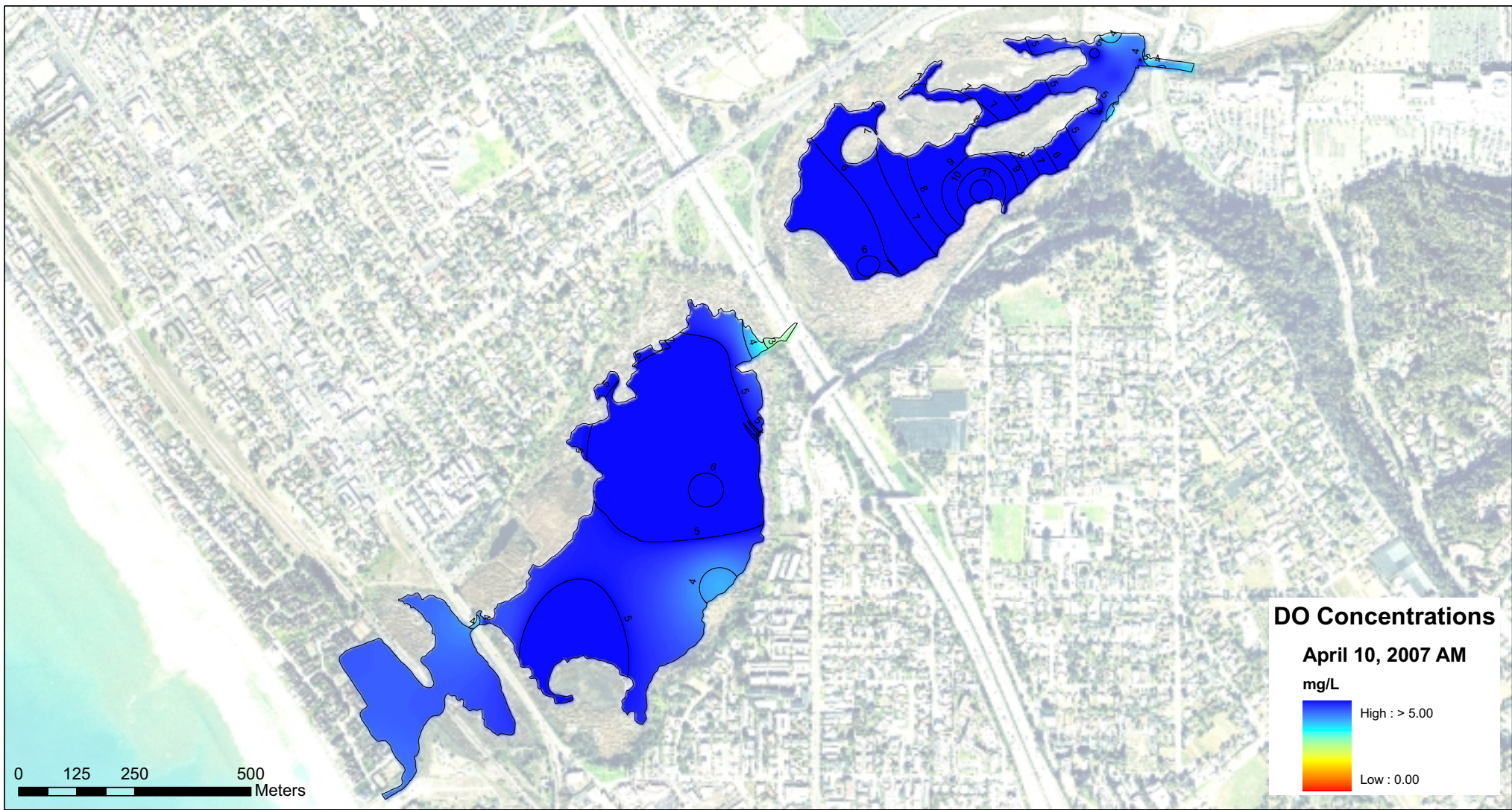
Buena Vista Lagoon Wastewater Spill Dissolved Oxygen Concentrations (mg/L) April 10, 2007 (AM)
