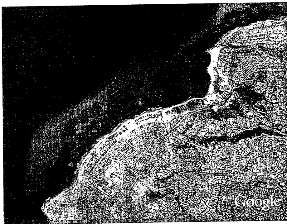
Figure 6. Example of the four sampling depth strata on a natural reef.
