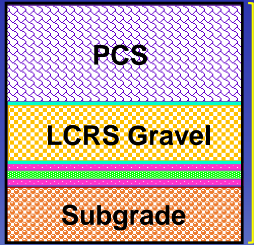
Sycamore's Engineered Alternative Liner System
