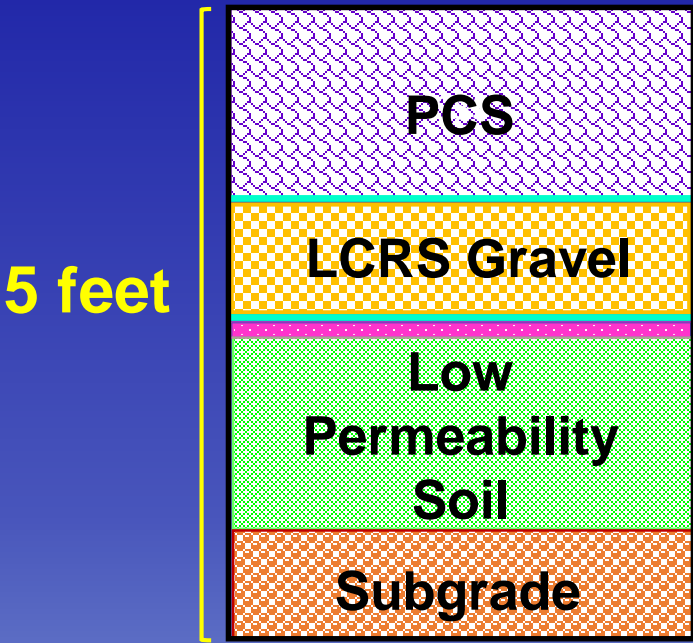
Prescriptive Liner System
