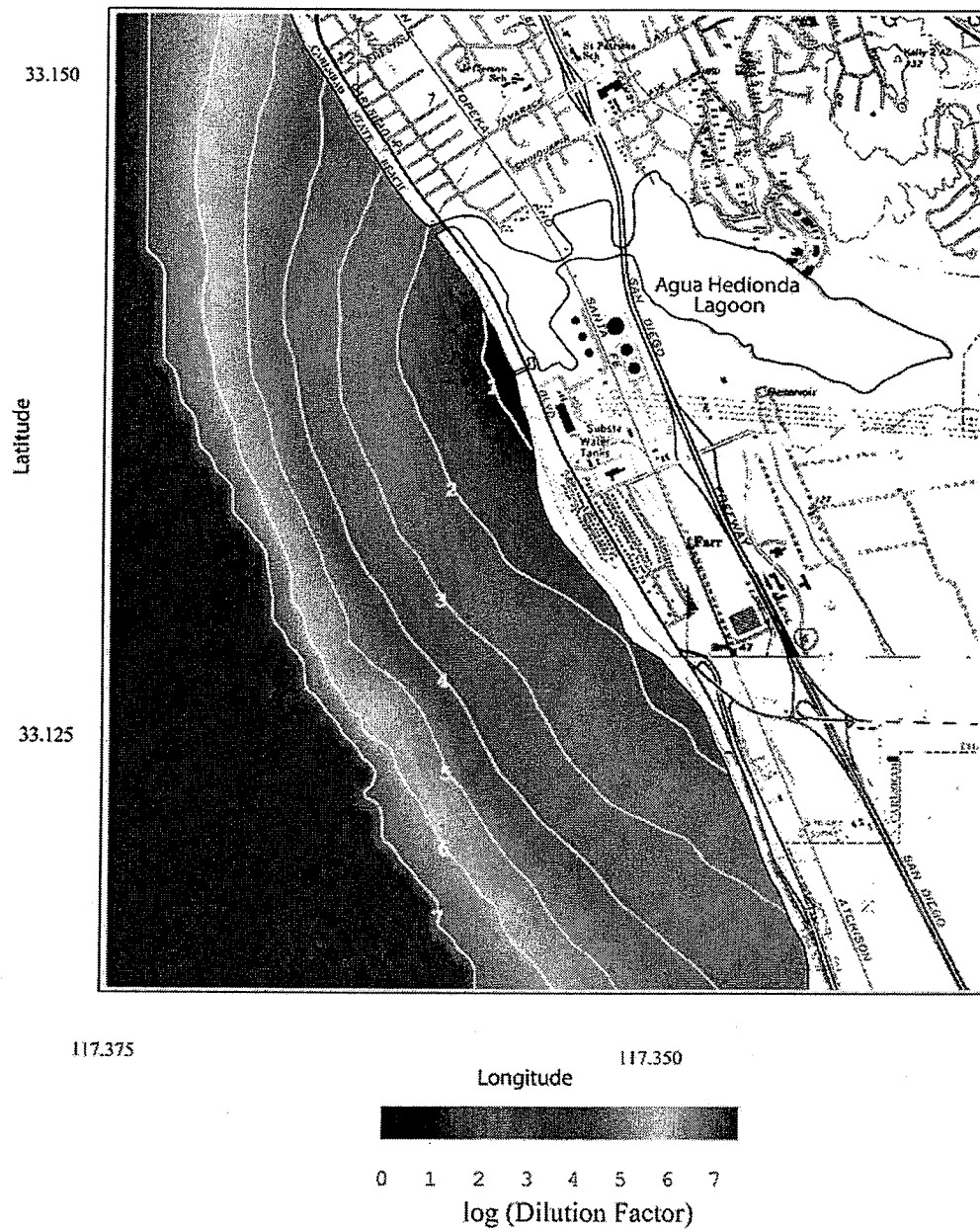
Figure 16. Scenario 3 worst case with one Unit 5 circulation pump, and one Unit 1 pump for \Delta T = 0^{\circ}\text{C} . Depth-averaged dilution factor for raw concentrate from desalination. R.O. = 50 mgd, plant inflow rate = 184.32 mgd, combined discharge = 134.32 mgd, ambient ocean salinity = 33.51 ppt, ocean conditions - 17 Aug 1992.
