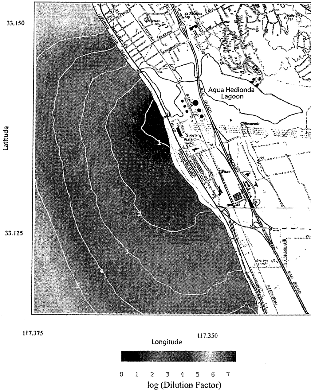
Figure 30. Scenario 2 average case with all circulation pumps - Units 1&2, and one pump - Unit 3 for \Delta T = 0^{\circ}\text{C} . Seafloor dilution factor for raw concentrate from desalination. R.O. = 50 mgd, plant inflow rate = 172.8 mgd, combined discharge = 122.8 mgd, ambient ocean salinity = 33.52 ppt, ocean conditions - 23 May 1994.
