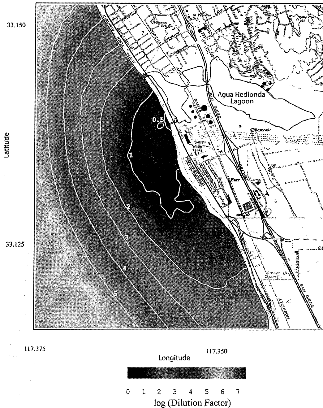
Figure 14. Scenario 3 worst case with one Unit 5 circulation pump, and one Unit 1 pump for \Delta T = 0^{\circ}\text{C} . Seafloor dilution factor for raw concentrate from desalination. R.O. = 50 mgd, plant inflow rate = 184.32 mgd, combined discharge = 134.32 mgd, ambient ocean salinity = 33.51 ppt, ocean conditions - 17 Aug 1992.
