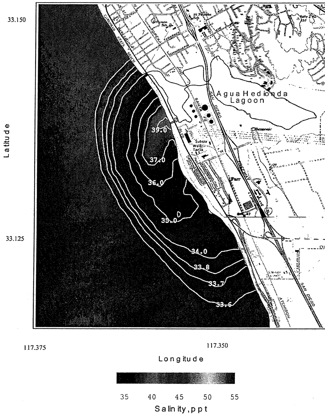
Figure 21. Scenario 5 worst case with two Unit 4 circulation 2 pumps for \Delta T = 0^{\circ}\text{C} . Daily average of the bottom salinity of concentrated seawater for R.O. = 50 mgd, plant inflow rate = 304 mgd, combined discharge = 254 mgd, ambient ocean salinity = 33.51 ppt, ocean conditions - 17 Aug 1992.
