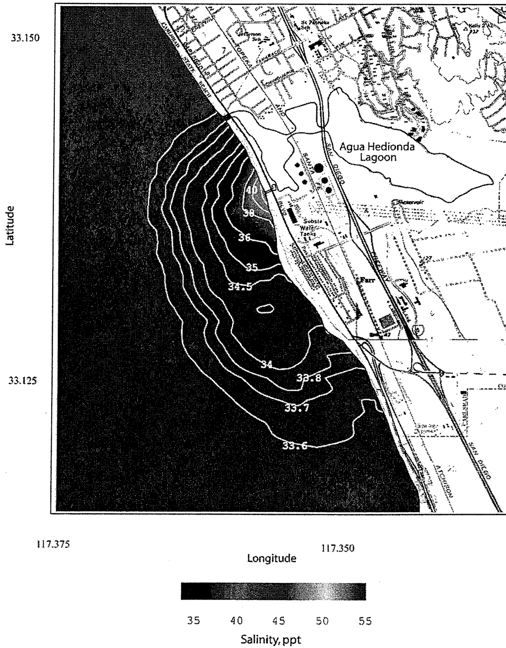
Figure 33. Scenario 3 average case with one Unit 5 circulation pump, and one Unit 1 pump for \Delta T = 0^{\circ}\text{C} . Daily average of the bottom salinity of concentrated seawater for R.O. = 50 mgd, plant inflow rate = 184.32 mgd, combined discharge = 134.32 mgd, ambient ocean salinity = 33.52 ppt, ocean conditions - 23 May 1994.
