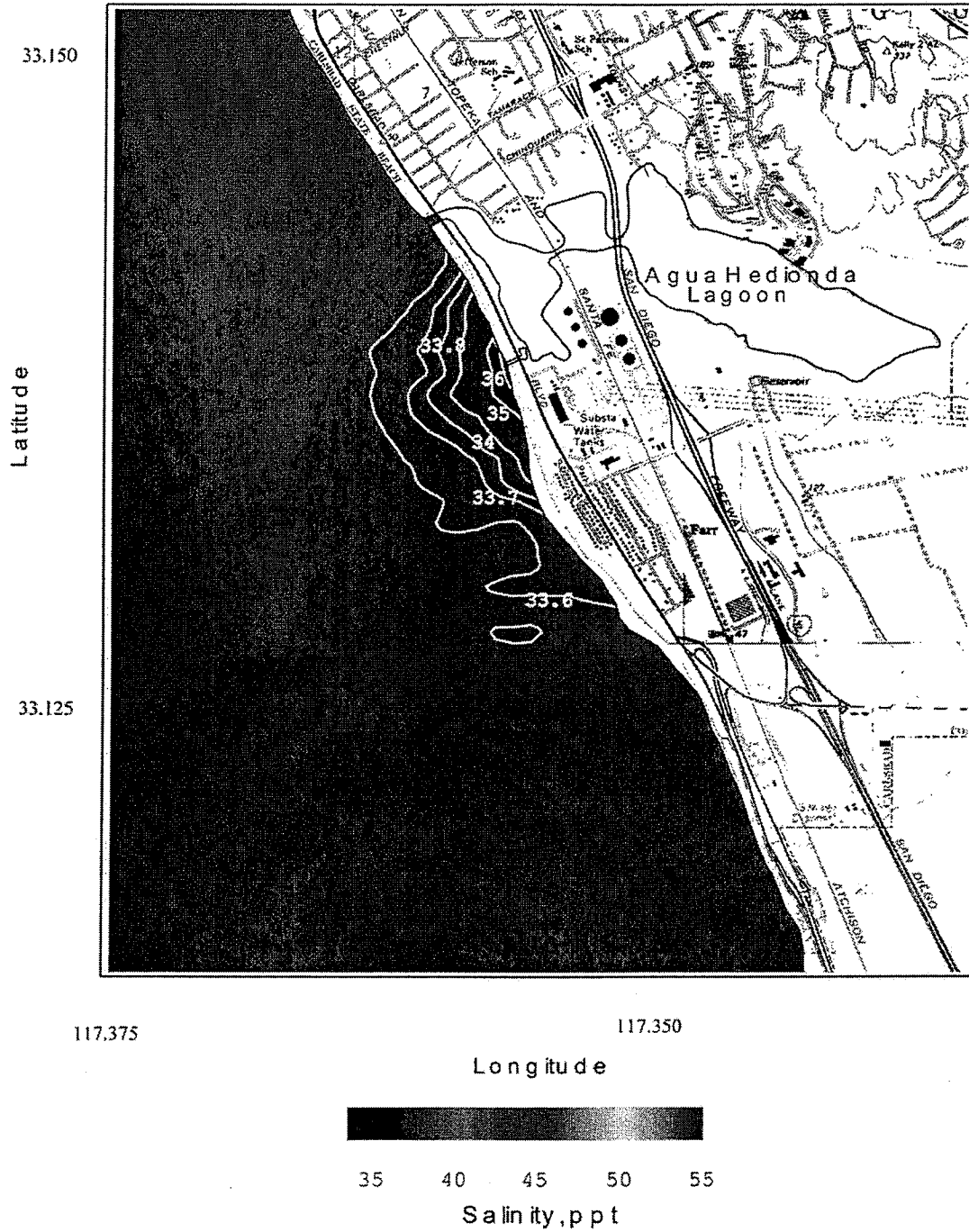
Figure 43. Scenario 5 average case with two Unit 4 circulation pumps for \Delta T = 0^{\circ}\text{C} . Daily depth-averaged salinity of concentrated seawater for R.O. = 50 mgd, plant inflow rate = 304 mgd, combined discharge = 254 mgd, ambient ocean salinity = 33.52 ppt, ocean conditions, 23 May 1994.
