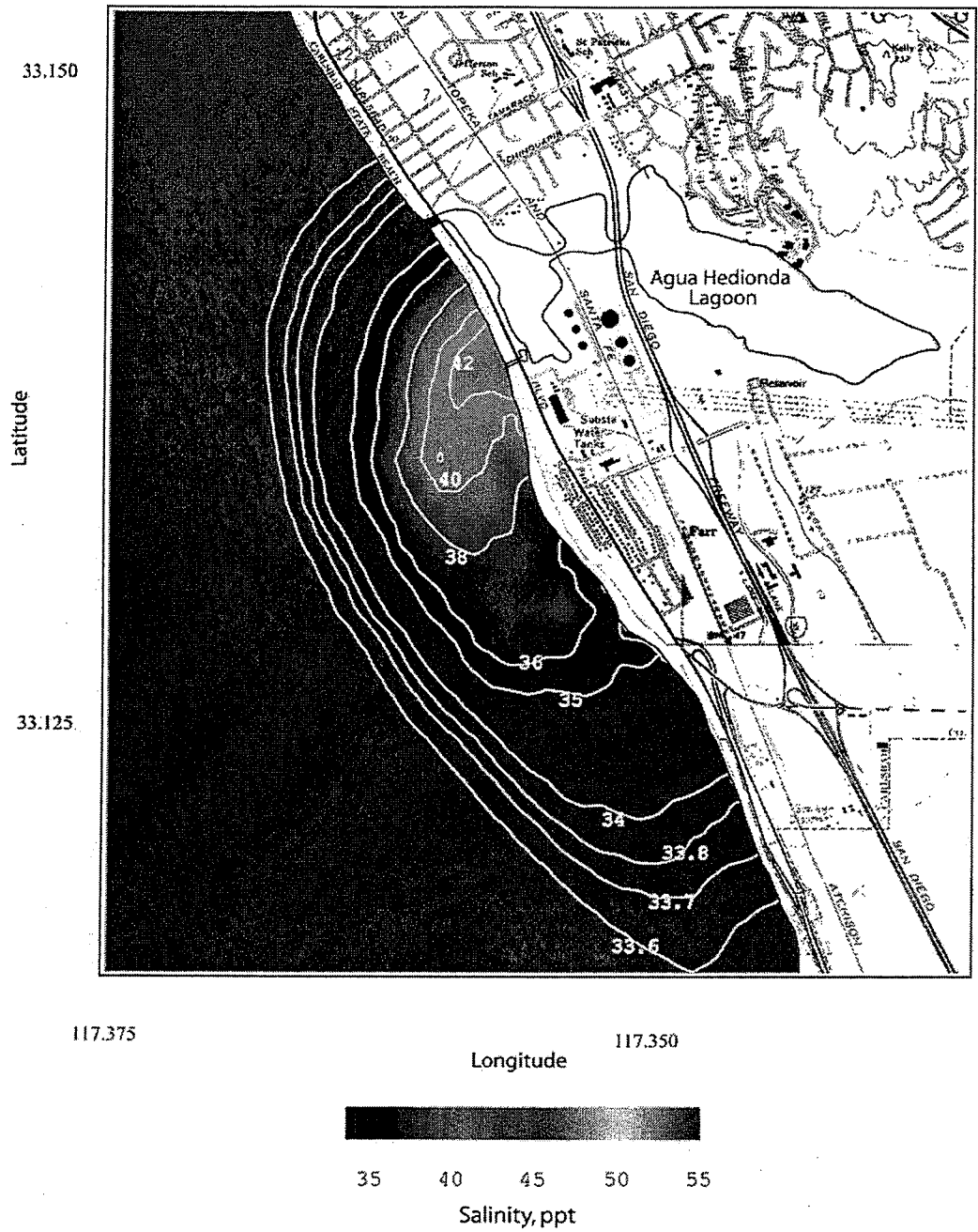
Figure 13. Scenario 3 worst case with one Unit 5 circulation pump, and one Unit 1 pump for \Delta T = 0^\circ\text{C} . Daily average of the bottom salinity of concentrated seawater for R.O. = 50 mgd, plant inflow rate = 184.32 mgd, combined discharge = 134.32 mgd, ambient ocean salinity = 33.51 ppt, ocean conditions - 17 Aug 1992.
