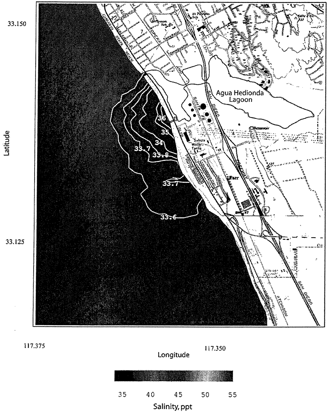
Figure 35. Scenario 3 average case with one Unit 5 circulation pump, and one Unit 1 pump for \Delta T = 0^\circ\text{C} . Daily depth-averaged salinity of concentrated seawater for R.O. = 50 mgd, plant inflow rate = 184.32 mgd, combined discharge = 134.32 mgd, ambient ocean salinity = 33.52 ppt, ocean conditions - 23 May 1994.
