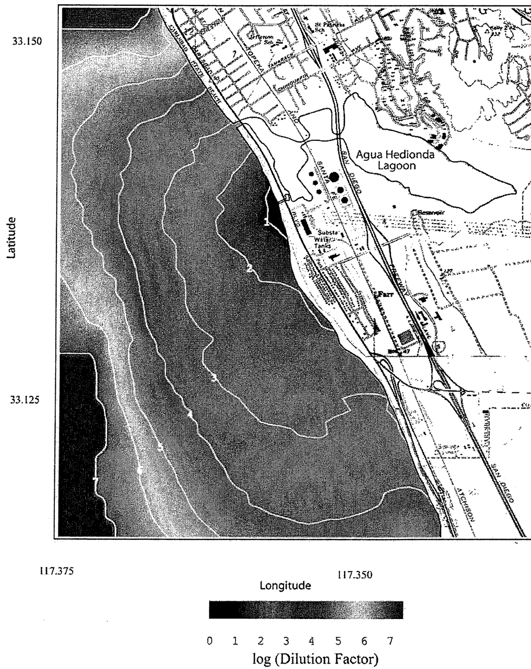
Figure 28. Scenario 1 average case with one Unit 5 circulation pump for \Delta T = 0^\circ\text{C} . Depth-averaged dilution factor for raw concentrate from desalination. R.O. = 50 mgd, plant inflow rate = 149.76 mgd, combined discharge = 99.76 mgd, ambient ocean salinity = 33.52 ppt, ocean conditions - 23 May 1994.
