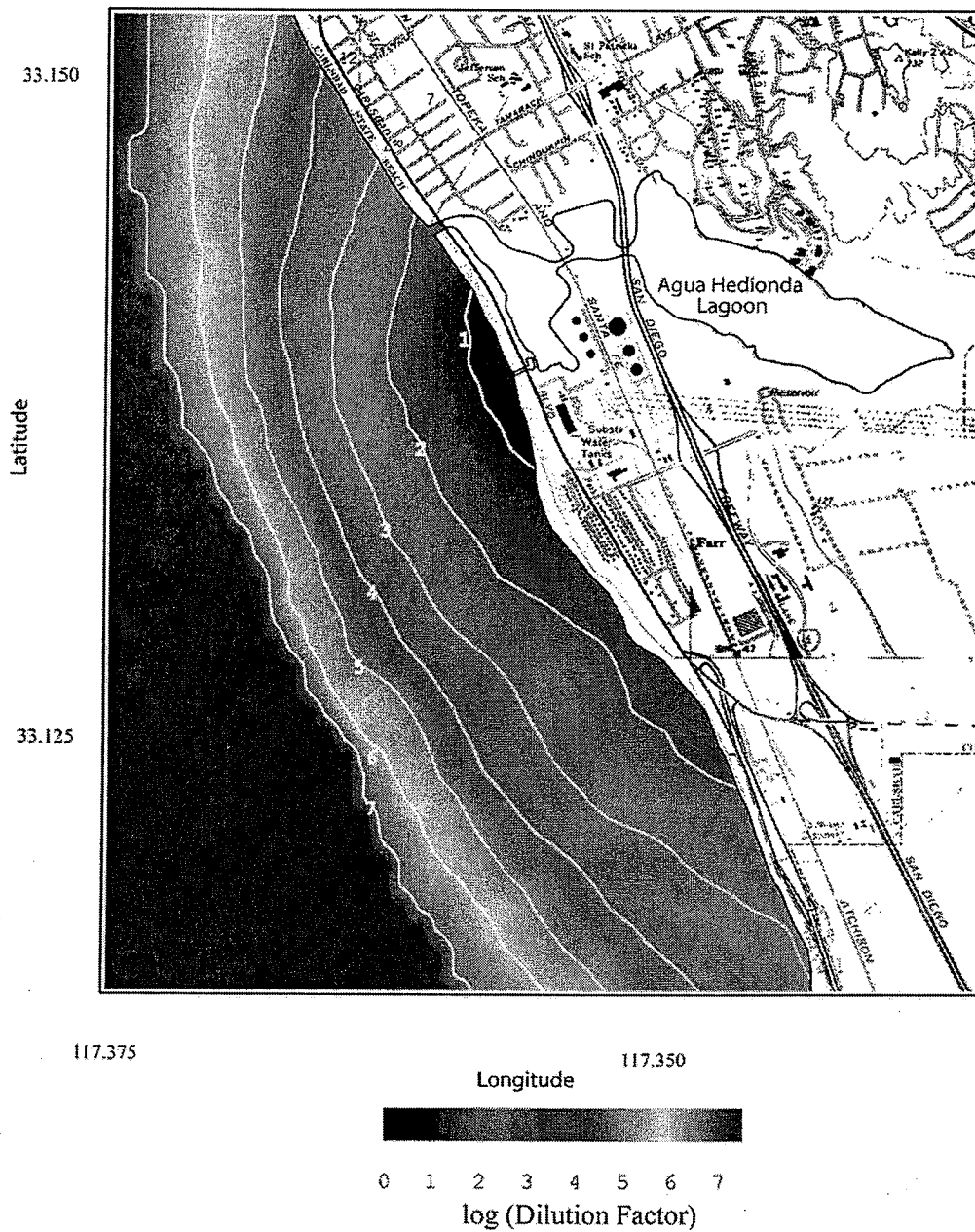
Figure 8. Scenario 1 worst case with one Unit 5 circulation pump for \Delta T = 0 °C. Depth-averaged dilution factor for raw concentrate from desalination. R.O. = 50 mgd, plant inflow rate = 149.76 mgd, combined discharge = 99.76 mgd, ambient ocean salinity = 33.51 ppt, ocean conditions - 17 Aug 1992.
