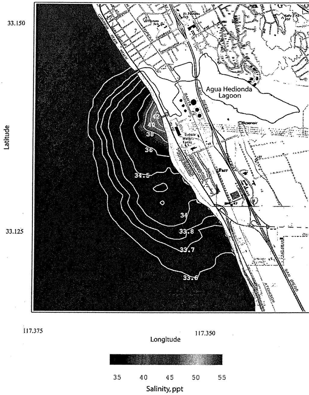
Figure 29. Scenario 2 average case with all circulation pumps - Units 1&2, and one pump - Unit 3 for \Delta T = 0^{\circ}\text{C} . Daily average of the bottom salinity of concentrated seawater for R.O. = 50 mgd, plant inflow rate = 172.8 mgd, combined discharge = 122.8 mgd, ambient ocean salinity = 33.52 ppt, ocean conditions - 23 May 1994.
