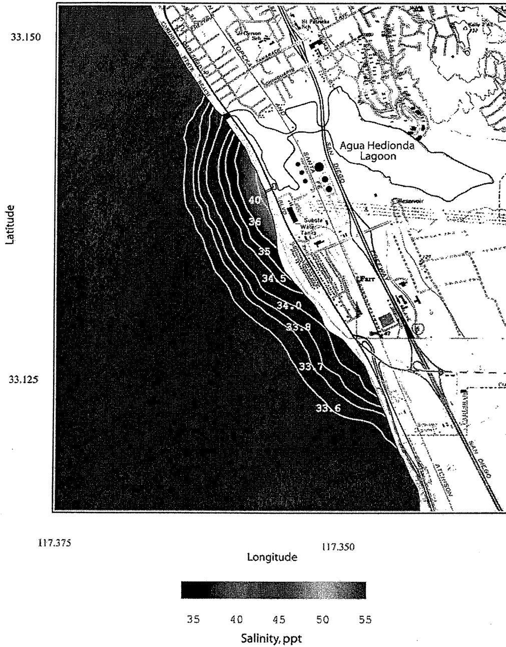
Figure 7. Scenario 1 worst case with one Unit 5 circulation pump for \Delta T = 0 °C. Daily depth-averaged salinity of concentrated seawater for R.O. = 50 mgd, plant inflow rate = 149.76 mgd, combined discharge = 99.76 mgd, ambient ocean salinity = 33.51 ppt, ocean conditions - 17 Aug 1992.
