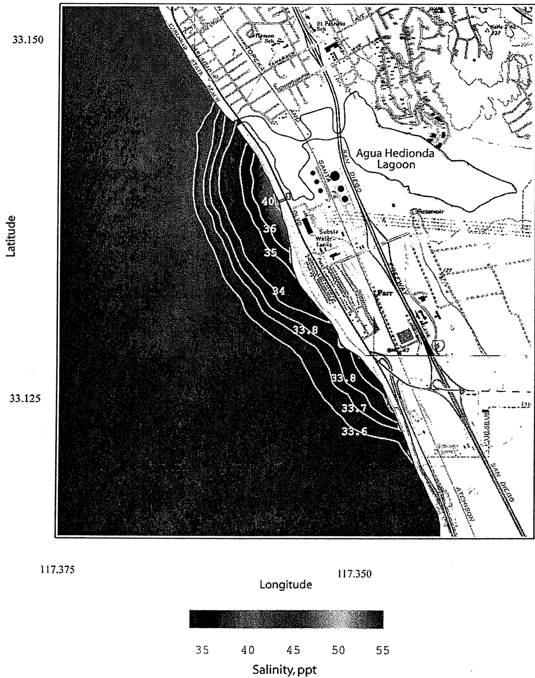
Figure 15. Scenario 3 worst case with one Unit 5 circulation pump, and one Unit 1 pump for \Delta T = 0^\circ\text{C} . Daily depth-averaged salinity of concentrated seawater for R.O. = 50 mgd, plant inflow rate = 184.32 mgd, combined discharge = 134.32 mgd, ambient ocean salinity = 33.51 ppt, ocean conditions - 17 Aug 1992.
