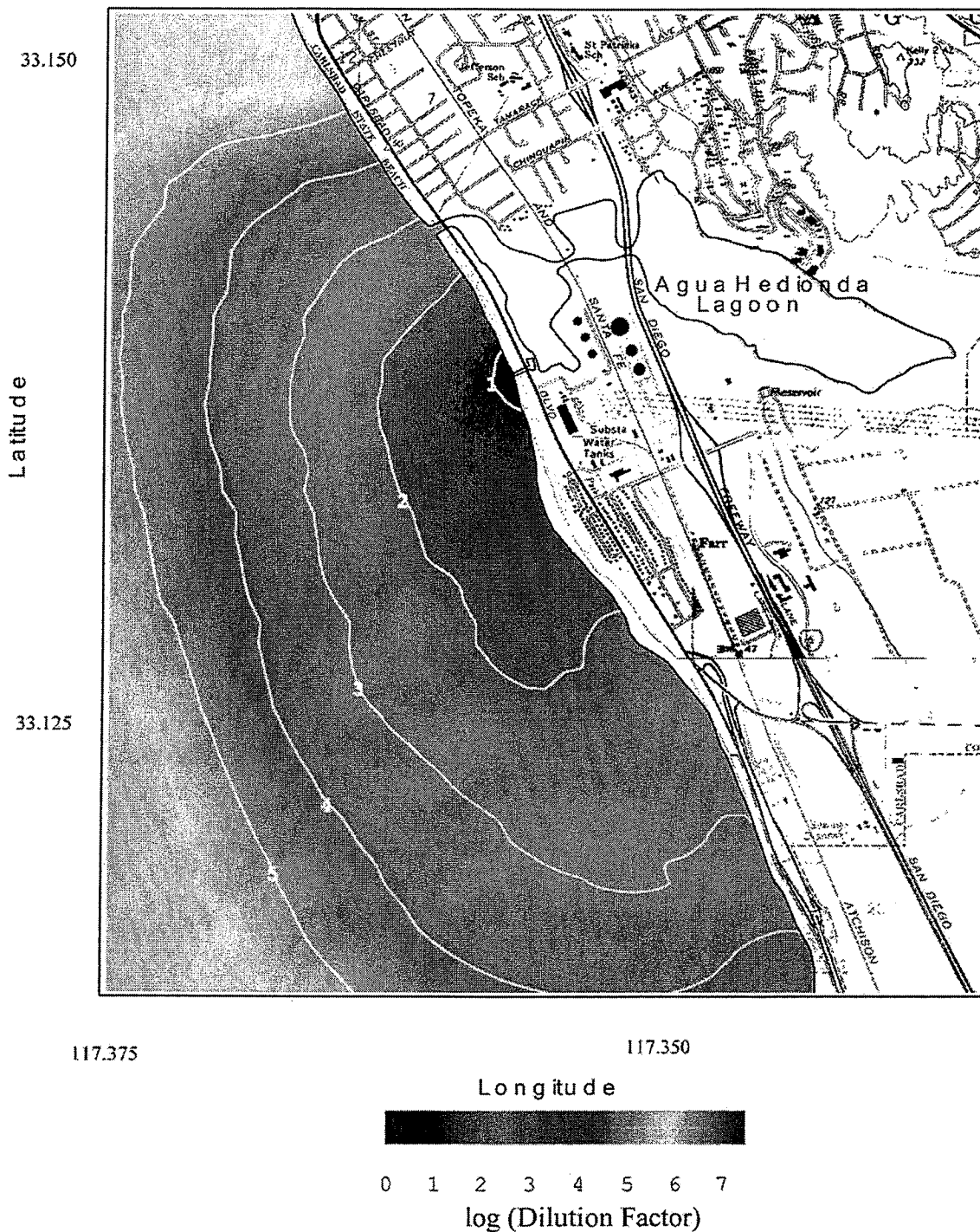
Figure 42. Scenario 5 average case with two Unit 4 circulation pumps for \Delta T = 0^{\circ}\text{C} . Seafloor dilution factor for raw concentrate from desalination. R.O. = 50 mgd, plant inflow rate = 304 mgd, combined discharge = 254 mgd, ambient ocean salinity = 33.52 ppt, ocean conditions, 23 May 1994.
