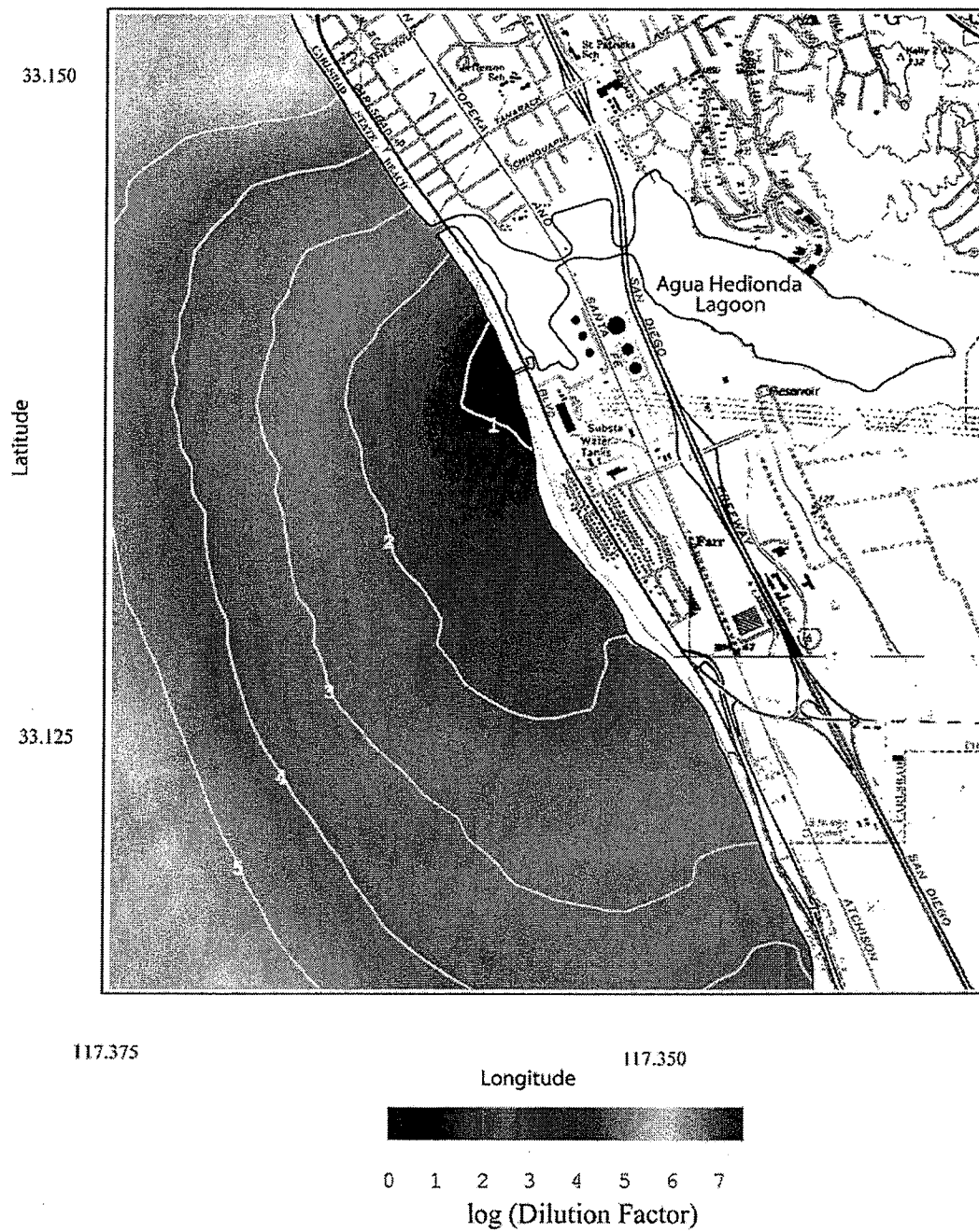
Figure 34. Scenario 3 average case with one Unit 5 circulation pump, and one Unit 1 pump for \Delta T = 0^\circ\text{C} . Seafloor dilution factor for raw concentrate from desalination. R.O. = 50 mgd, plant inflow rate = 184.32 mgd, combined discharge = 134.32 mgd, ambient ocean salinity = 33.52 ppt, ocean conditions - 23 May 1994.
