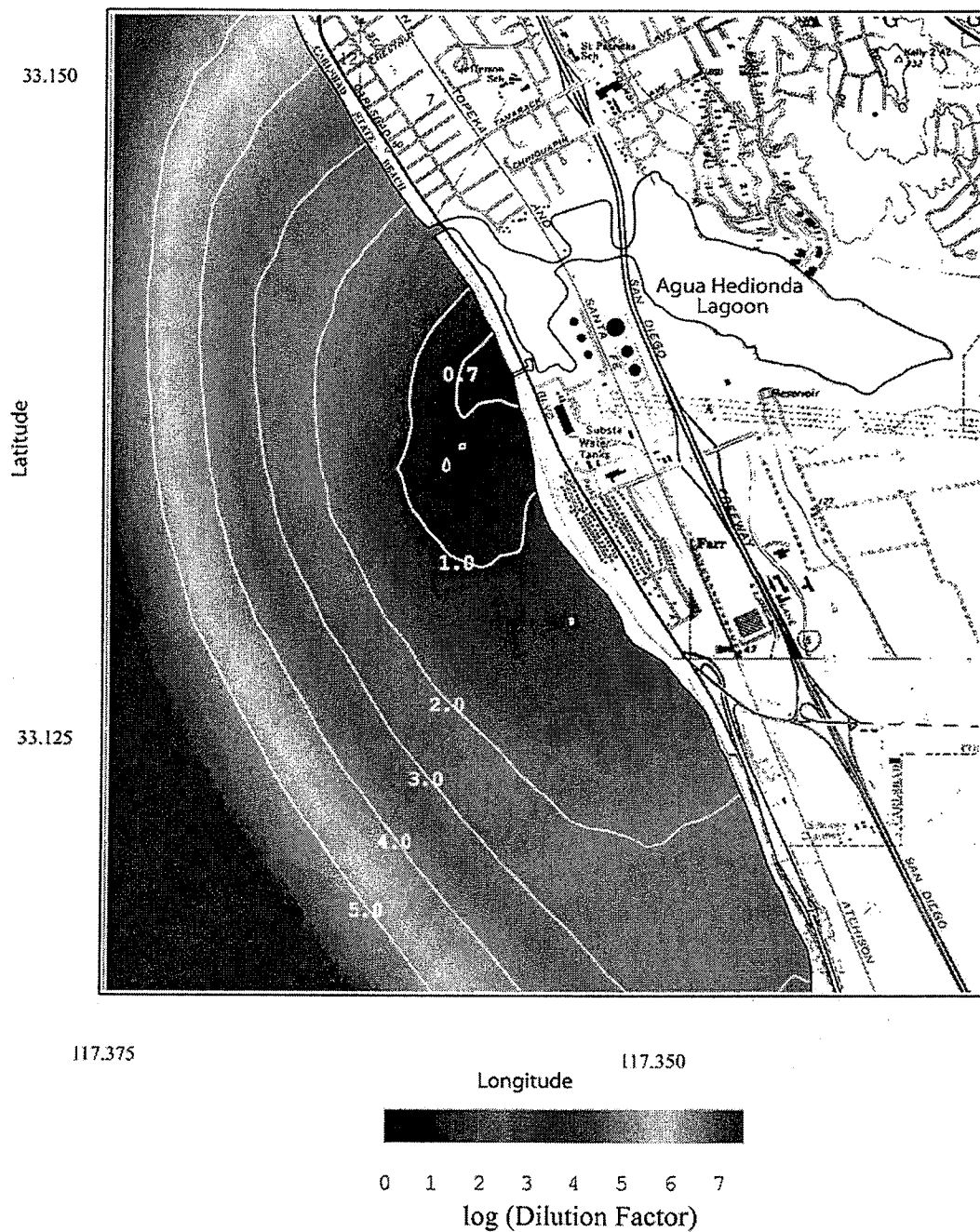
Figure 18. Scenario 4 worst case with one Unit 5 circulation pump, and two Unit 1 pumps for \Delta T = 0^{\circ}\text{C} . Seafloor dilution factor for raw concentrate from desalination. R.O. = 50 mgd, plant inflow rate = 218.88 mgd, combined discharge = 168.88 mgd, ambient ocean salinity = 33.51 ppt, ocean conditions - 17 Aug 1992.
