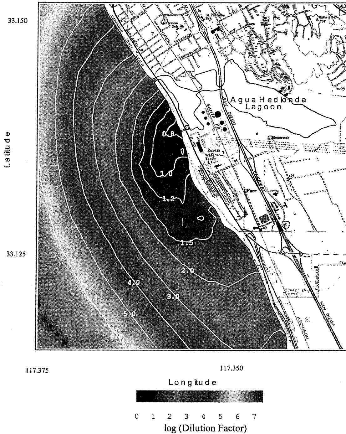
Figure 22. Scenario 5 worst case with two Unit 4 circulation pumps for \Delta T = 0^\circ\text{C} . Seafloor dilution factor for raw concentrate from desalination. R.O. = 50 mgd, plant inflow rate = 304 mgd, combined discharge = 254 mgd, ambient ocean salinity = 33.51 ppt, ocean conditions, 17 Aug 1992.
