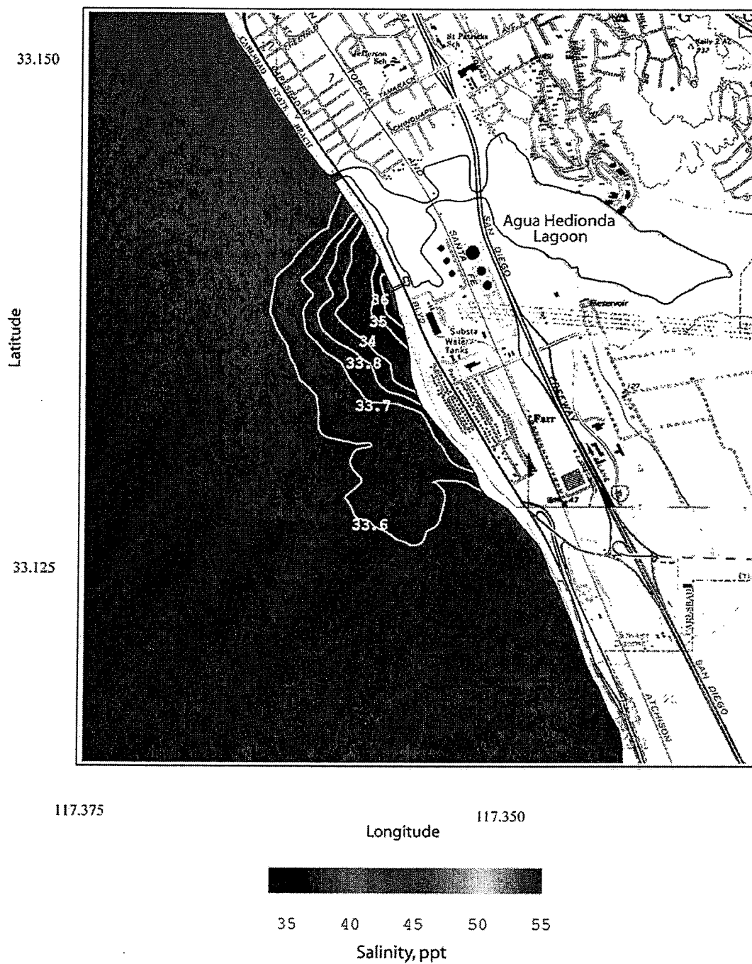
Figure 39. Scenario 4 average case with one Unit 5 circulation pump, and two Unit 1 pumps for \Delta T = 0^\circ\text{C} . Daily depth-averaged salinity of concentrated seawater for R.O. = 50 mgd, plant inflow rate = 218.88 mgd, combined discharge = 168.88 mgd, ambient ocean salinity = 33.52 ppt, ocean conditions - 23 May 1994.
