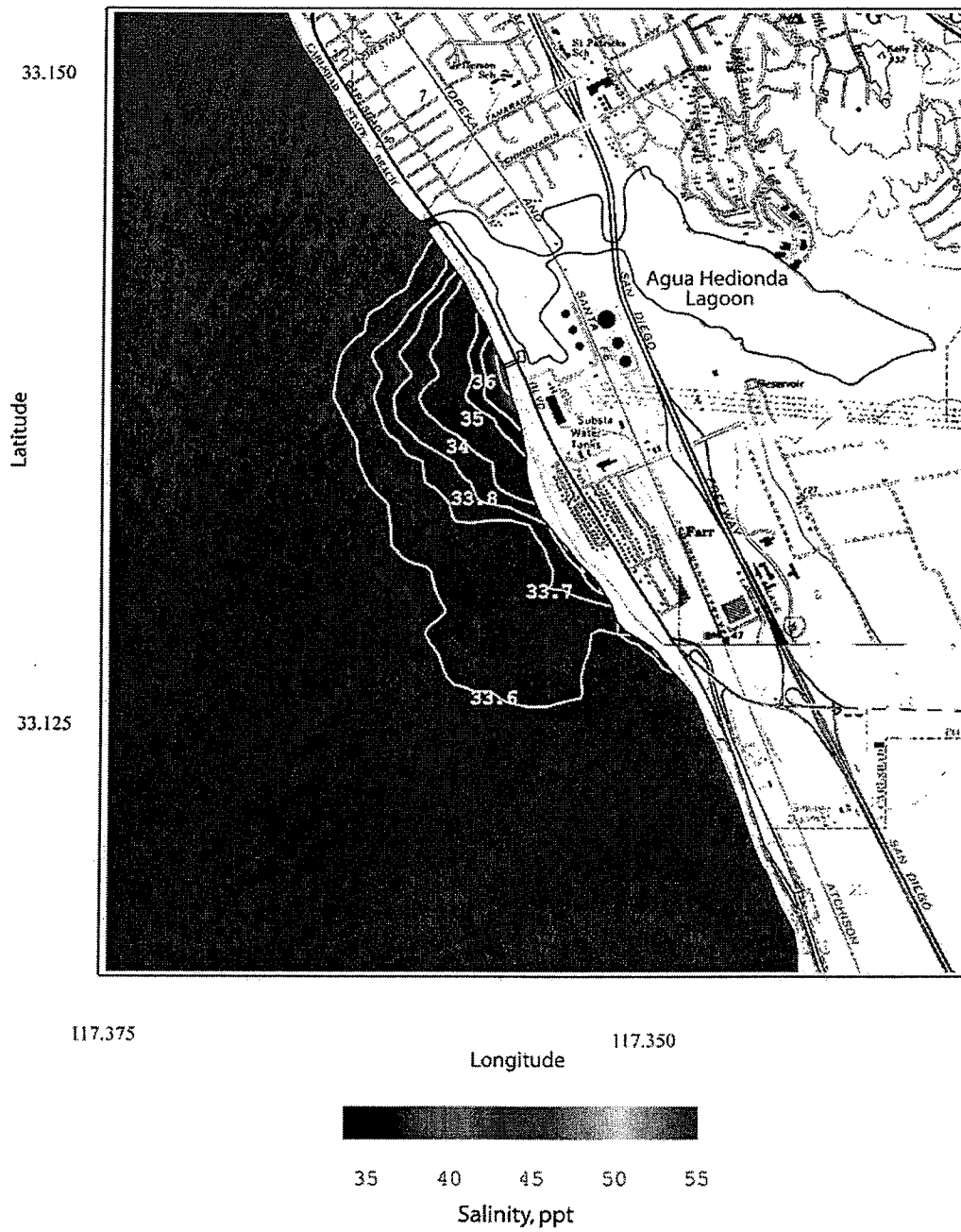
Figure 31. Scenario 2 average case with all circulation pumps - Units 1&2, and one pump - Unit 3 for \Delta T = 0^{\circ}C . Daily depth-averaged salinity of concentrated seawater for R.O. = 50 mgd, plant inflow rate = 172.8 mgd, combined discharge = 122.8 mgd, ambient ocean salinity = 33.52 ppt, ocean conditions - 23 May 1994.
