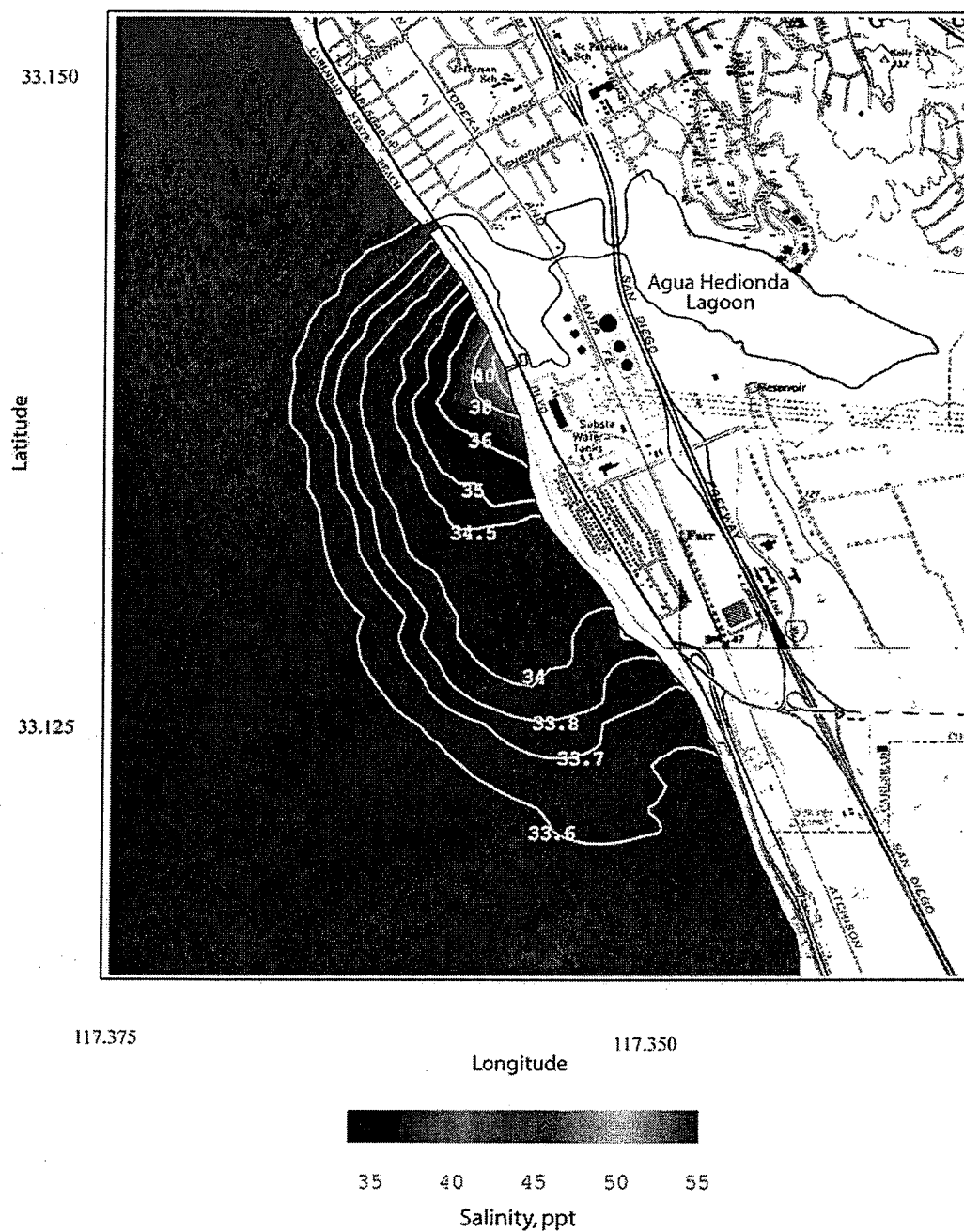
Figure 37. Scenario 4 average case with one Unit 5 circulation pump, and two Unit 1 pumps for \Delta T = 0^\circ\text{C} . Daily average of the bottom salinity of concentrated seawater for R.O. = 50 mgd, plant inflow rate = 218.88 mgd, combined discharge = 168.88 mgd, ambient ocean salinity = 33.52 ppt, ocean conditions - 23 May 1994.
