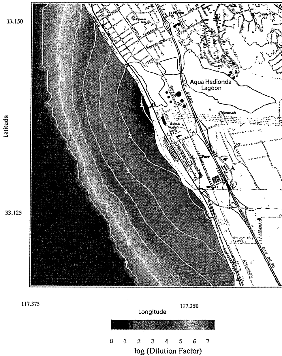
Figure 20. Scenario 4 worst case with one Unit 5 circulation pump, and two Unit 1 pumps for \Delta T = 0^\circ\text{C} . Depth-averaged dilution factor for raw concentrate from desalination. R.O. = 50 mgd, plant inflow rate = 218.88 mgd, combined discharge = 168.88 mgd, ambient ocean salinity = 33.51 ppt, ocean conditions - 17 Aug 1992.
