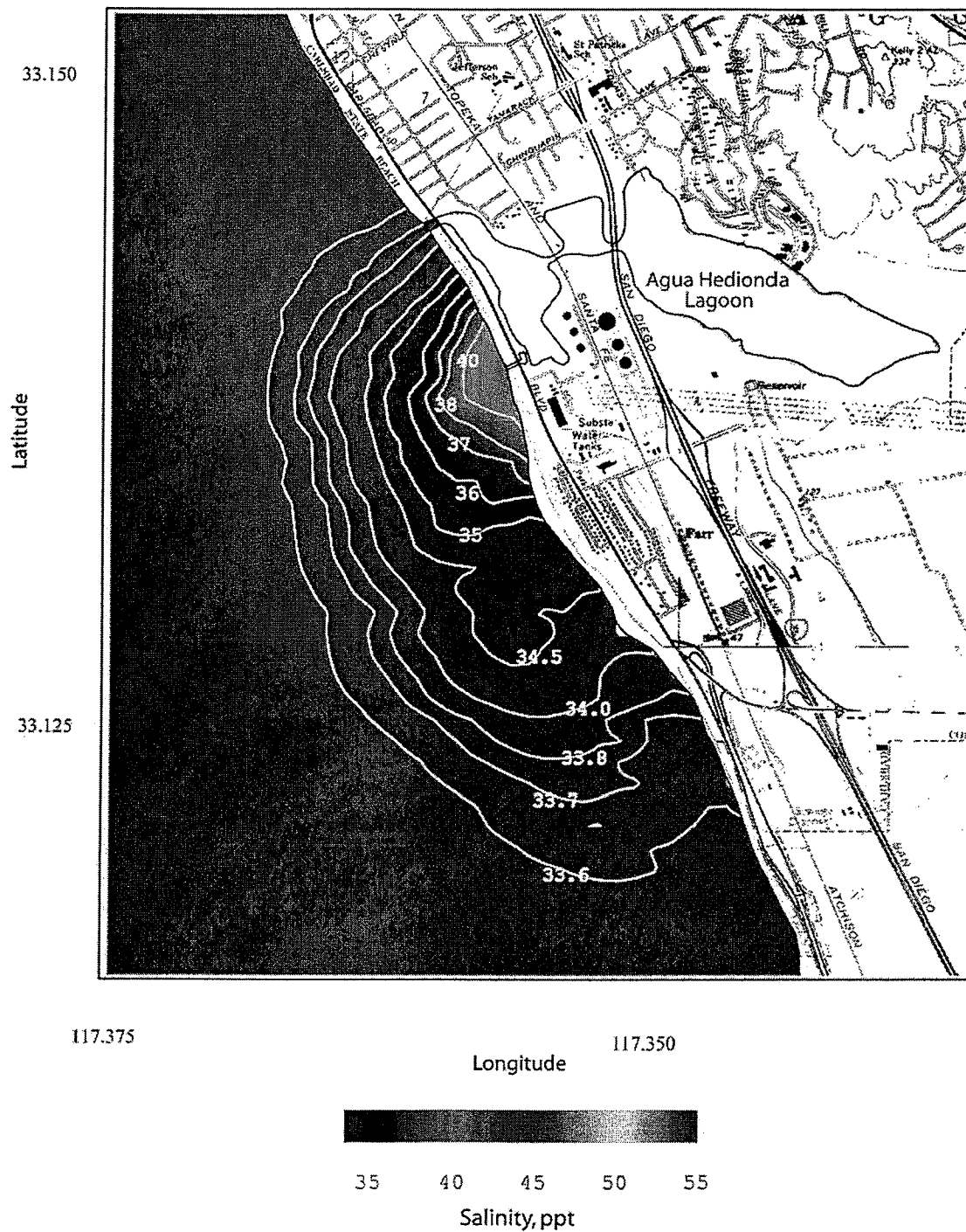
Figure 25. Scenario 1 average case with 1 Unit 5 circulation pump, for \Delta T = 0^{\circ}\text{C} . Daily average of the bottom salinity of concentrated seawater for R.O. = 50 mgd, plant inflow rate = 149.76 mgd, combined discharge = 99.76 mgd, ambient ocean salinity = 33.52 ppt, ocean conditions - 23 May 1994.
