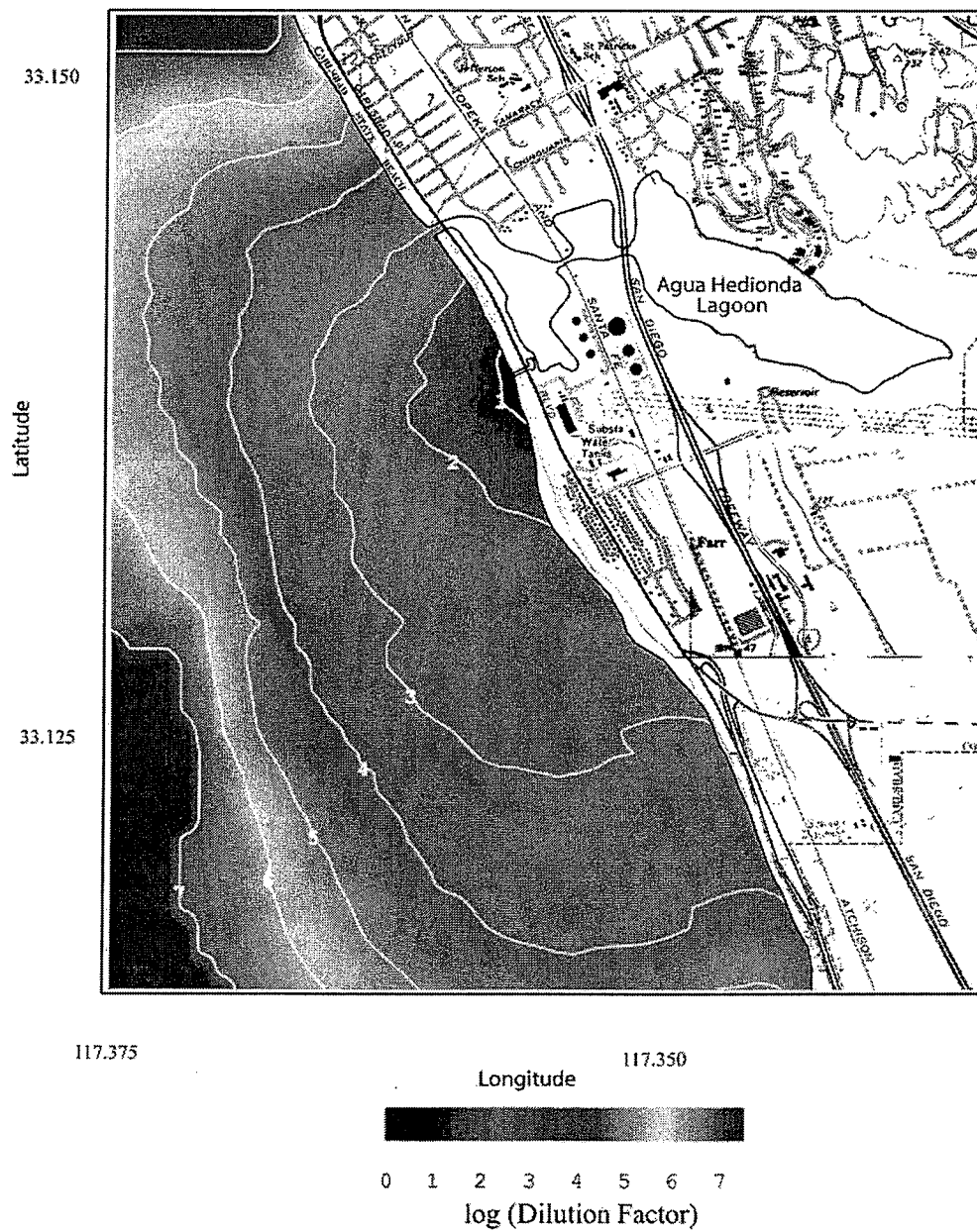
Figure 32. Scenario 2 average case with all circulation pumps - Units 1&2, and one pump - Unit 3 for \Delta T = 0^\circ\text{C} . Depth-averaged dilution factor for raw concentrate from desalination. R.O. = 50 mgd, plant inflow rate = 172.8 mgd, combined discharge = 122.8 mgd, ambient ocean salinity = 33.52 ppt, ocean conditions - 23 May 1994.
