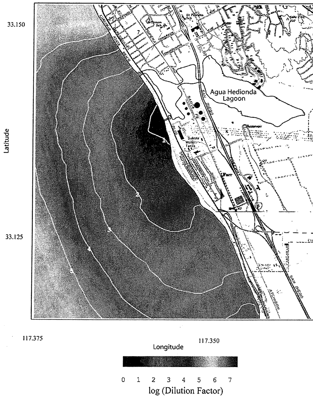
Figure 38. Scenario 4 average case with one Unit 5 circulation pump, and two Unit 1 pumps for \Delta T = 0^\circ\text{C} . Seafloor dilution factor for raw concentrate from desalination. R.O. = 50 mgd, plant inflow rate = 218.88 mgd, combined discharge = 168.88 mgd, ambient ocean salinity = 33.52 ppt, ocean conditions - 23 May 1994.
