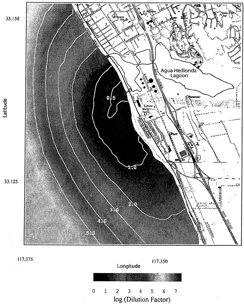
Figure 6. Scenario 1 worst case with one Unit 5 circulation pump for \Delta T = 0^\circ\text{C} . Sea floor dilution factor for raw concentrate from desalination. R.O. = 50 mgd, plant inflow rate = 149.76 mgd, combined discharge = 99.76 mgd, ambient ocean salinity = 33.51 ppt, ocean conditions - 17 Aug 1992.
