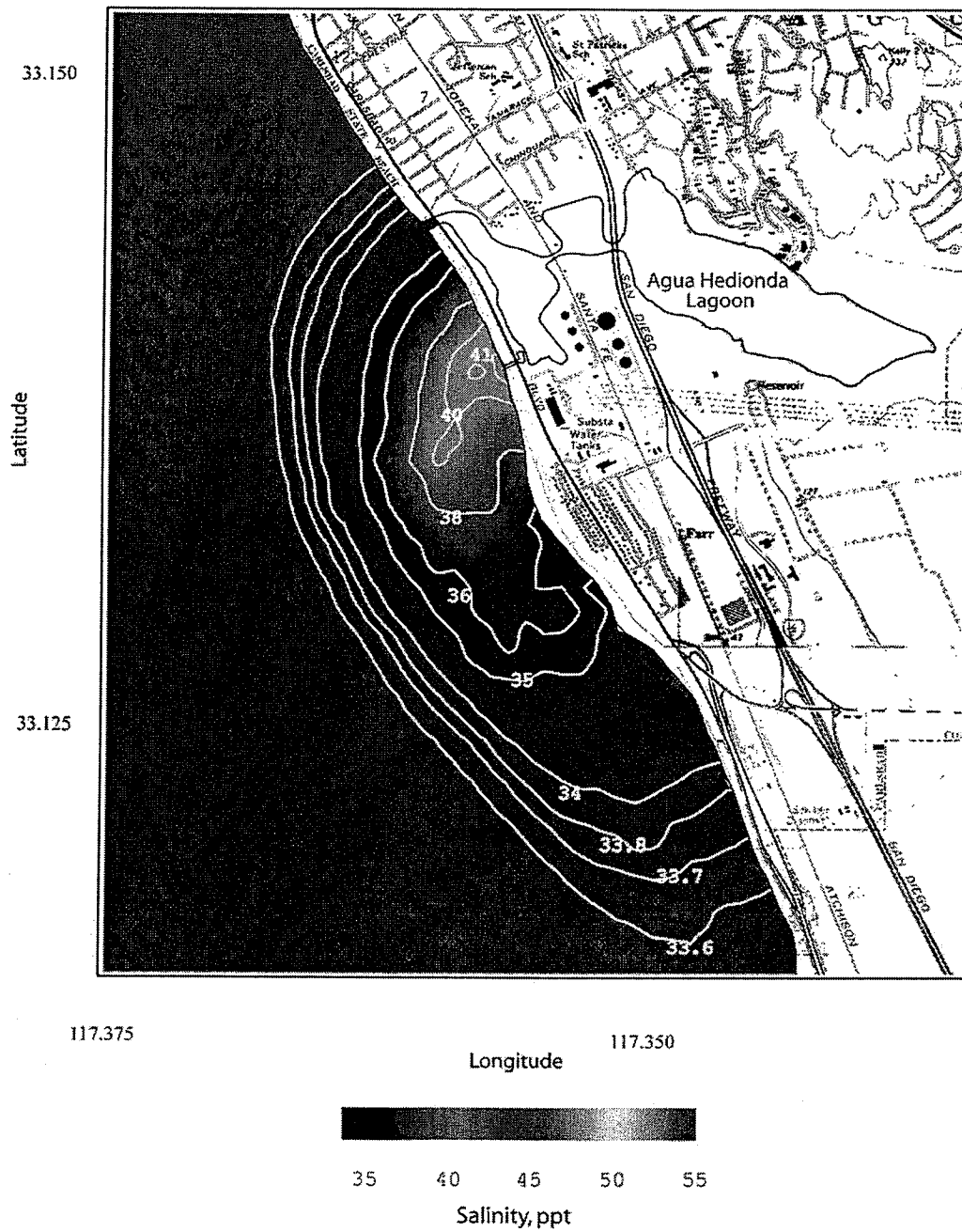
Figure 17. Scenario 4 worst case with one Unit 5 circulation pump, and two Unit 1 pumps for \Delta T = 0^{\circ}C . Daily average of the bottom salinity of concentrated seawater for R.O. = 50 mgd, plant inflow rate = 218.88 mgd, combined discharge = 168.88 mgd, ambient ocean salinity = 33.51 ppt, ocean conditions - 17 Aug 1992.
