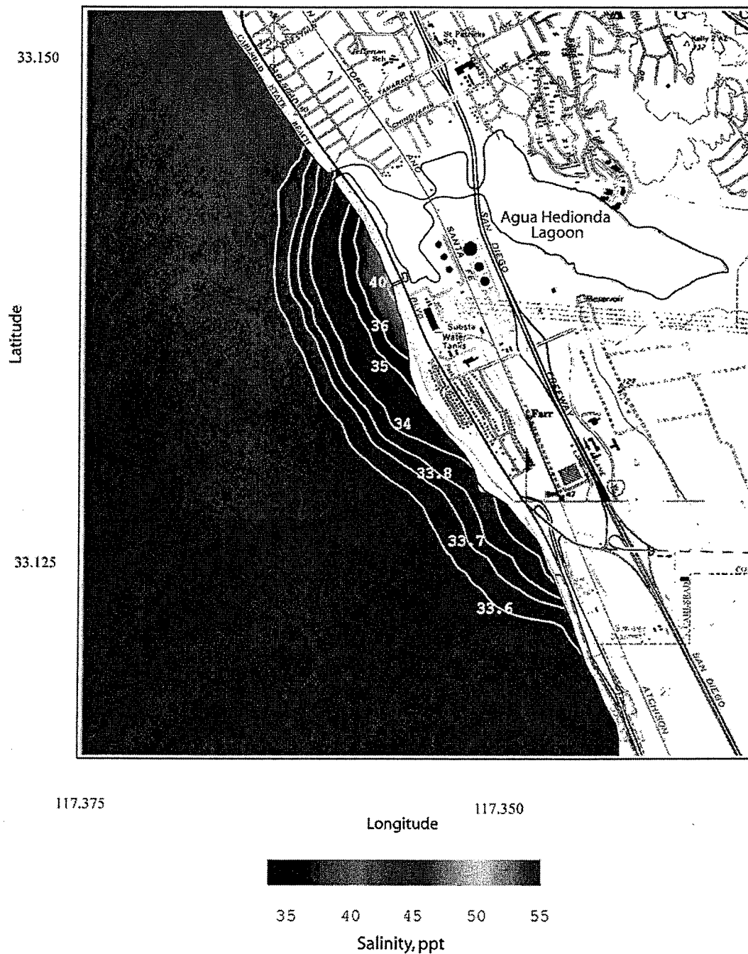
Figure 11. Scenario 2 worst case with all circulation pumps - Units 1&2, and one pump - Unit 3 for \Delta T = 0^\circ\text{C} . Daily depth-averaged salinity of concentrated seawater for R.O. = 50 mgd, plant inflow rate = 172.8 mgd, combined discharge = 122.8 mgd, ambient ocean salinity = 33.51 ppt, ocean conditions - 17 Aug 1992.
