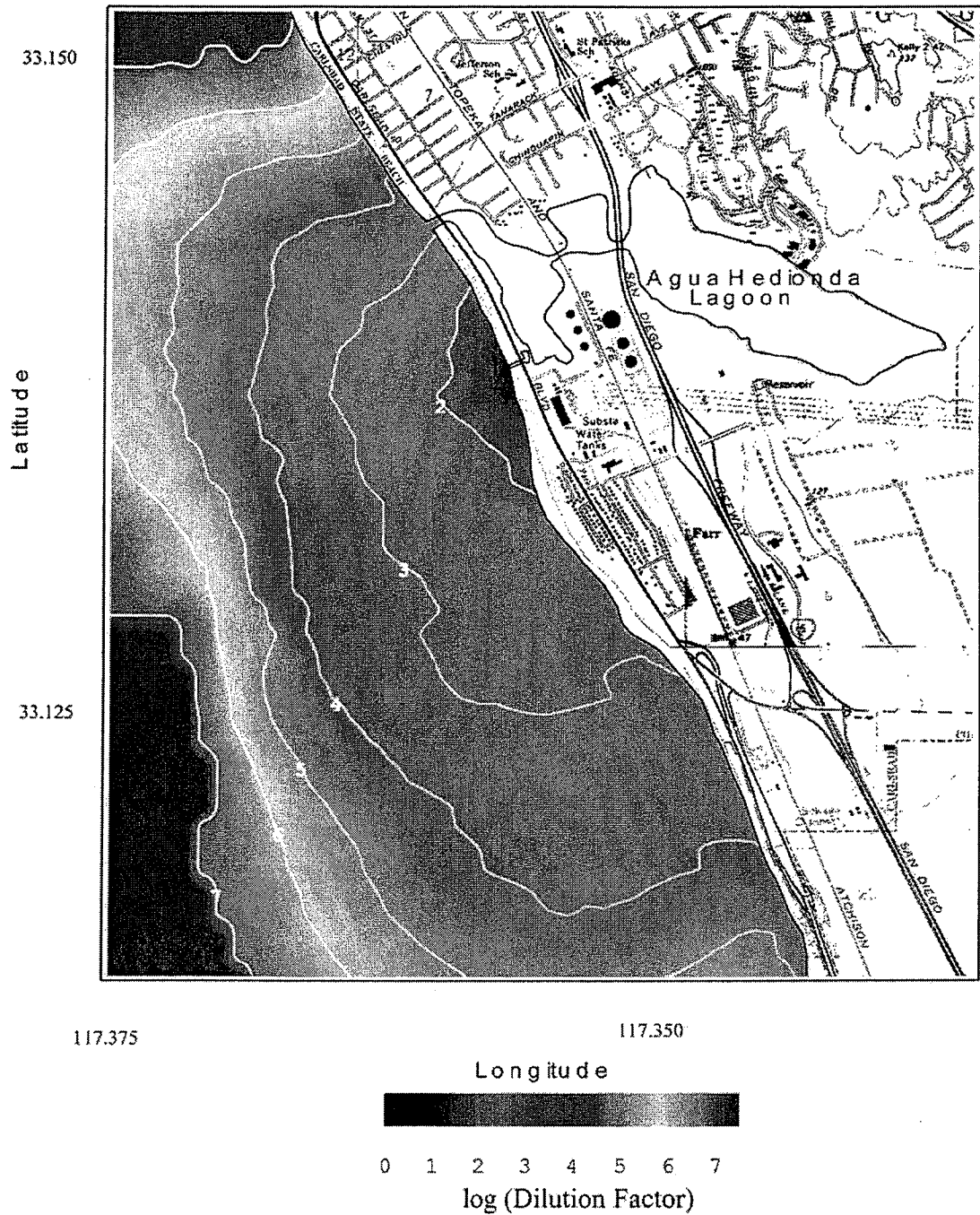
Figure 44. Scenario 5 average case with two Unit 4 circulation pumps for \Delta T = 0^\circ\text{C} . Depth-averaged dilution factor for raw concentrate from desalination. R.O. = 50 mgd, plant inflow rate = 304 mgd, combined discharge = 254 mgd, ambient ocean salinity = 33.52 ppt, ocean conditions, 23 May 1994.
