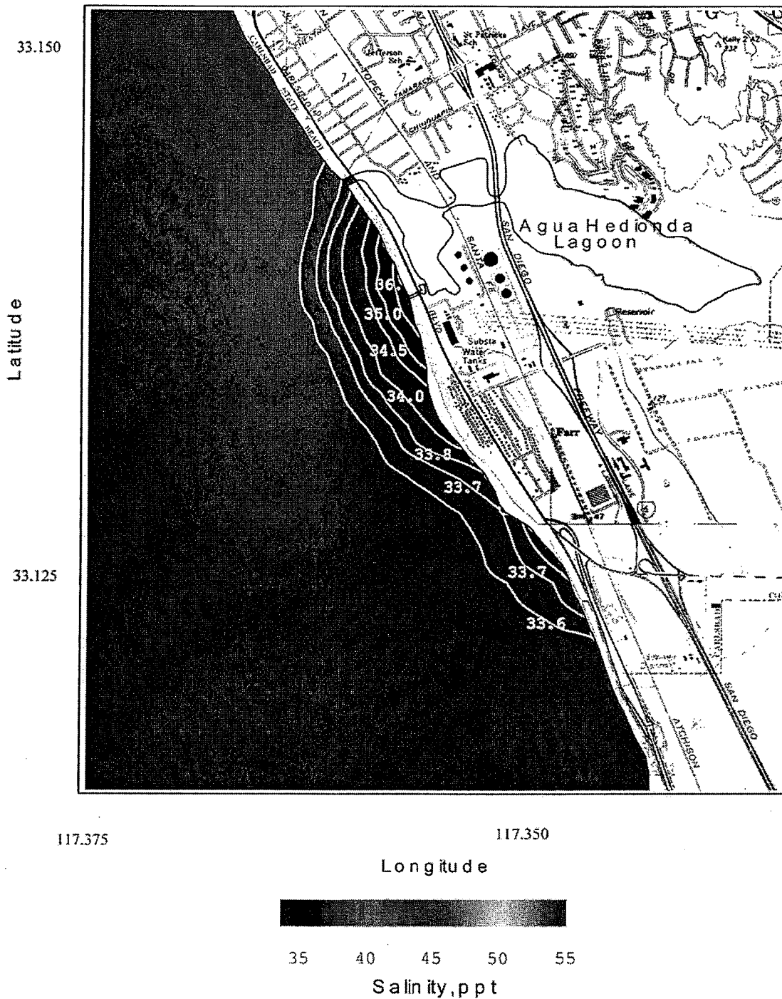
Figure 23. Scenario 5 worst case with two Unit 4 circulation pumps for \Delta T = 0^\circ\text{C} . Daily depth-averaged salinity of concentrated seawater for R.O. = 50 mgd, plant inflow rate = 304 mgd, combined discharge = 254 mgd, ambient ocean salinity = 33.51 ppt, ocean conditions, 17 Aug 1992.
