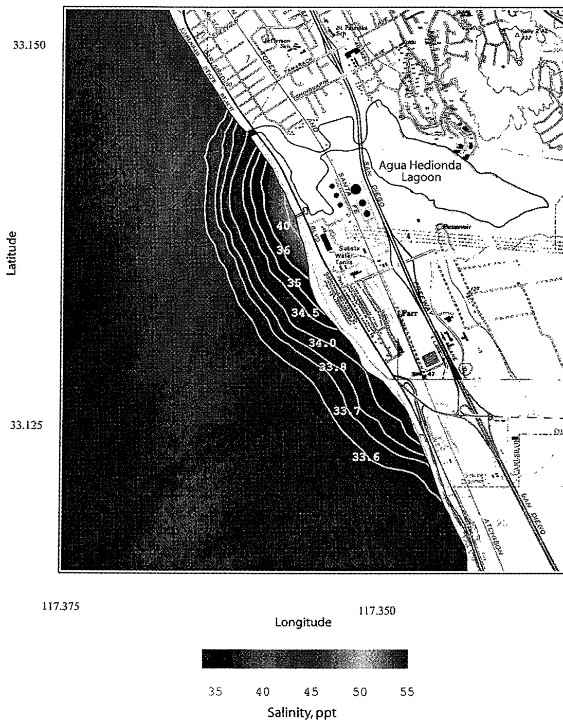
Figure 27. Scenario 1 average case with one Unit 5 circulation pump for \Delta T = 0^\circ\text{C} . Daily depth-averaged salinity of concentrated seawater for R.O. = 50 mgd, plant inflow rate = 149.76 mgd, combined discharge = 99.76 mgd, ambient ocean salinity = 33.52 ppt, ocean conditions - 23 May 1994.
