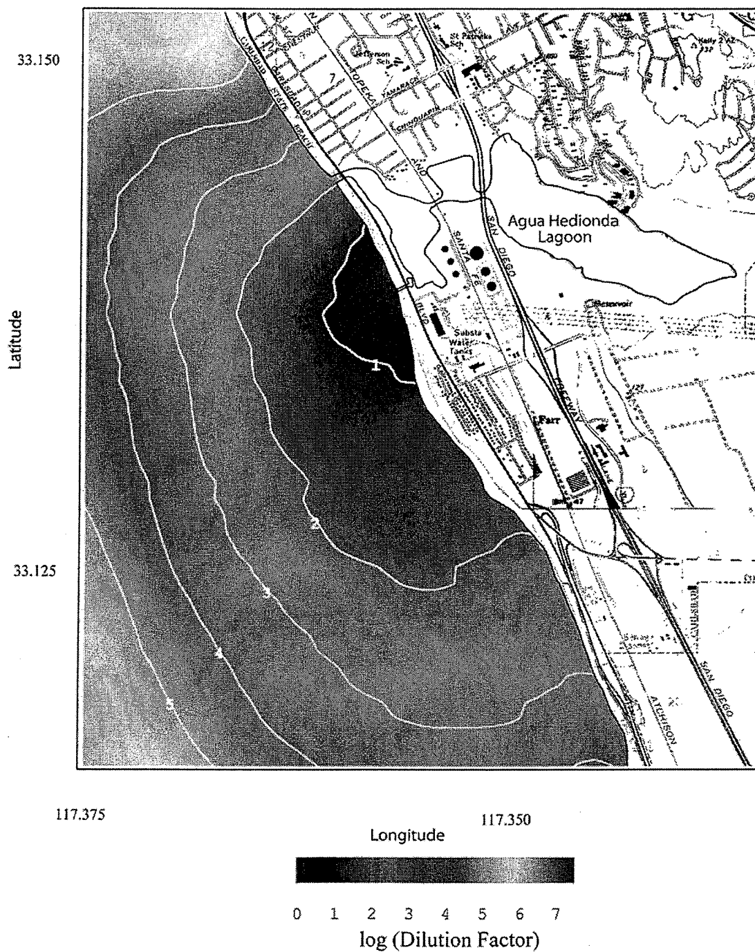
Figure 26. Scenario 1 average case with one Unit 5 circulation pump for DT = 0^{\circ}C . Seafloor dilution factor for raw concentrate from desalination. R.O. = 50 mgd, plant inflow rate = 149.76 mgd, combined discharge = 99.76 mgd, ambient ocean salinity = 33.52 ppt, ocean conditions - 23 May 1994.
