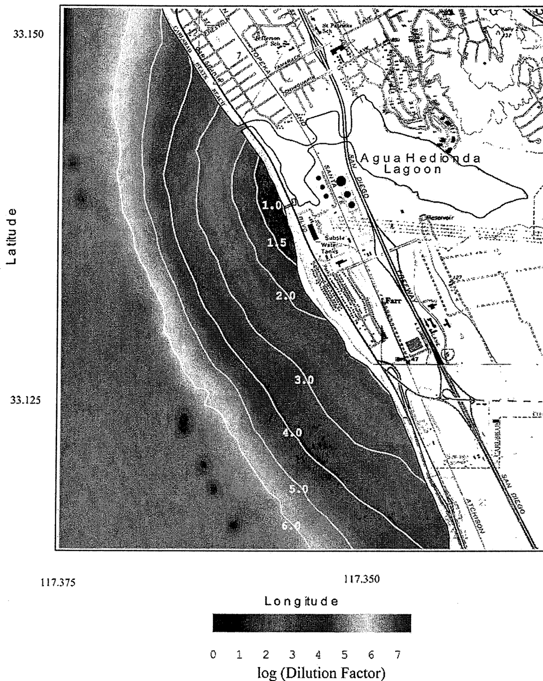
Figure 24. Scenario 5 worst case with two Unit 4 circulation pumps for \Delta T = 0^{\circ}\text{C} . Depth-averaged dilution factor for raw concentrate from desalination. R.O. = 50 mgd, plant inflow rate = 304 mgd, combined discharge = 254 mgd, ambient ocean salinity = 33.51 ppt, ocean conditions, 17 Aug 1992.
