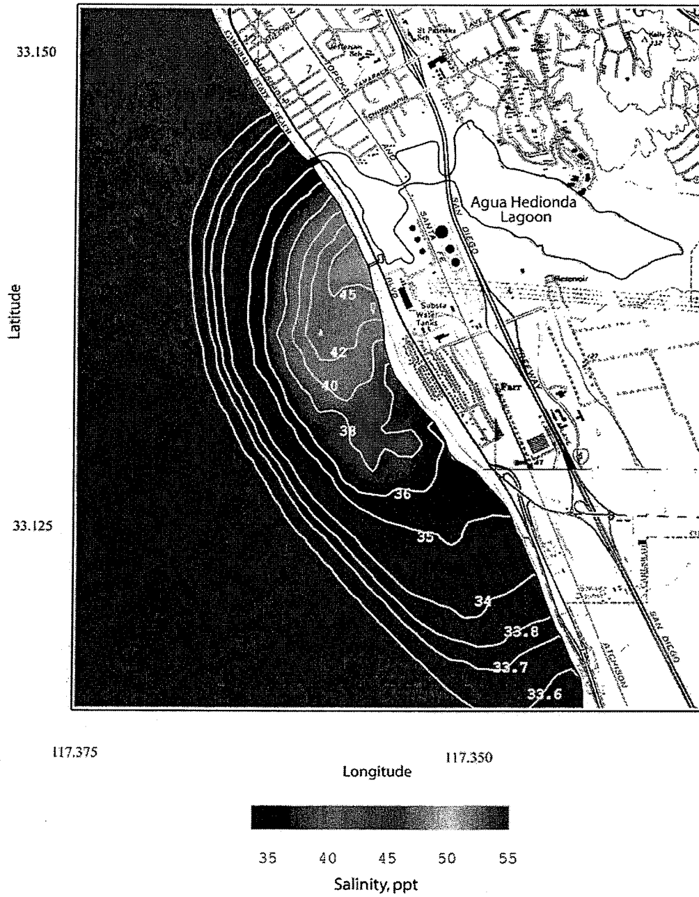
Figure 5. Scenario 1 worst case with one Unit 5 circulation pump for \Delta T = 0^\circ\text{C} . Daily average of the bottom salinity of concentrated seawater for R.O. = 50 mgd, plant inflow rate = 149.76 mgd, combined discharge = 99.76 mgd, ambient ocean salinity = 33.51 ppt, ocean conditions - 17 Aug 1992.
