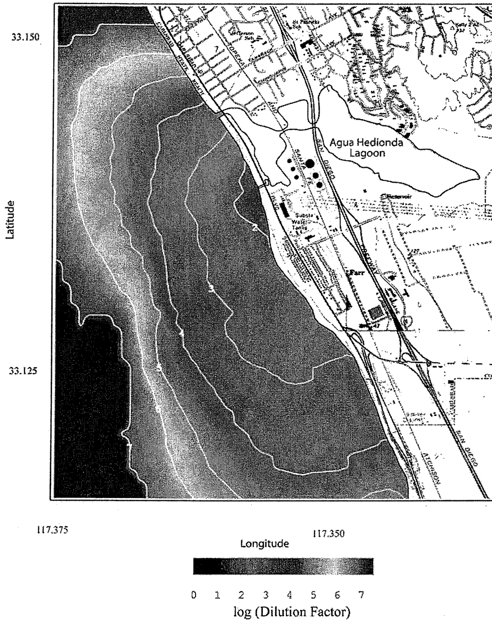
Figure 40. Scenario 4 average case with one Unit 5 circulation pump, and two Unit 1 pumps for \Delta T = 0^\circ\text{C} . Depth-averaged dilution factor for raw concentrate from desalination. R.O. = 50 mgd, plant inflow rate = 218.88 mgd, combined discharge = 168.88 mgd, ambient ocean salinity = 33.52 ppt, ocean conditions - 23 May 1994.
