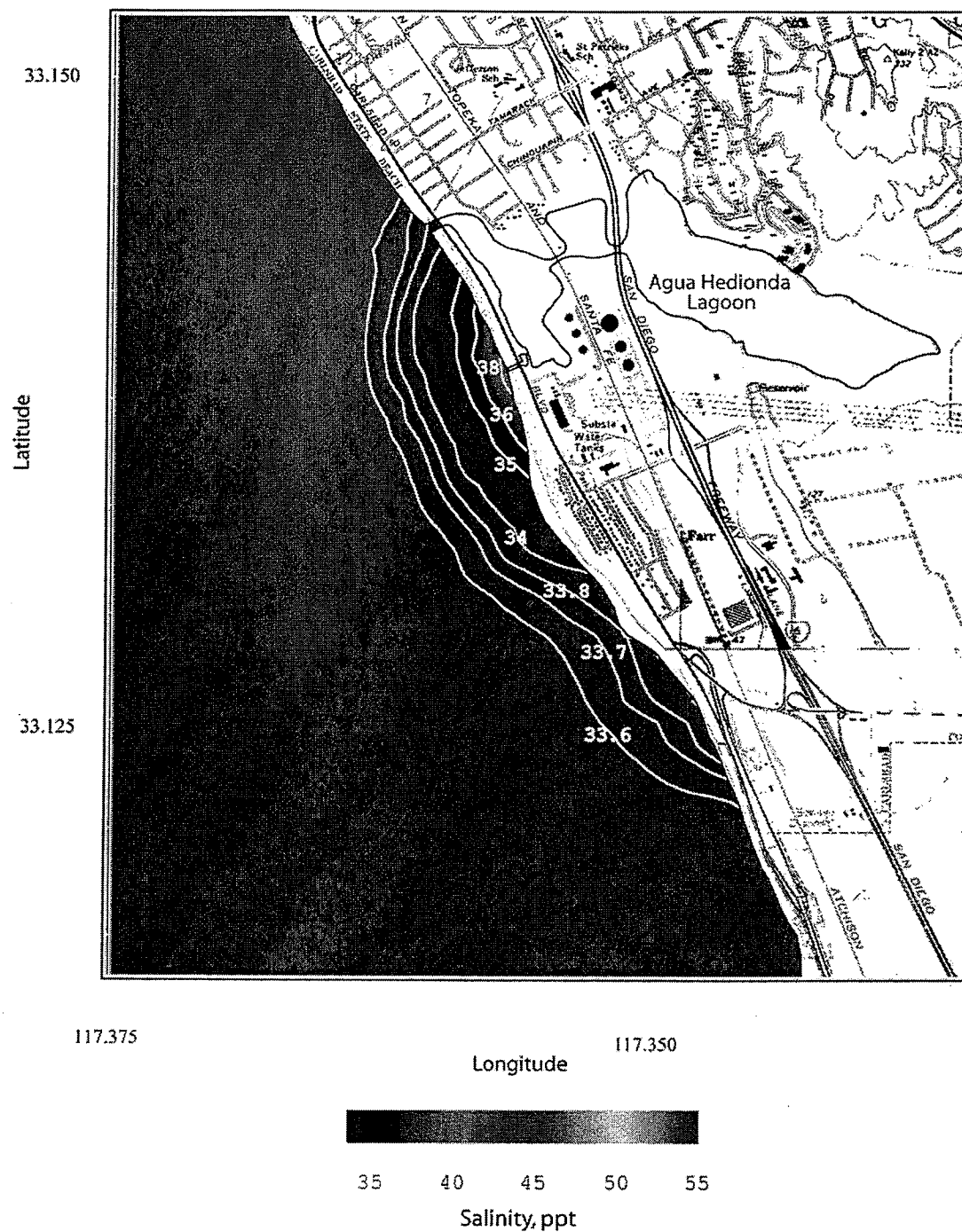
Figure 19. Scenario 4 worst case with one Unit 5 circulation pump, and two Unit 1 pumps for \Delta T = 0^{\circ}\text{C} . Daily depth-averaged salinity of concentrated seawater for R.O. = 50 mgd, plant inflow rate = 218.88 mgd, combined discharge = 168.88 mgd, ambient ocean salinity = 33.51 ppt, ocean conditions - 17 Aug 1992.
