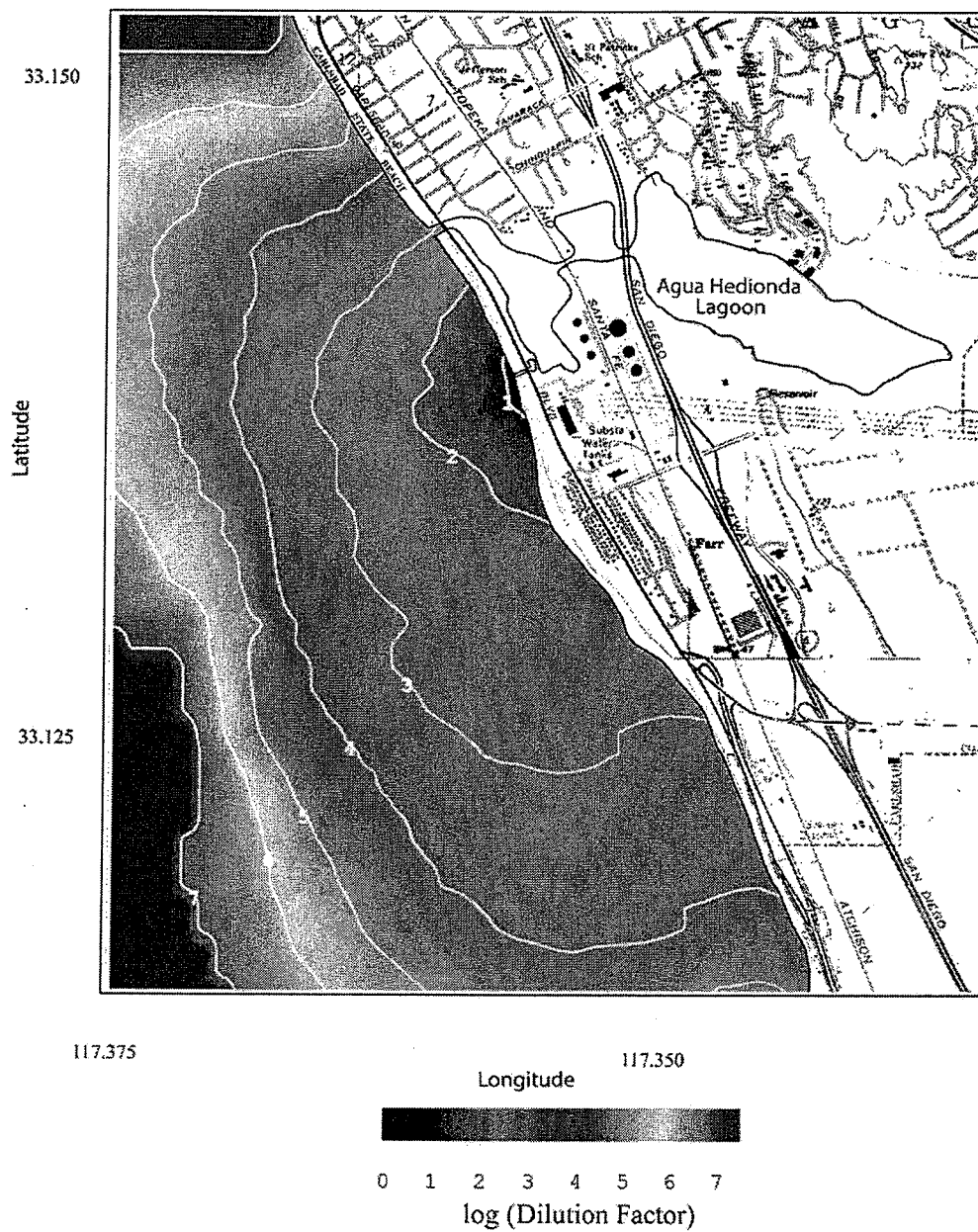
Figure 36. Scenario 3 average case with one Unit 5 circulation pump, and one Unit 1 pump for \Delta T = 0^\circ\text{C} . Depth-averaged dilution factor for raw concentrate from desalination. R.O. = 50 mgd, plant inflow rate = 184.32 mgd, combined discharge = 134.32 mgd, ambient ocean salinity = 33.52 ppt, ocean conditions - 23 May 1994.
