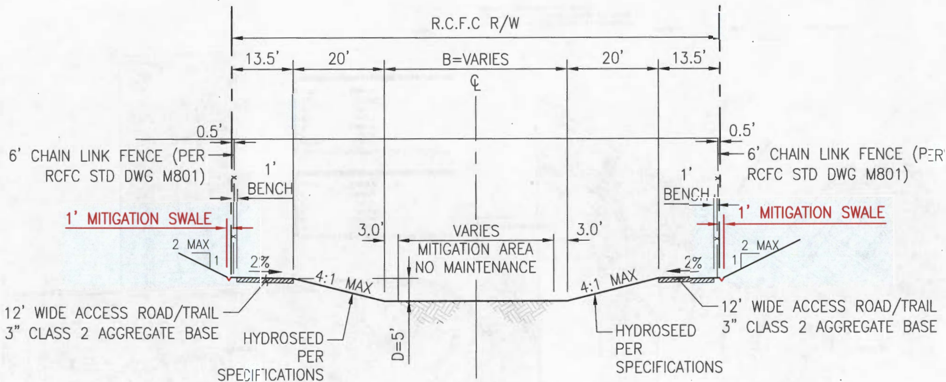
TYPICAL CHANNEL CROSS SECTION
