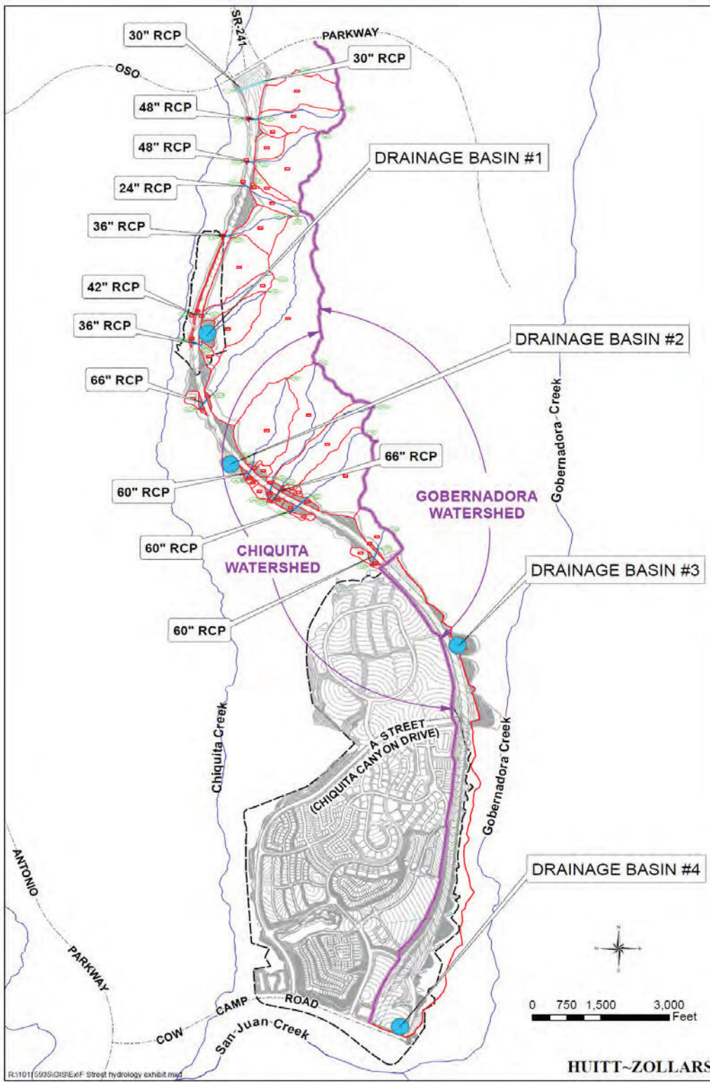
Figure 1: Proposed Hydrologic Boundaries
