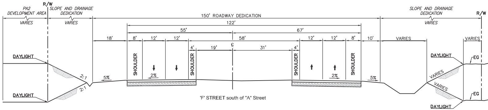
"F" STREET TYPICAL STREET SECTIONS
