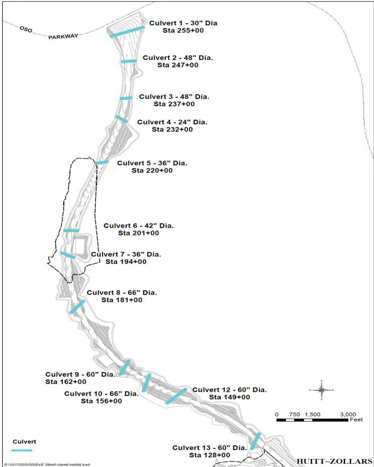
Figure 2: Cross-Culvert Locations
