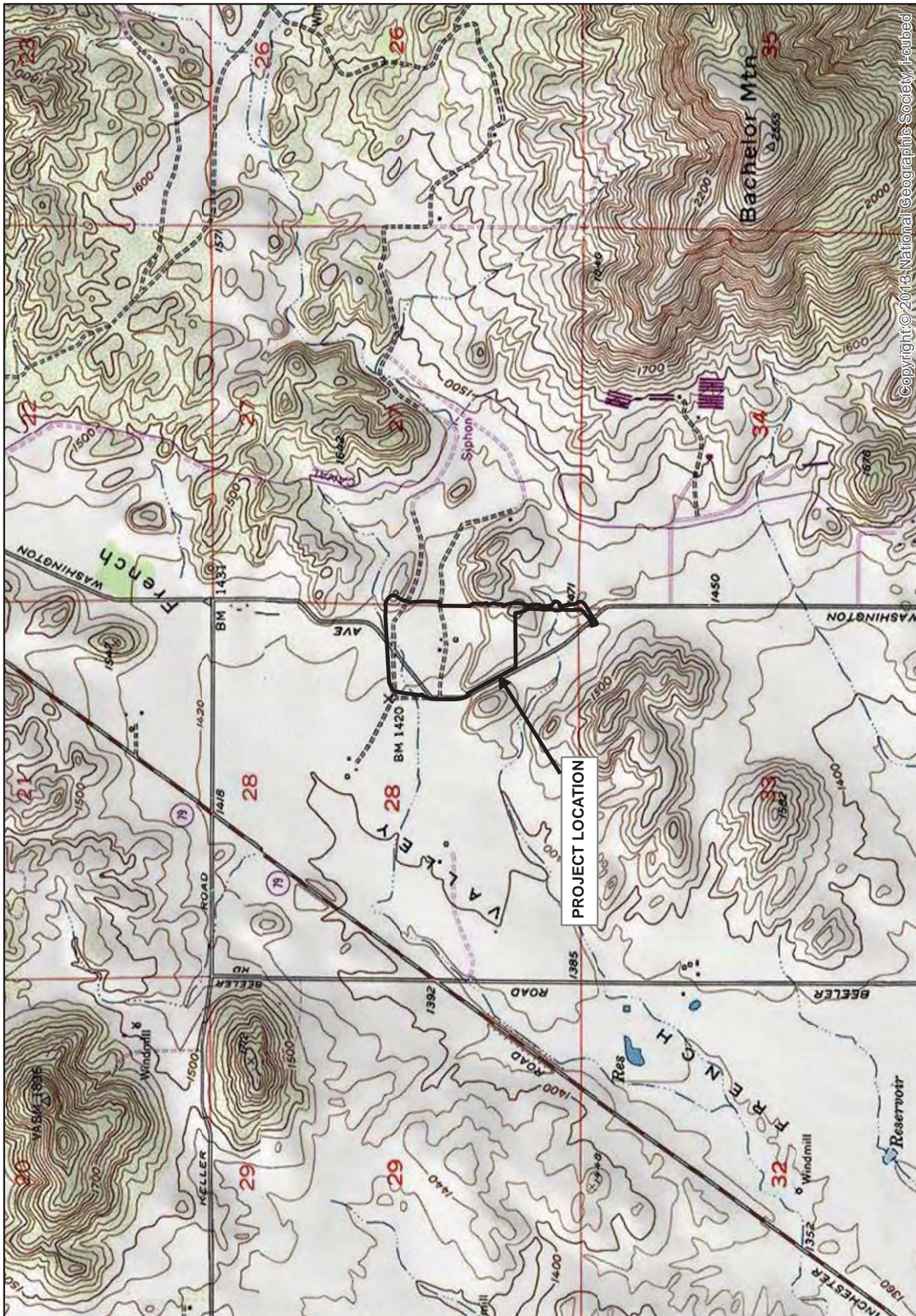
Adapted from USGS Bachelor Mountain, CA quadrangle
