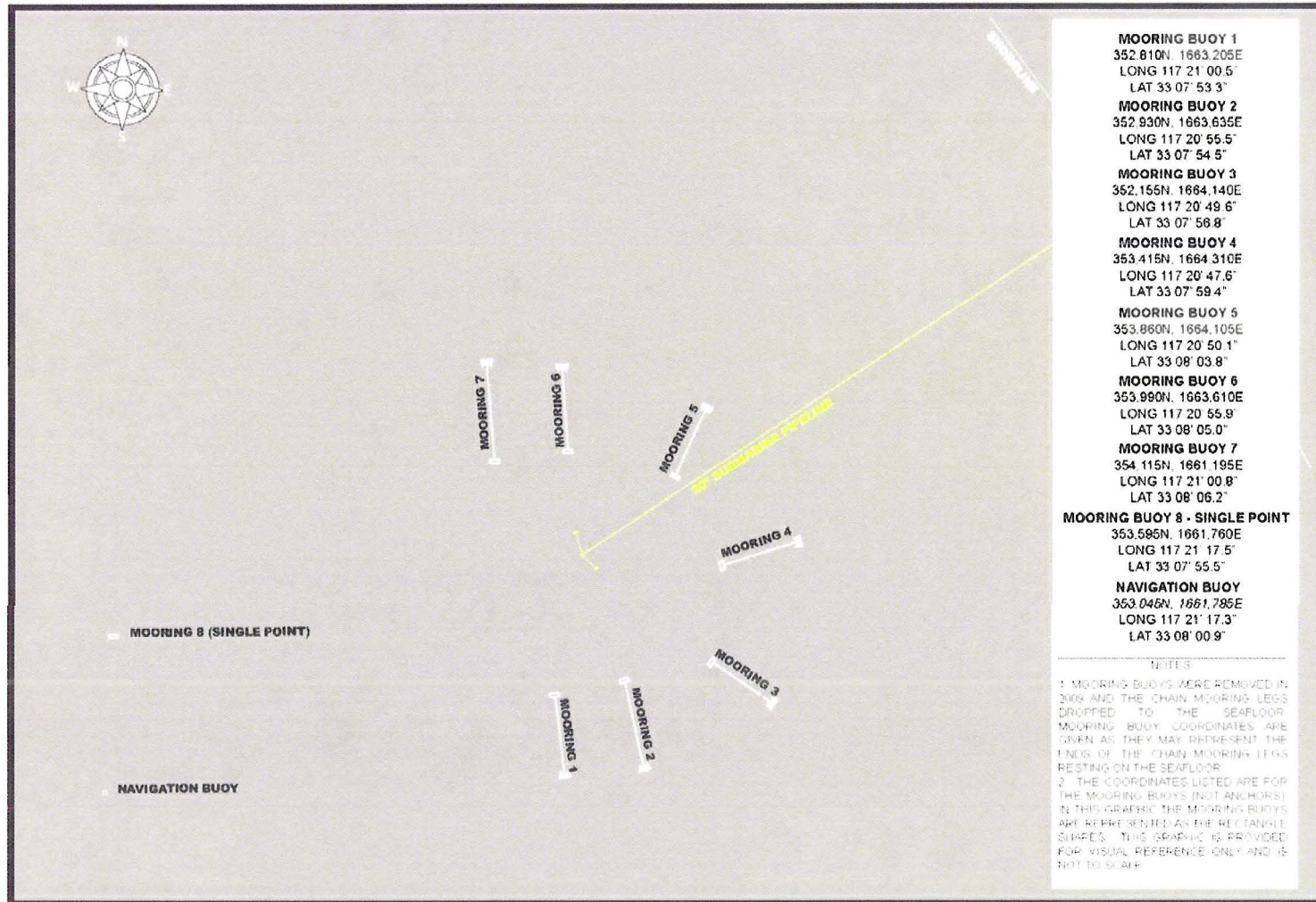
Figure 1-2. Mooring Area Detail
