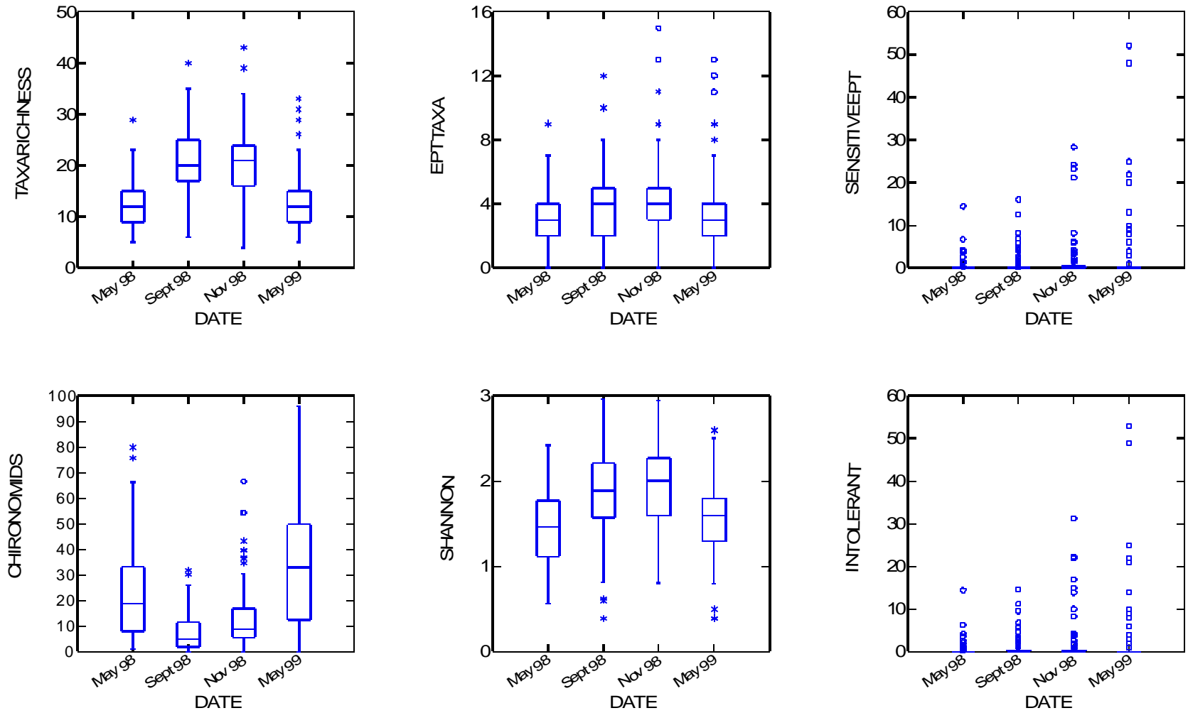
Figure 6. Boxplots describing the relationship between major bioassessment metrics and sampling date. See Appendix VII for an explanation of axes.
