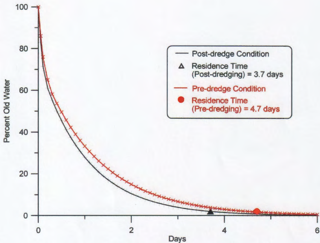
Figure 11. Water mass exchange rating function and residence time in the East Basin of Agua Hedionda Lagoon for pre-dredge (red) and post-dredge (black) bathymetry.
