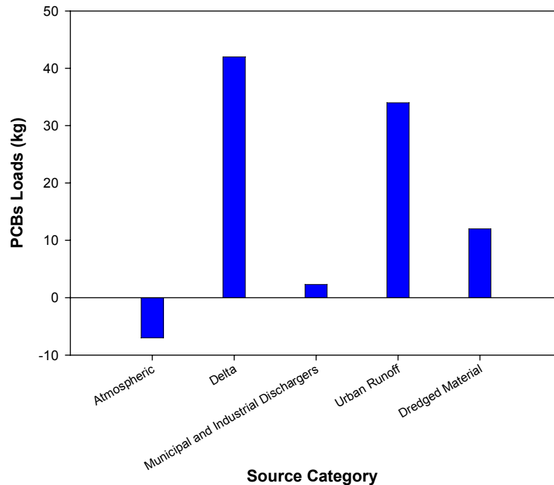
Figure 17-Sources and Loads of PCBs to San Francisco Bay
