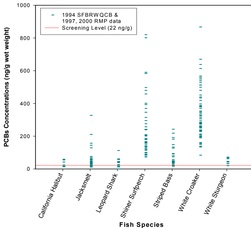
Figure 4-PCBs Concentrations in San Francisco Bay Fish. (Source www.sfei.org )
