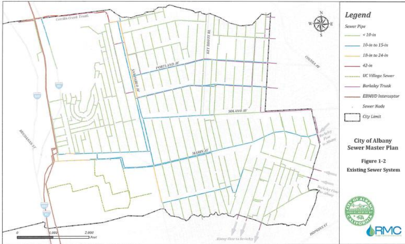
Figure B-1. Sewer Map
