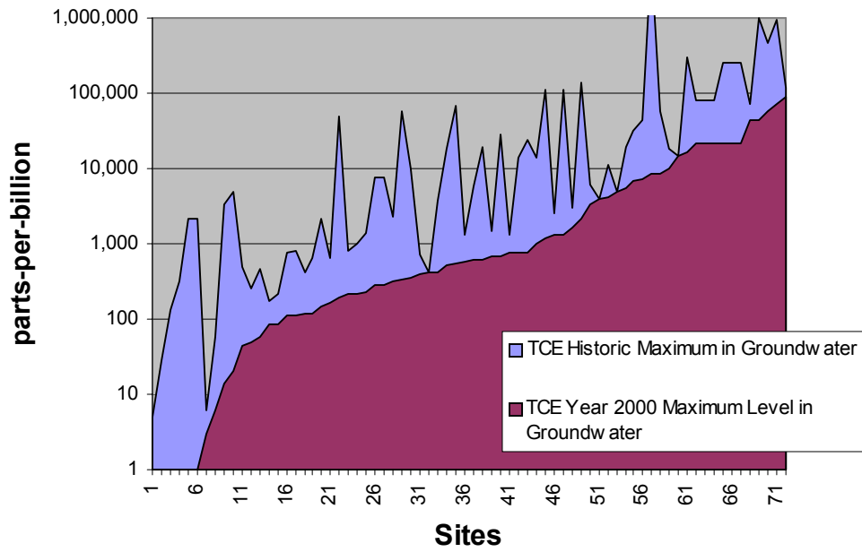
Figure 30. Maximum Levels of TCE in Groundwater at South Bay Sites
