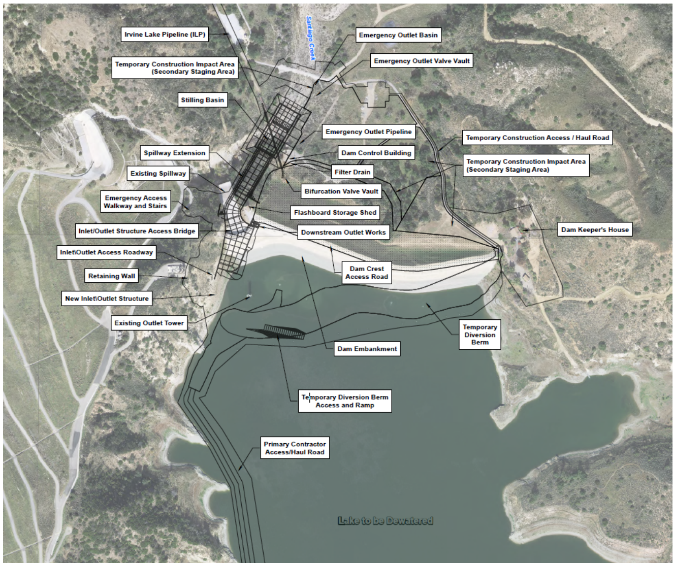
Figure 6: Santiago Dam Construction Features
