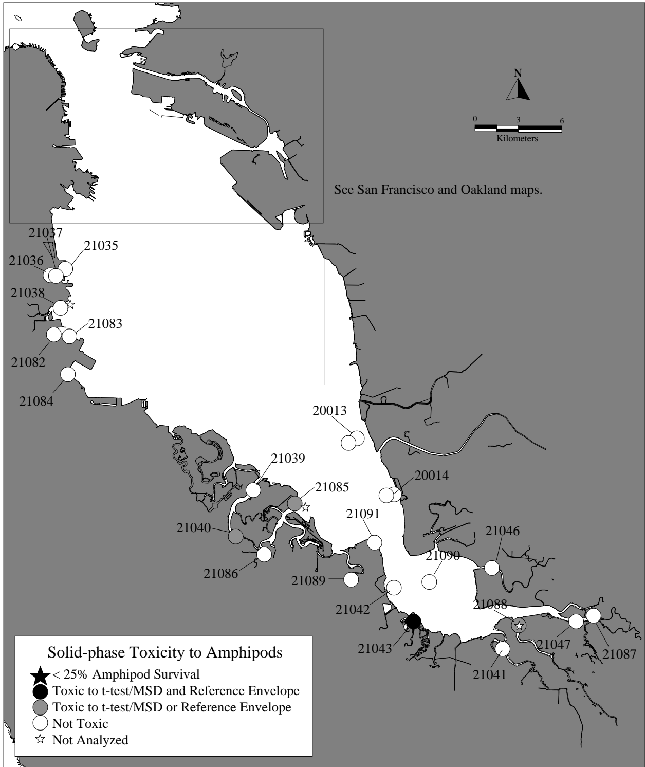
Figure 4d. Results of Amphipod Toxicity Screening for Stations in South San Francisco Bay.
