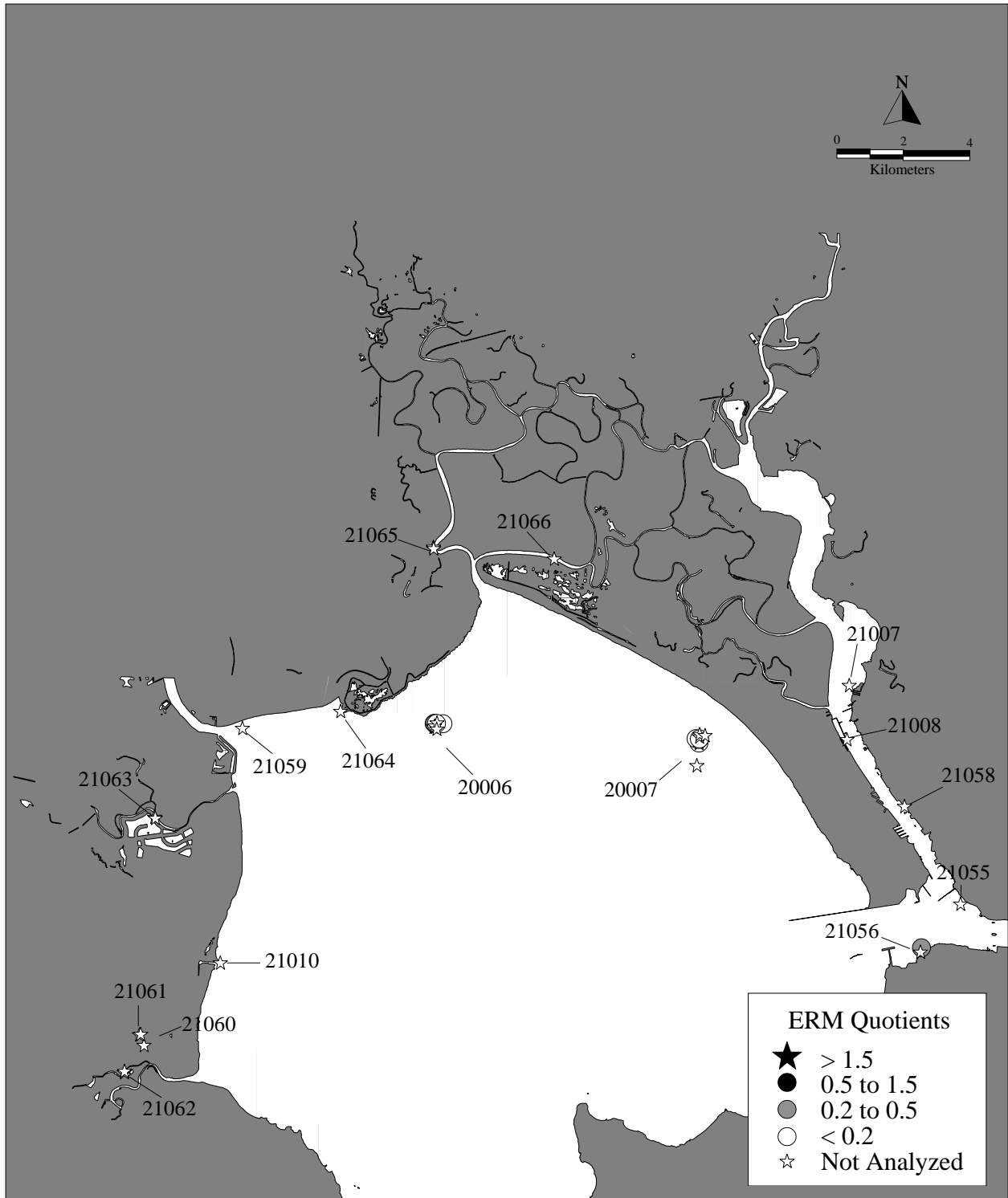
Figure 9b. Mean ERM Quotient Values for Stations in San Pablo Bay.
