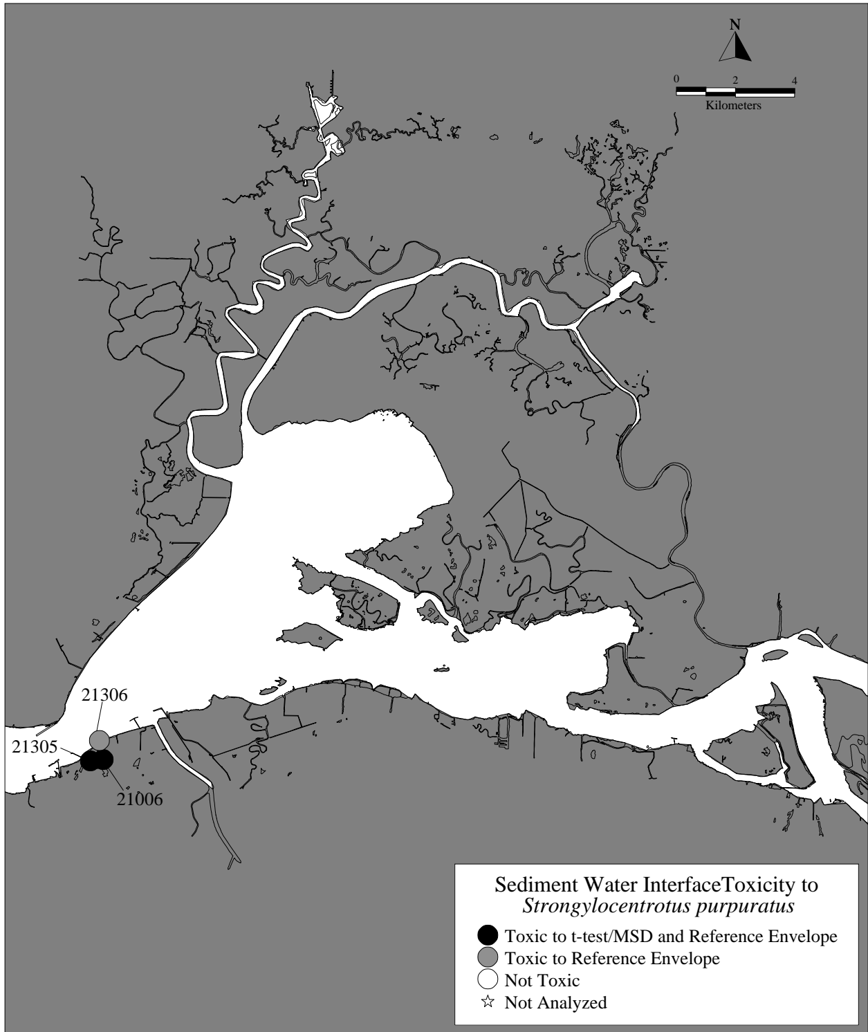
Figure 8a. Results of Sediment Water Interface Toxicity Confirmation for Stations in Suisun Bay.
