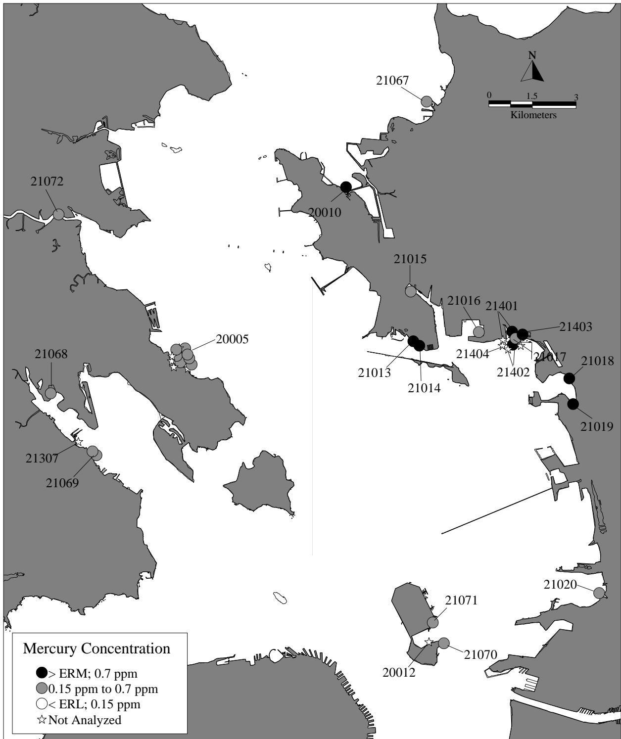
Figure 11c. Mercury Concentrations at Stations in Central San Francisco Bay.
