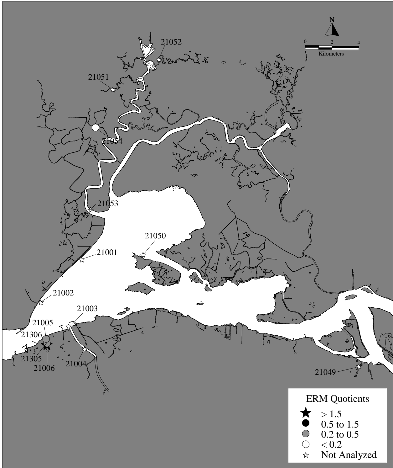
Figure 9a. Mean ERM Quotient Values for Stations in Suisun Bay.
