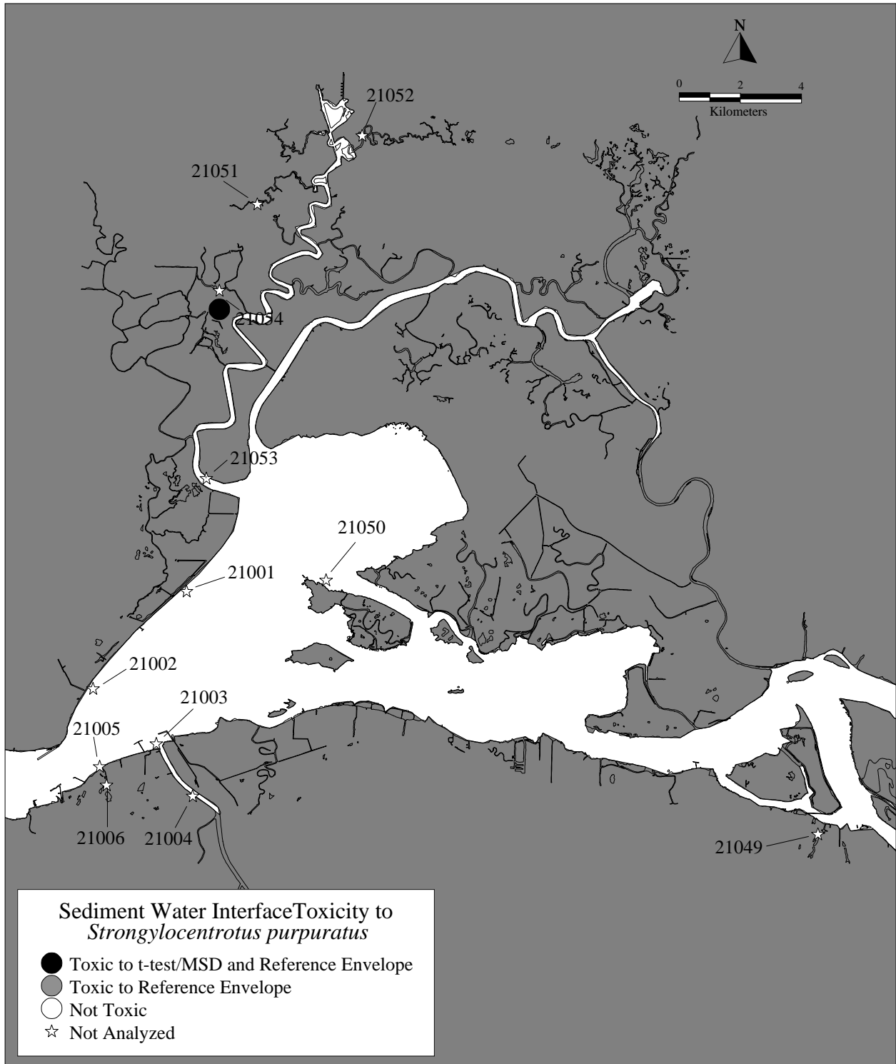
Figure 6a. Results of Sediment-Water Interface Toxicity Screening for Stations in Suisun Bay.
