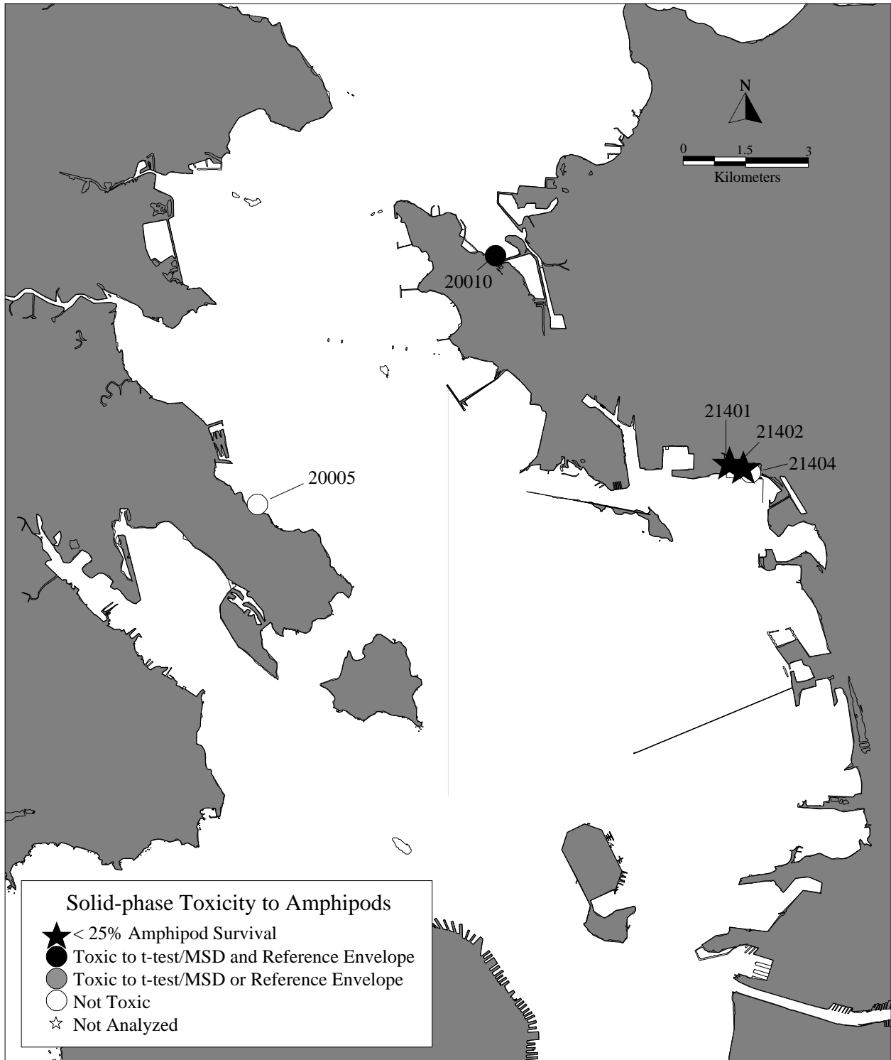
Figure 7c. Results of Amphipod Toxicity Confirmation for Stations in Central San Francisco Bay.
