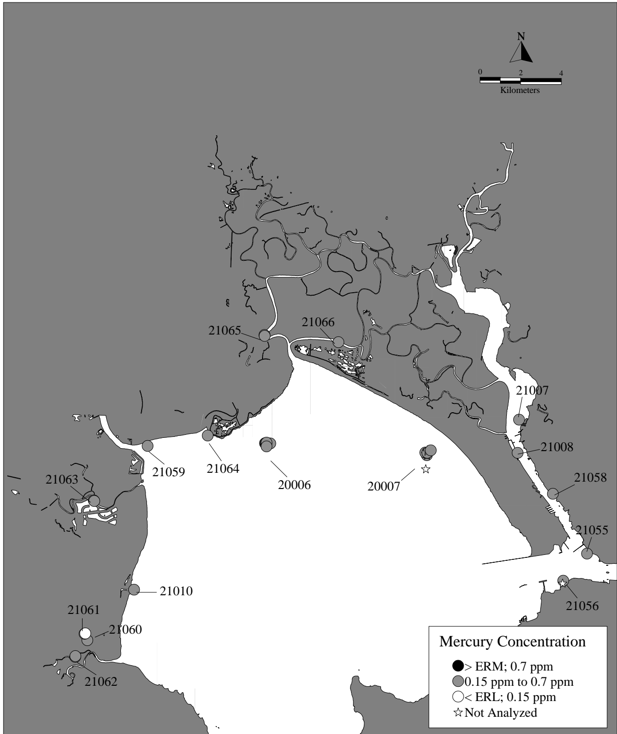
Figure 11b. Mercury Concentrations at Stations in San Pablo Bay.
