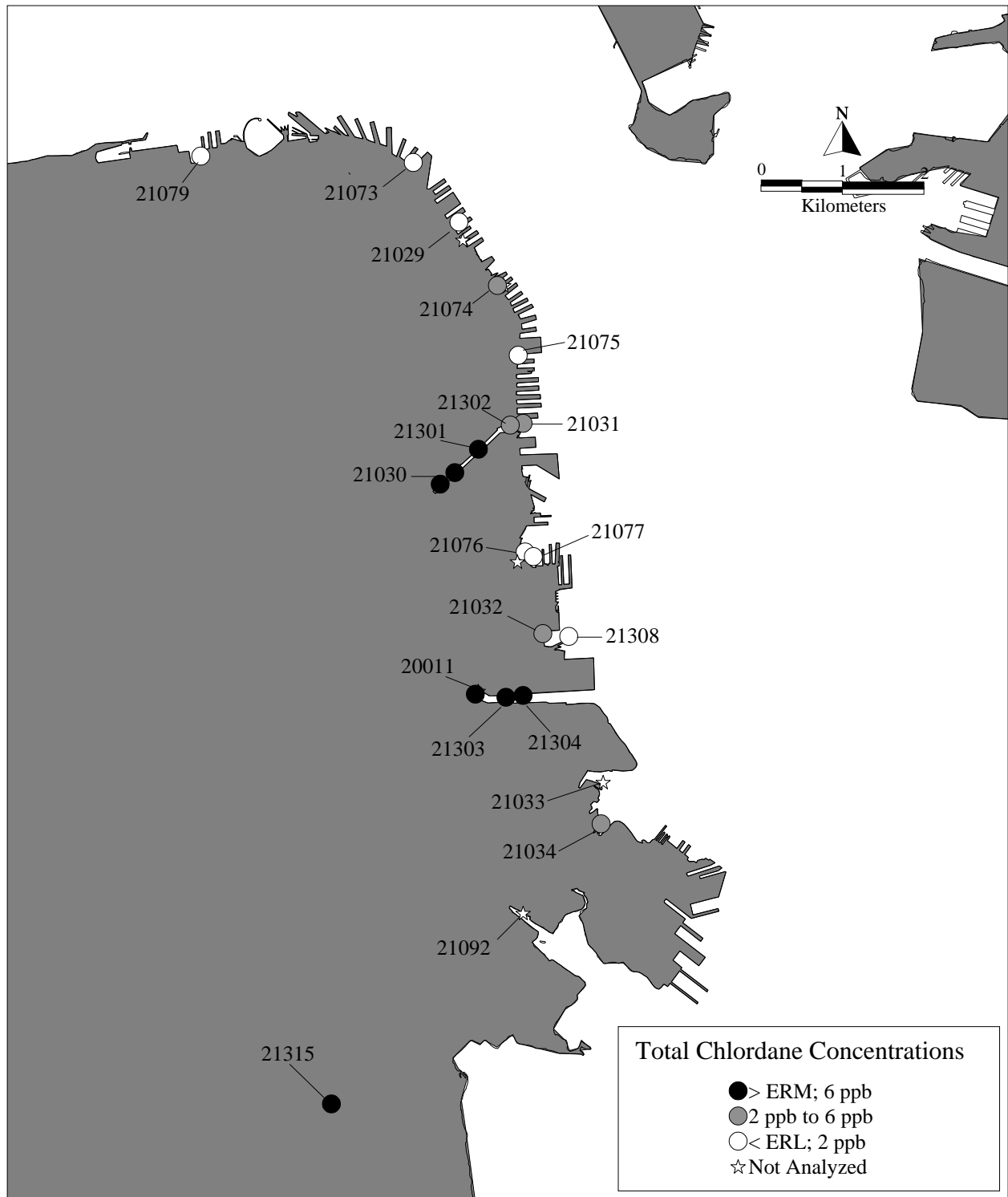
Figure 12f. Total Chlordane Concentrations at Stations in San Francisco.
