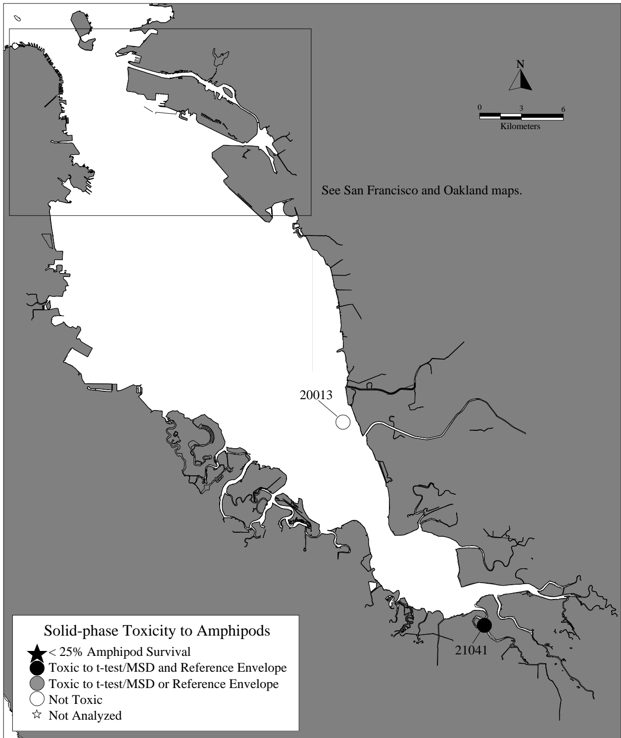
Figure 7d. Results of Amphipod Toxicity Confirmation for Stations in South San Francisco Bay.
