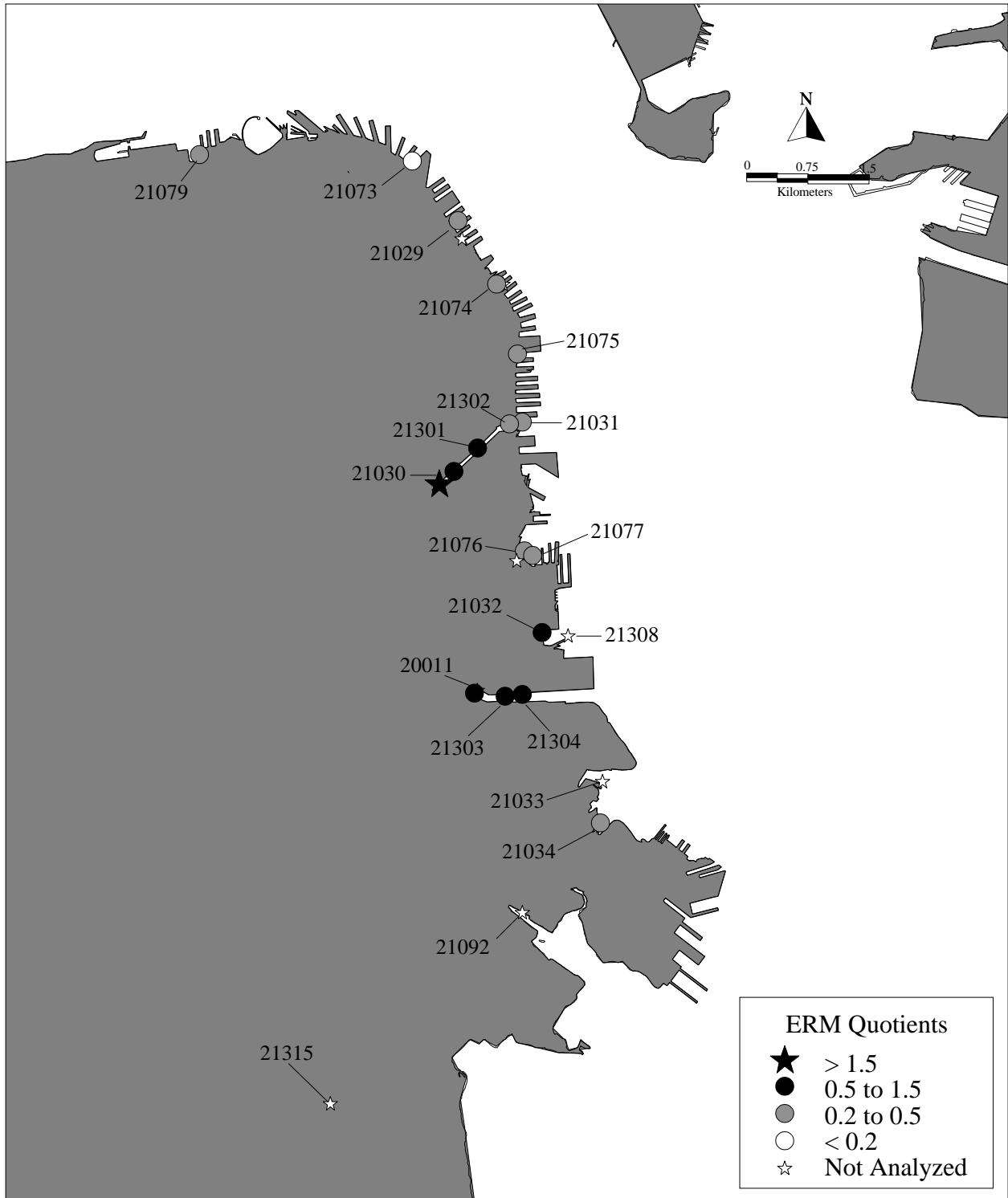
Figure 9f. Mean ERM Quotient Values for Stations in San Francisco.
