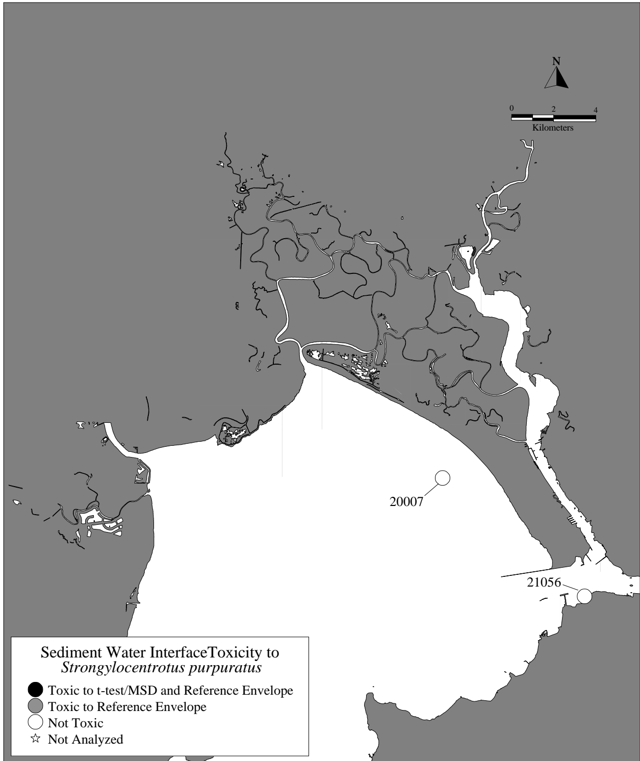
Figure 8b. Results of Sediment Water Interface Toxicity Confirmation for Stations in San Pablo Bay.
