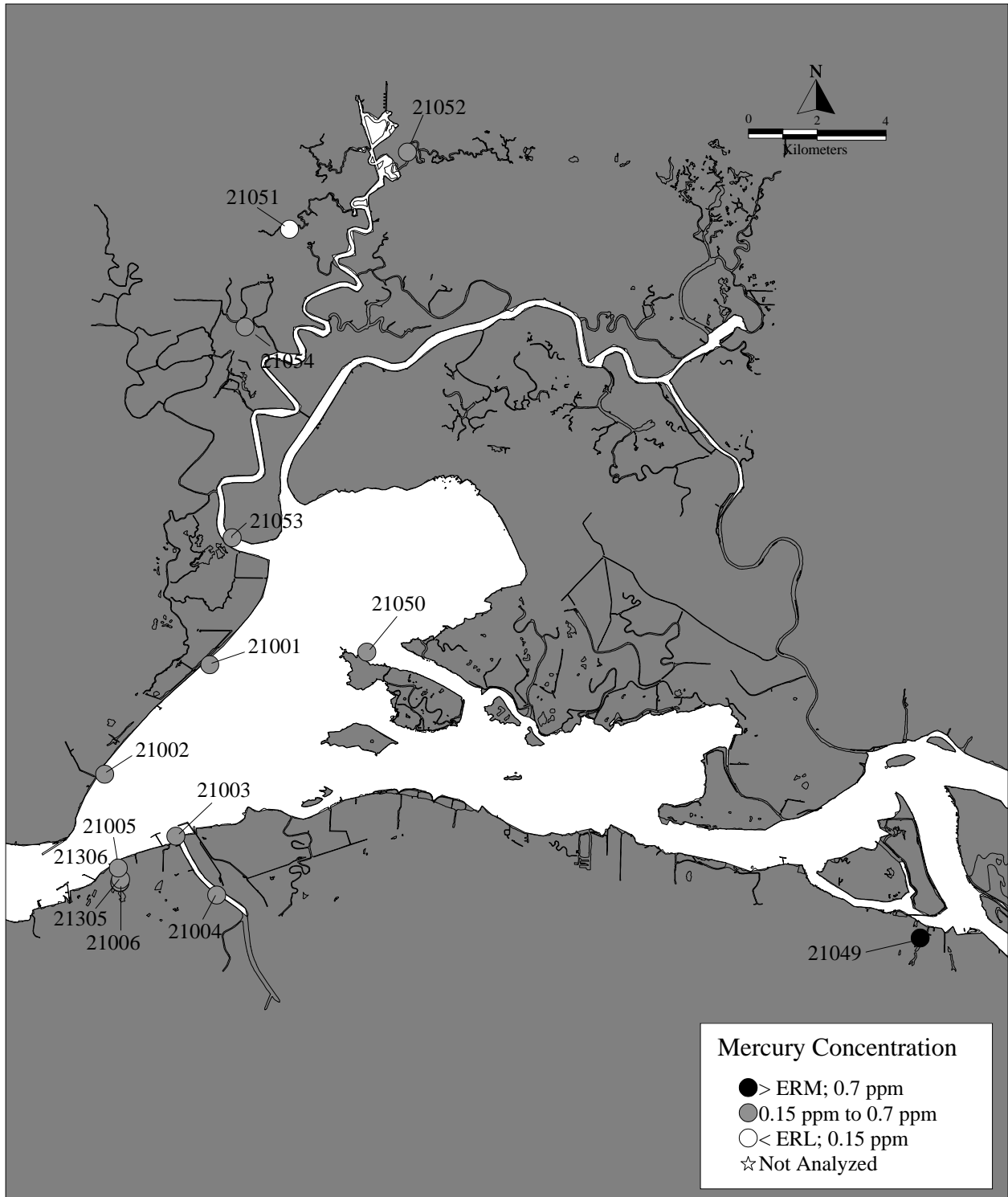
Figure 11a. Mercury Concentrations at Stations in Suisun Bay.
