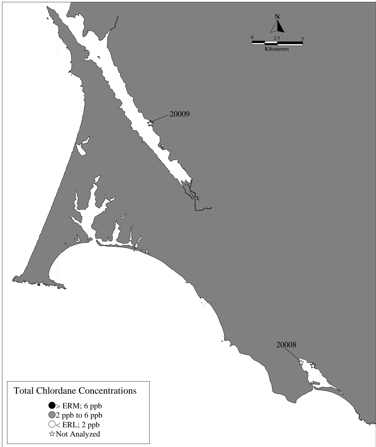
Figure 12g. Total Chlordane Concentrations at Stations in Tomales Bay and Bolinas Lagoon.
