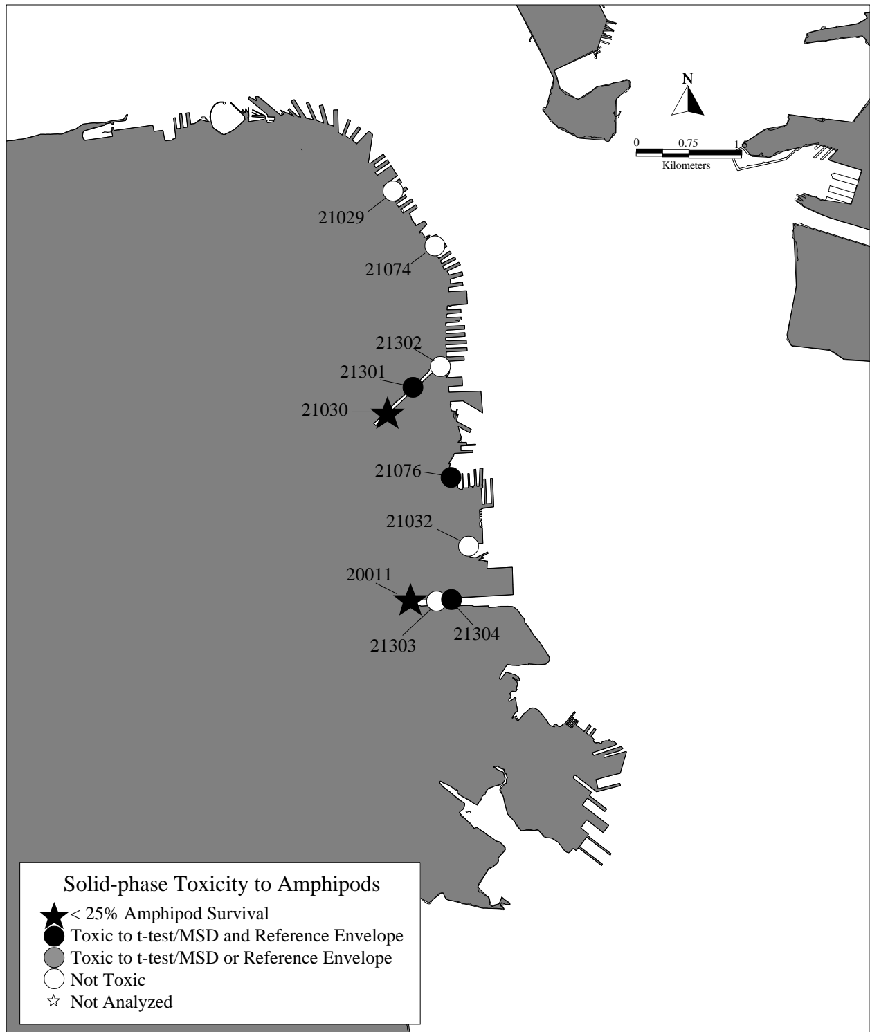
Figure 7f. Results of Amphipod Toxicity Confirmation for Stations in San Francisco.
