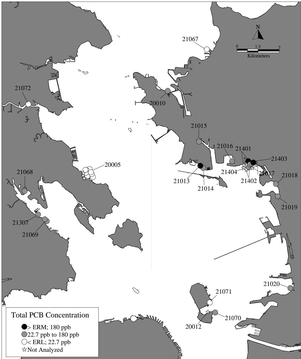
Figure 10c. Total PCB Concentrations at Stations in Central San Francisco Bay.
