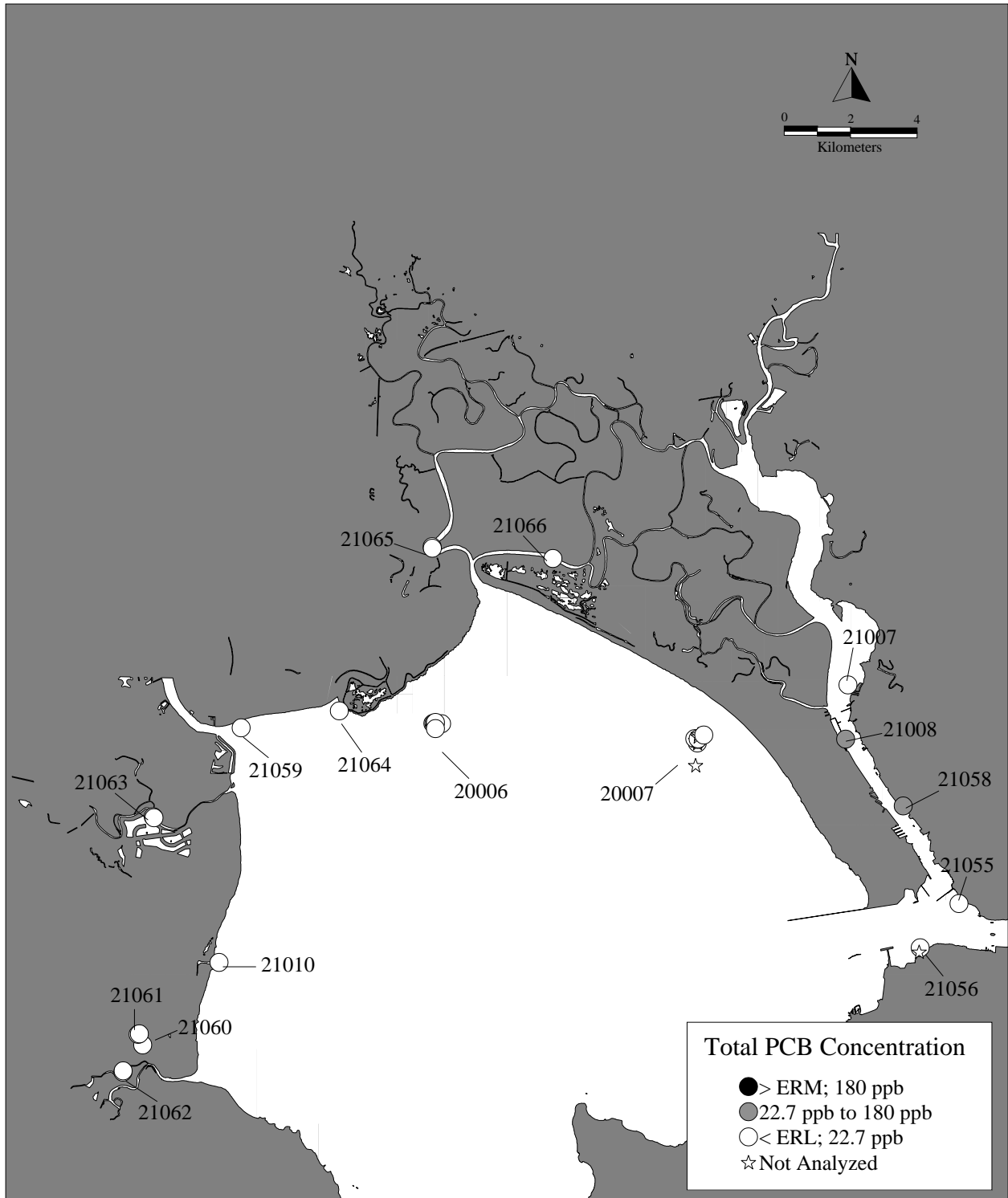
Figure 10b. Total PCB Concentrations at Stations in San Pablo Bay.
