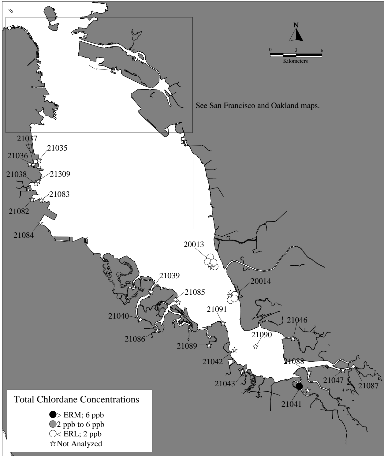
Figure 12d. Total Chlordane Concentrations at Stations in South San Francisco Bay.
