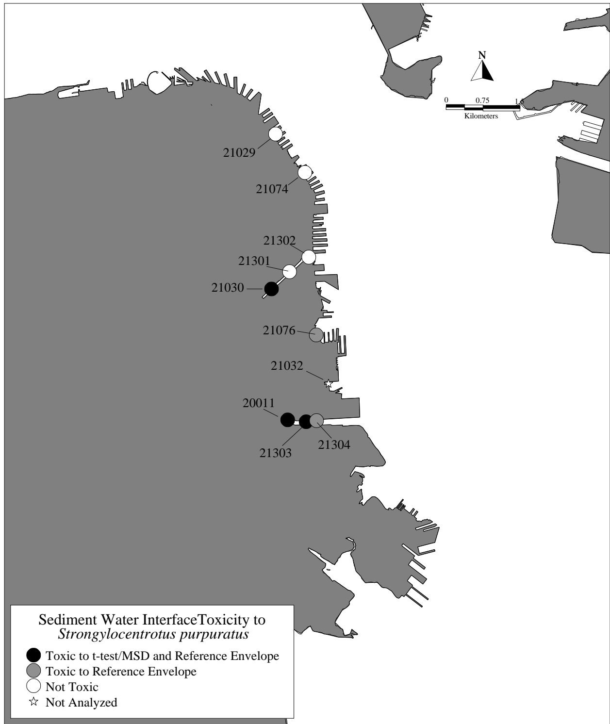
Figure 8f. Results of Sediment Water Interface Toxicity Confirmation for Stations in San Francisco.
