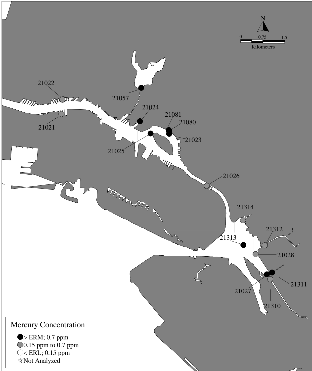
Figure 11e. Mercury Concentrations at Stations in Oakland.
