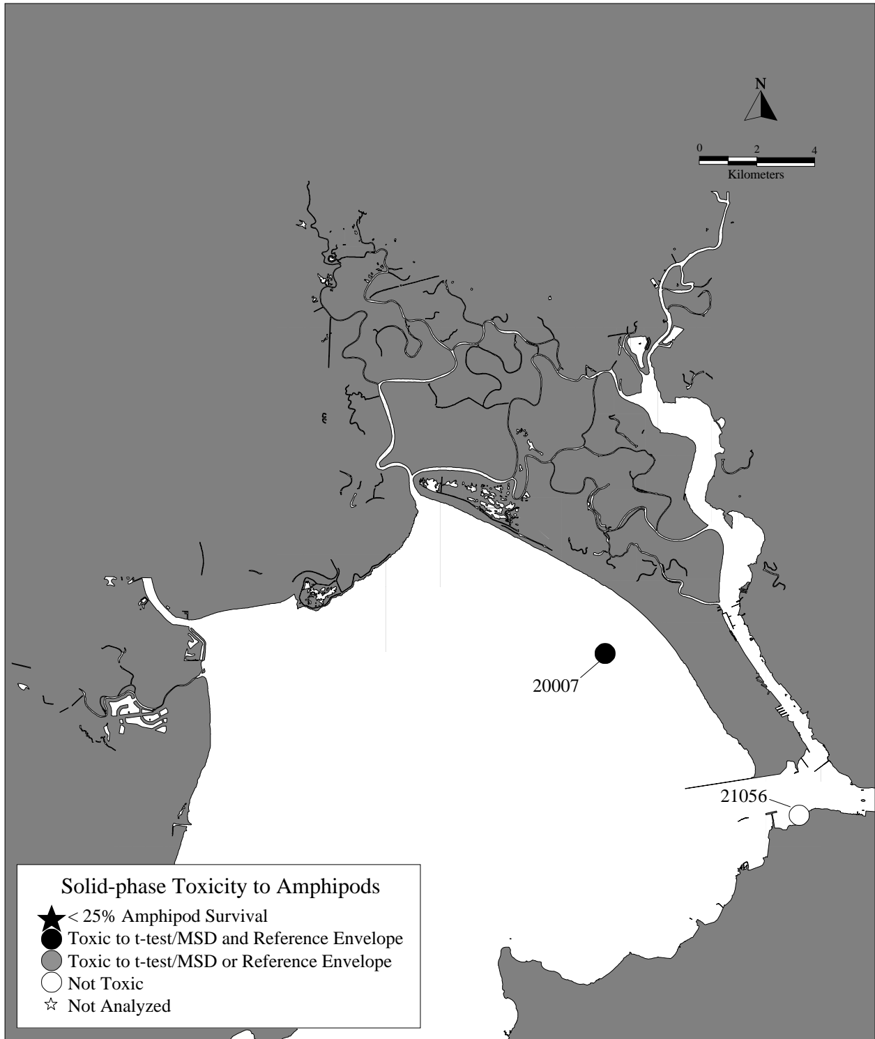
Figure 7b. Results of Amphipod Toxicity Confirmation for Stations in San Pablo Bay.
