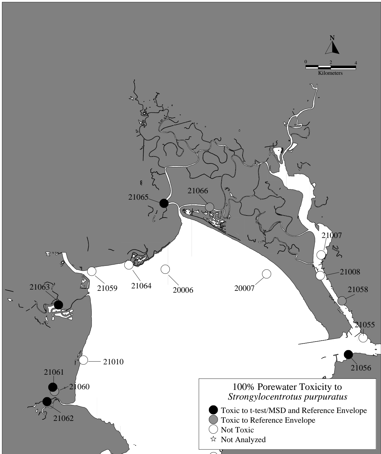
Figure 5b. Results of Porewater Toxicity Screening for Stations in San Pablo Bay.
