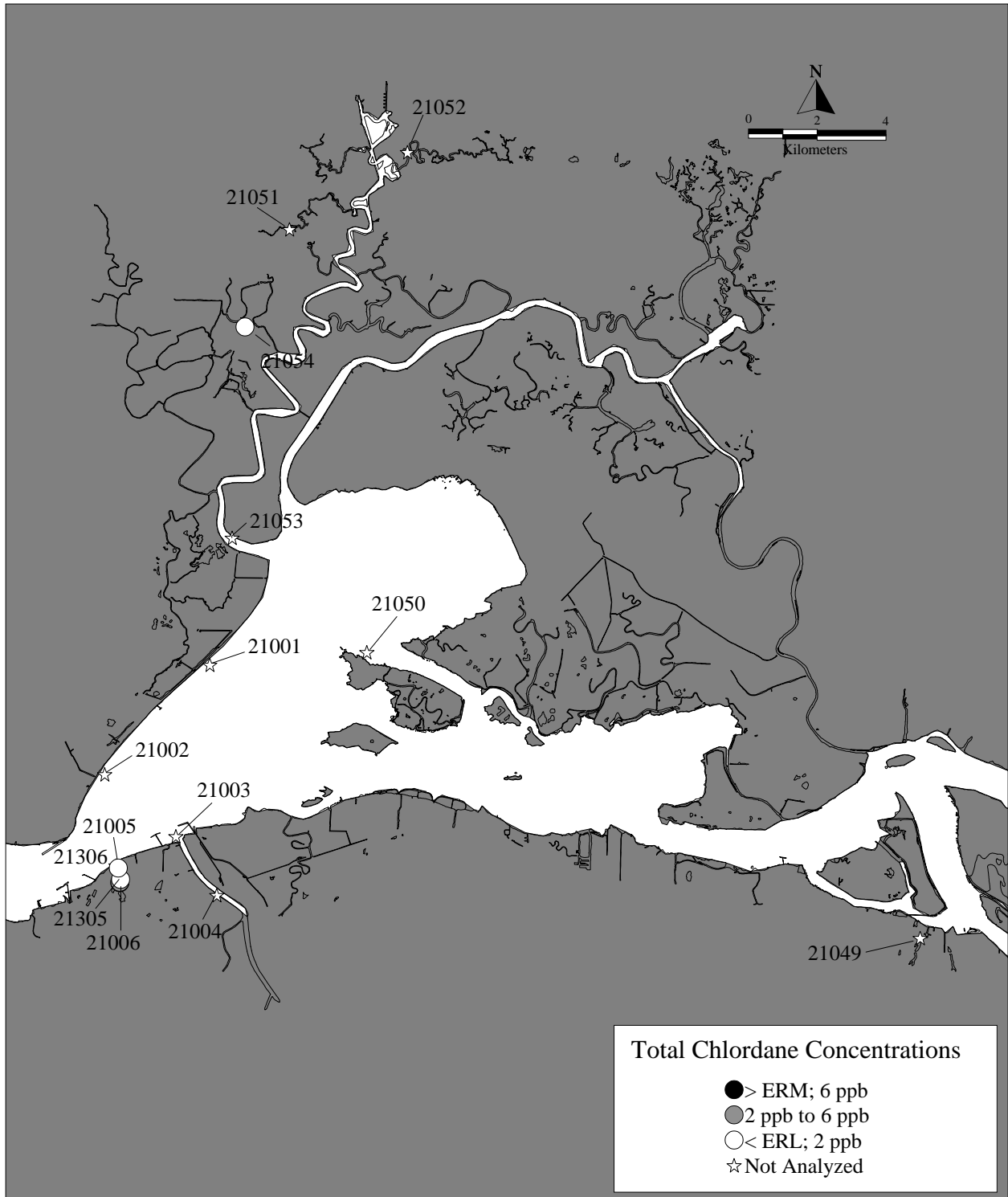
Figure 12a. Total Chlordane Concentrations at Stations in Suisun Bay.
