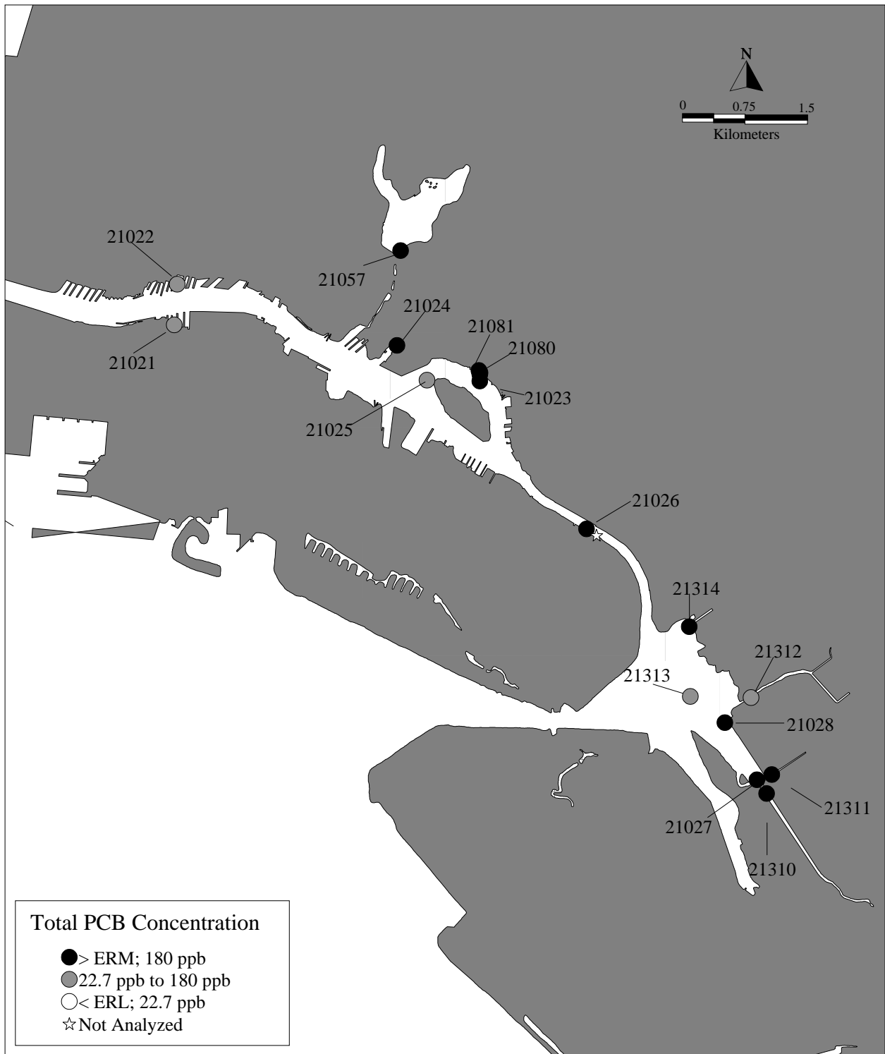
Figure 10e. Total PCB Concentrations at Stations in Oakland.
