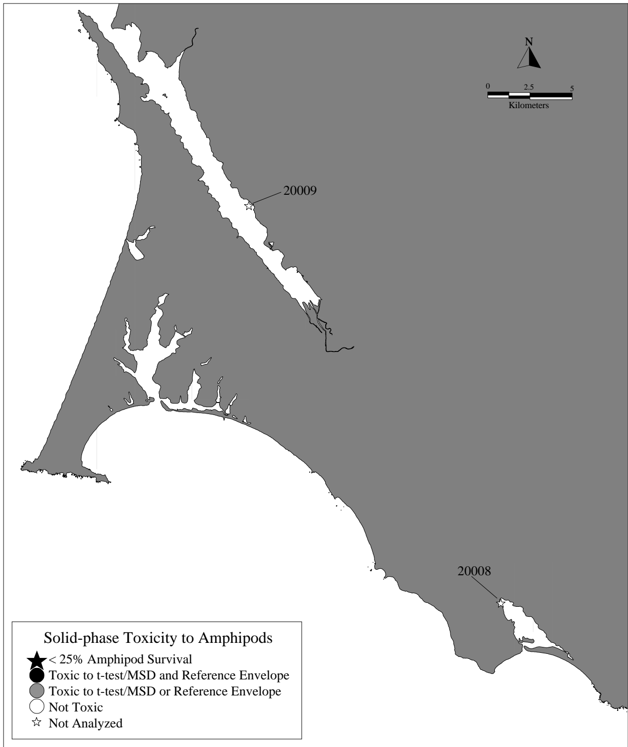
Figure 7g. Results of Amphipod Toxicity Confirmation for Stations in Tomales Bay and Bolinas Lagoon.
