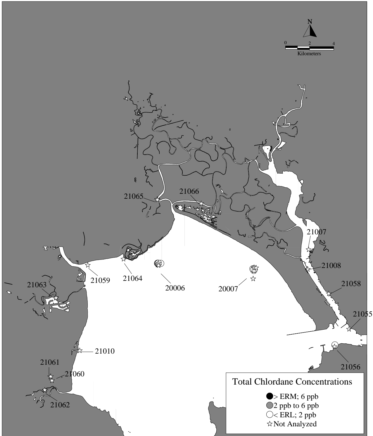
Figure 12b. Total Chlordane Concentrations at Stations in San Pablo Bay.
