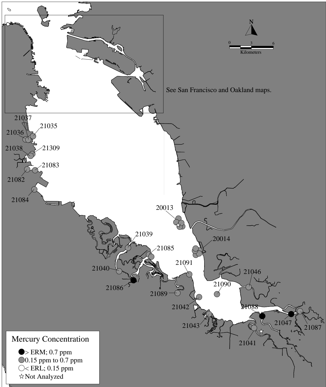
Figure 11d. Mercury Concentrations at Stations in South San Francisco Bay.
