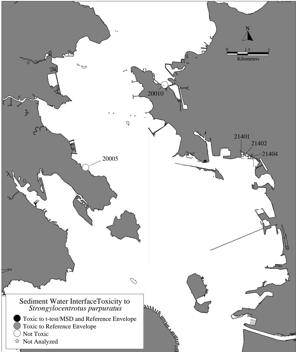
Figure 8c. Results of Sediment Water Interface Toxicity Confirmation for Stations in Central San Francisco Bay.
