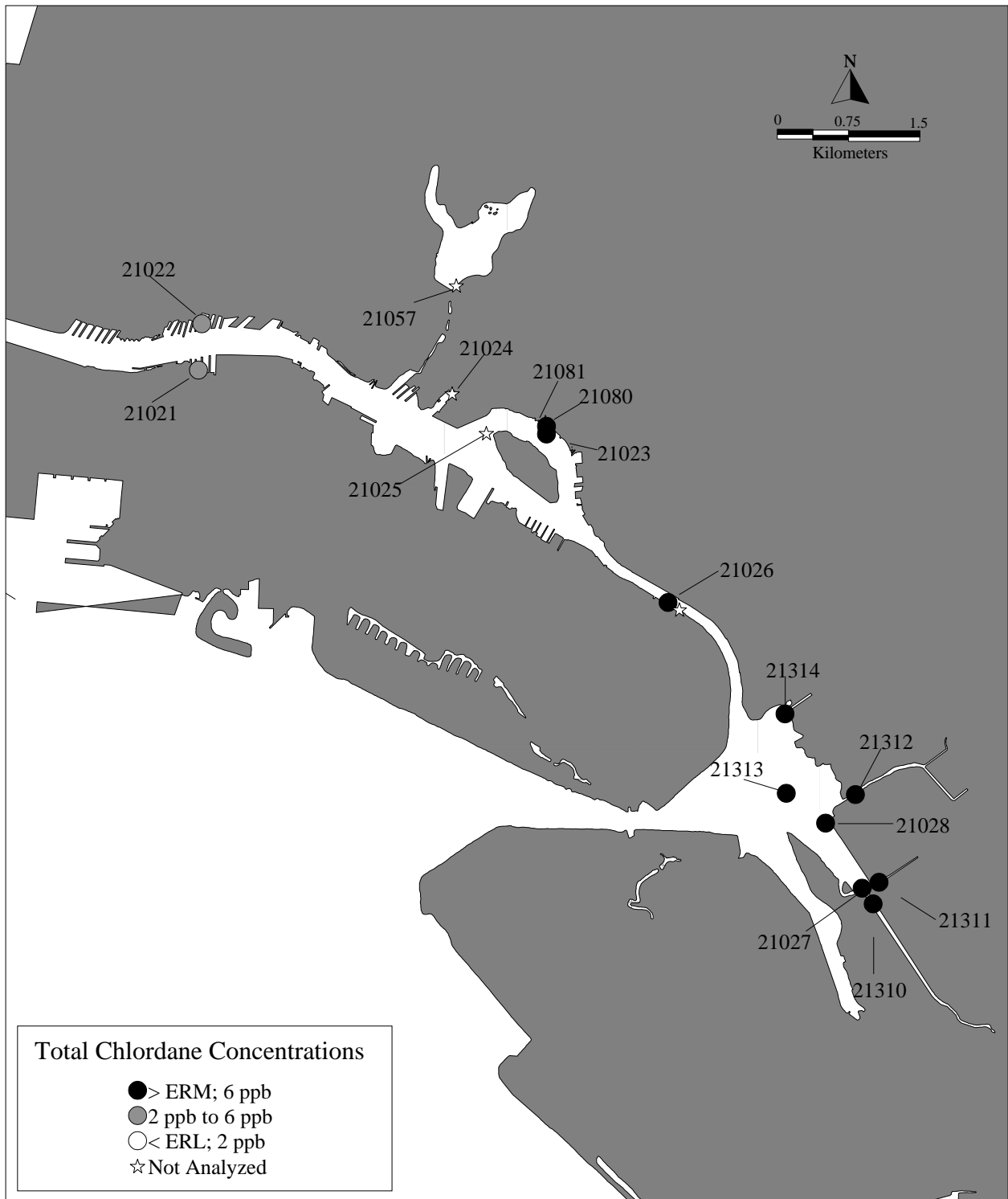
Figure 12e. Total Chlordane Concentrations at Stations in Oakland.
