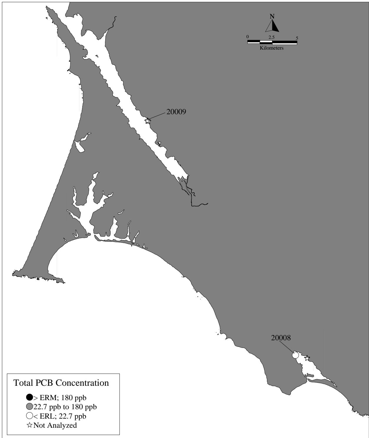
Figure 10g. Total PCB Concentrations at Stations in Tomales Bay and Bolinas Lagoon.
