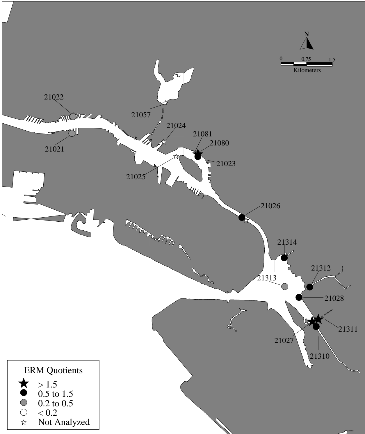
Figure 9e. Mean ERM Quotient Values for Stations in Oakland.
