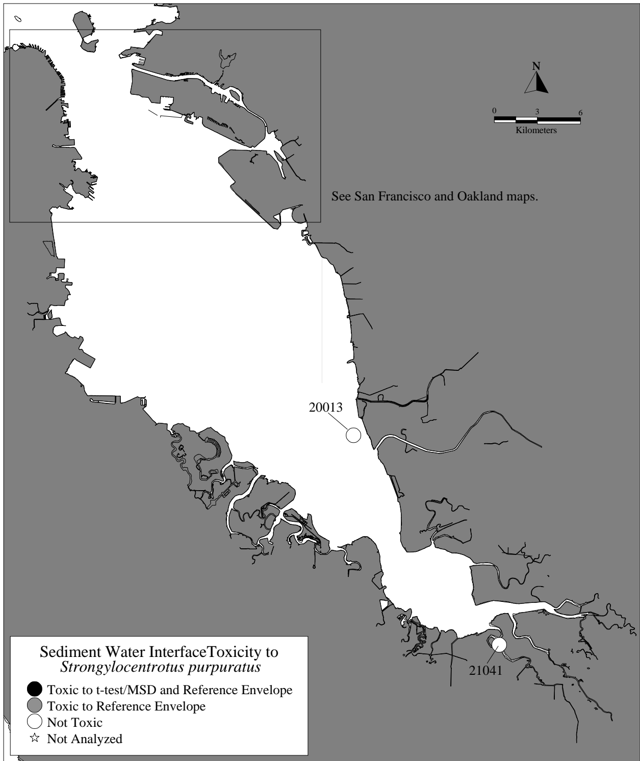
Figure 8d. Results of Sediment Water Interface Toxicity Confirmation for Stations in South San Francisco Bay.
