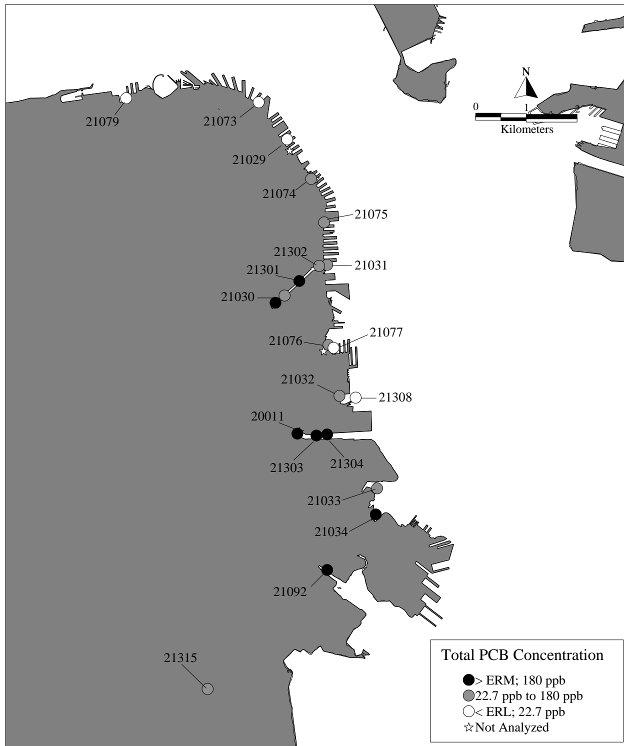
Figure 10f. Total PCB Concentrations at Stations in San Francisco.
