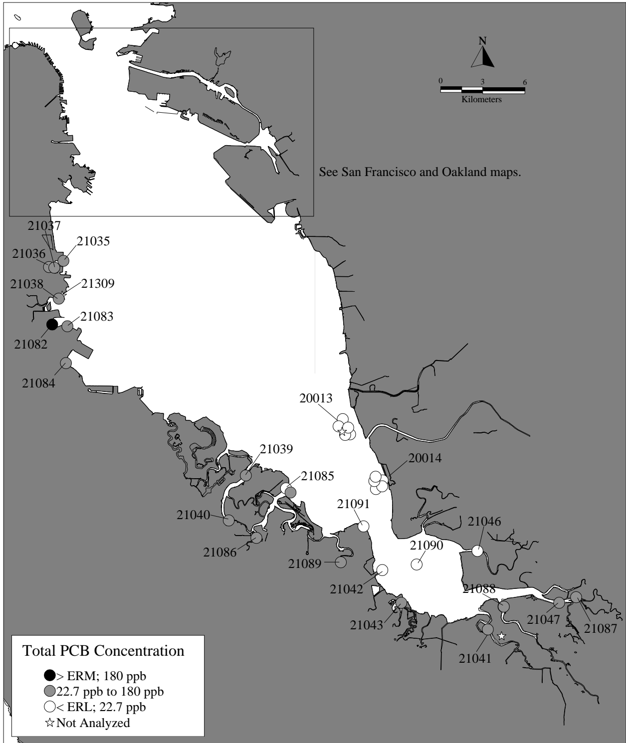
Figure 10d. Total PCB Concentrations at Stations in South San Francisco Bay.
