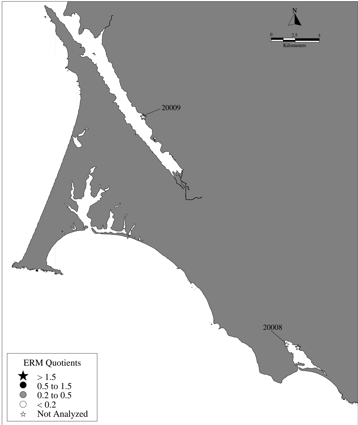
Figure 9g. Mean ERM Quotient Values for Stations in Tomales Bay and Bolinas Lagoon.
