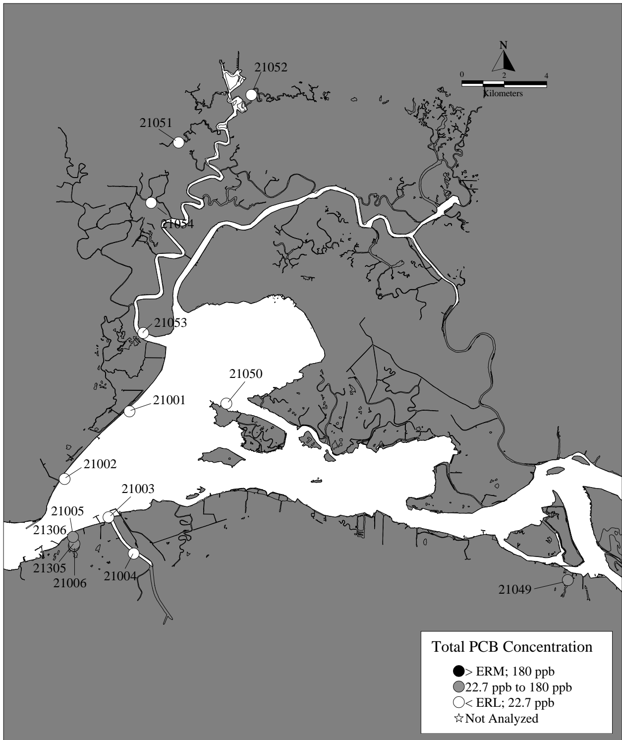
Figure 10a. Total PCB Concentrations at Stations in Suisun Bay.
