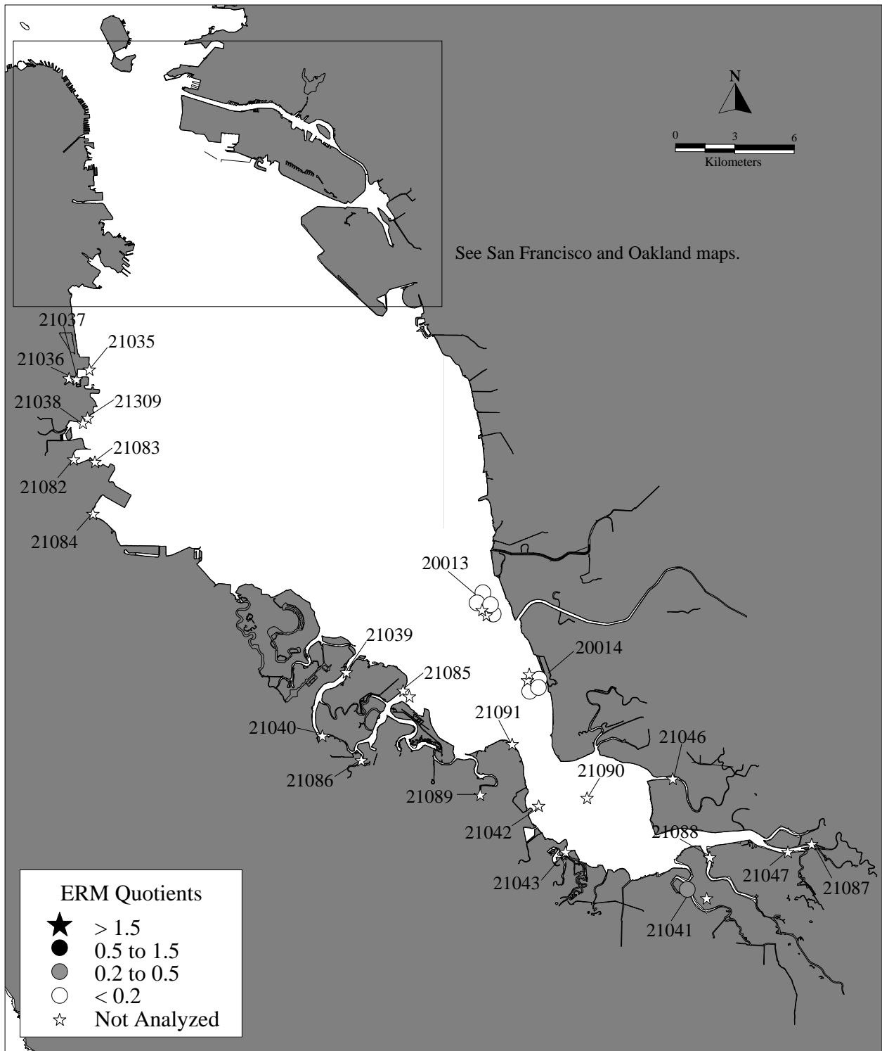
Figure 9d. Mean ERM Quotient Values for Stations in South San Francisco Bay.
