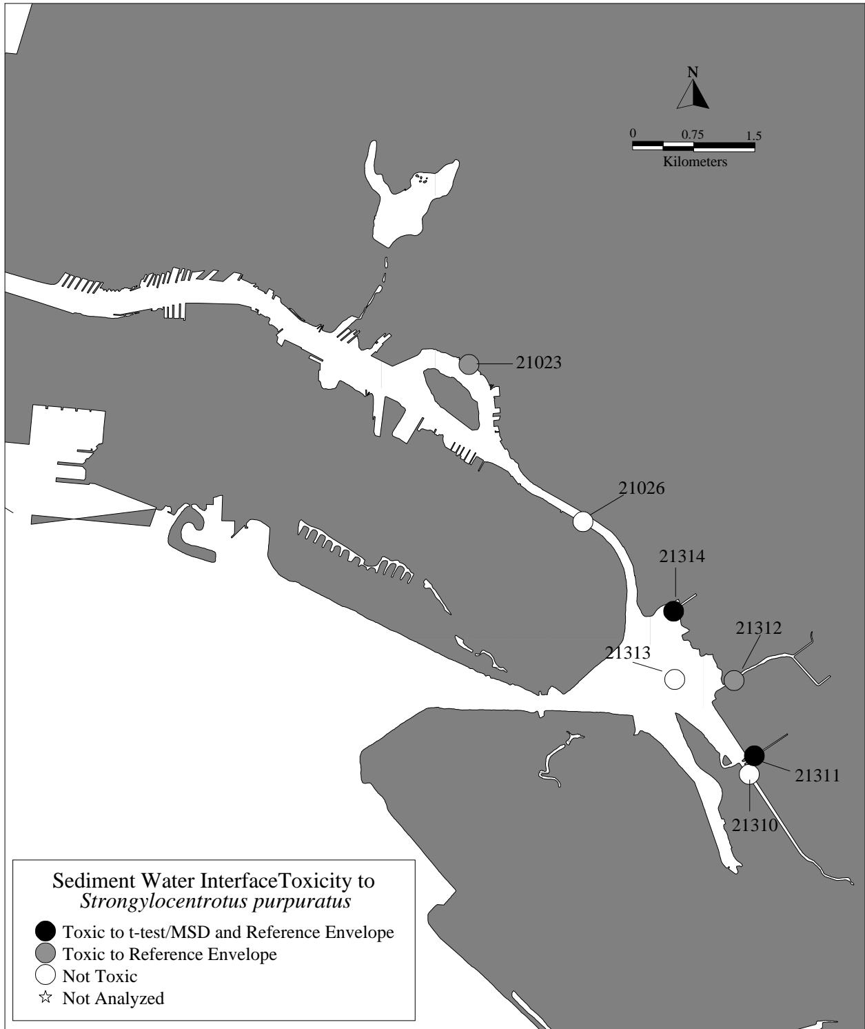
Figure 8e. Results of Sediment Water Interface Toxicity Confirmation for Stations in Oakland.
