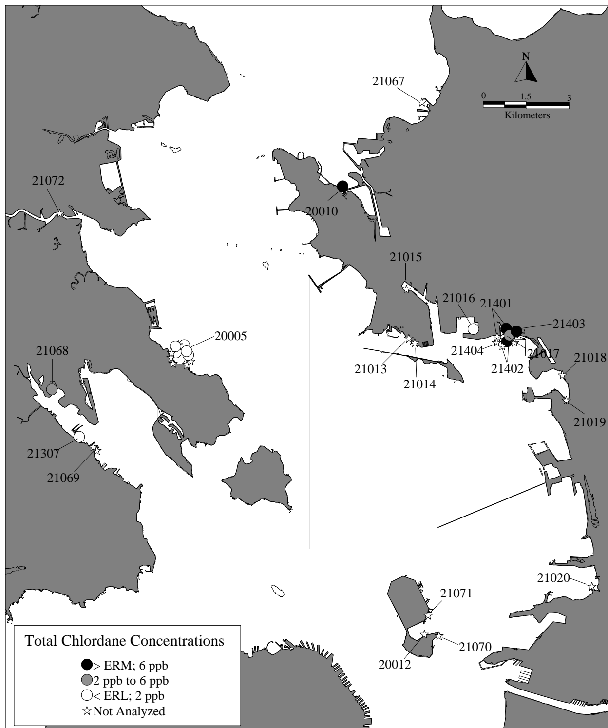
Figure 12c. Total Chlordane Concentrations at Stations in Central San Francisco Bay.
