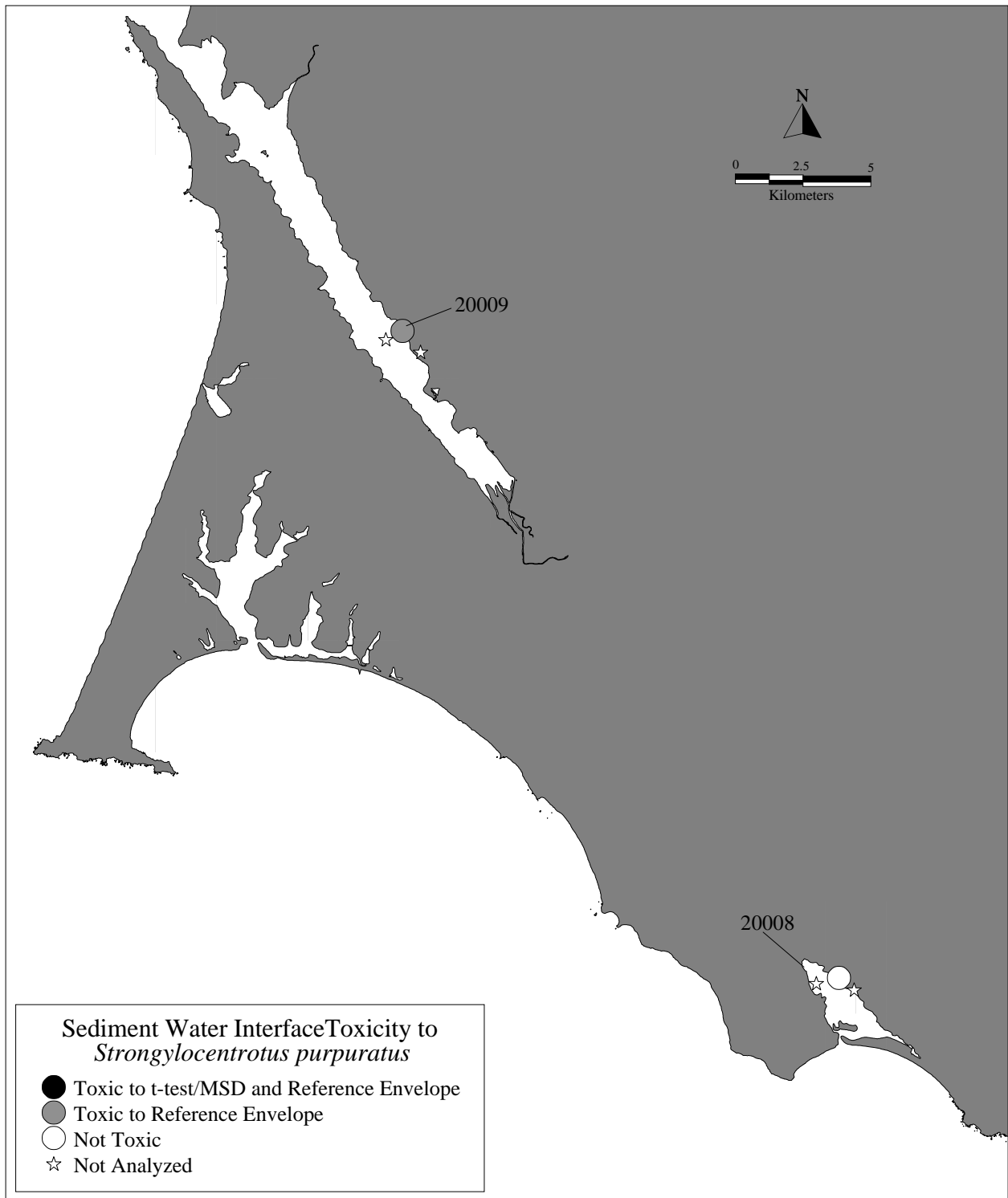
Figure 6g. Results of Sediment-Water Interface Toxicity Screening for Stations in Tomales Bay and Bolinas Lagoon.
