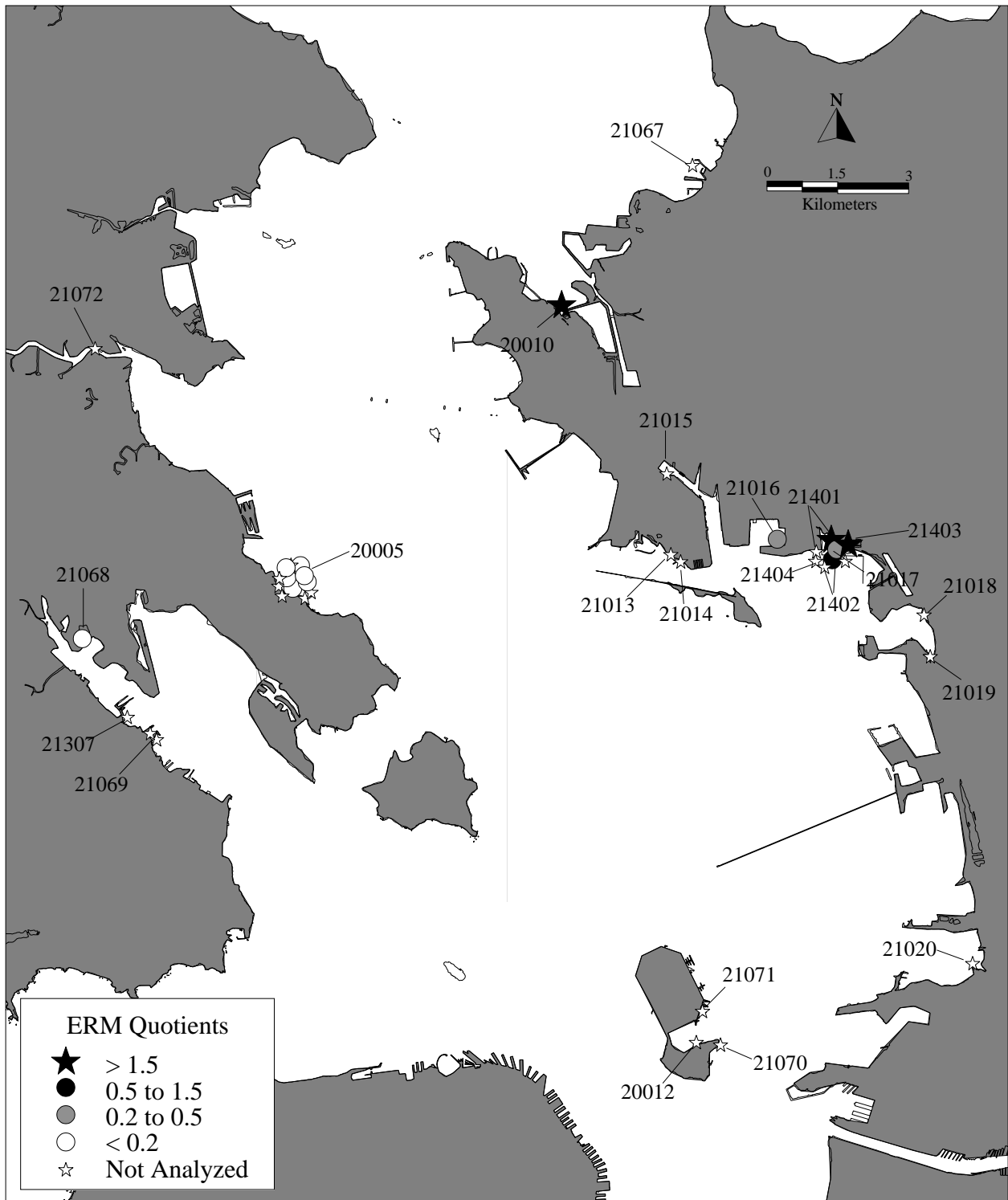
Figure 9c. Mean ERM Quotient Values for Stations in Central San Francisco Bay.
