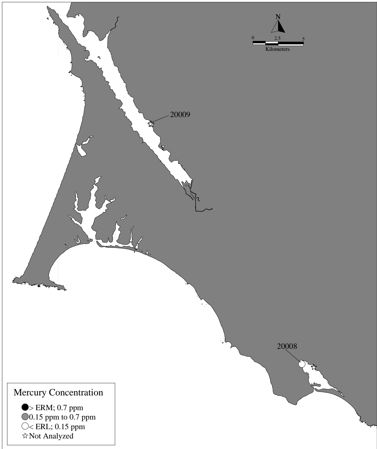
Figure 11g. Mercury Concentrations at Stations in Tomales Bay and Bolinas Lagoon.
