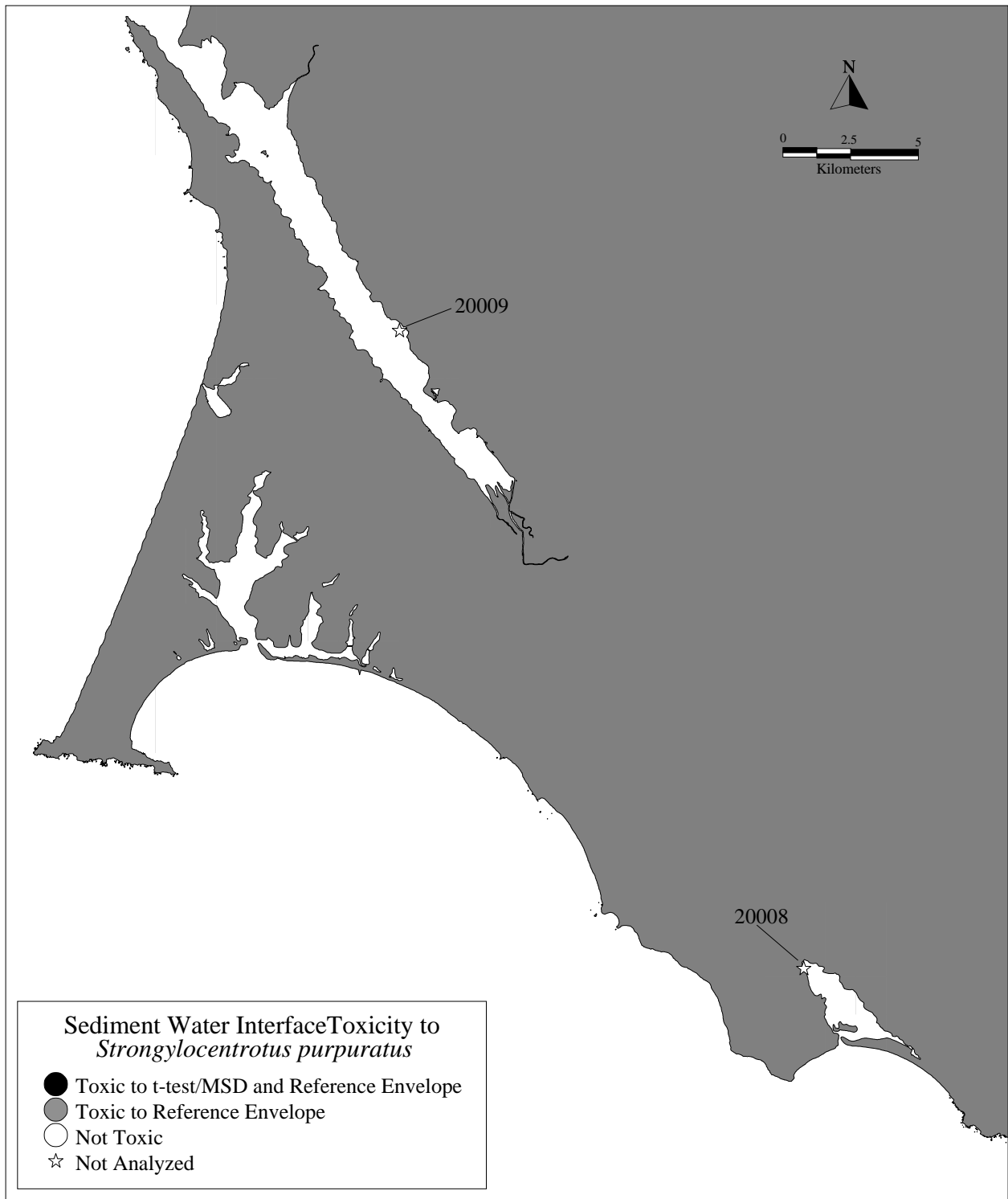
Figure 8g. Results of Sediment-Water Interface Toxicity Confirmation for Stations in Tomales Bay and Bolinas Lagoon.
