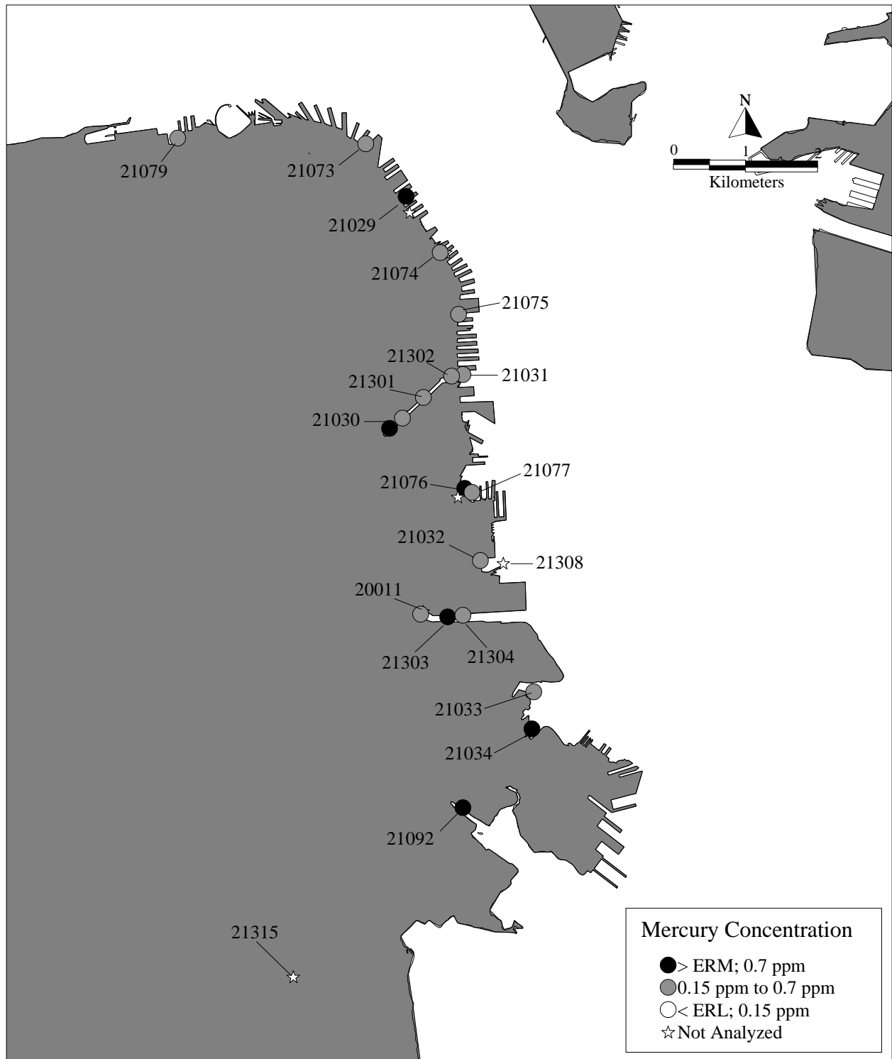
Figure 11f. Mercury Concentrations at Stations in San Francisco.
