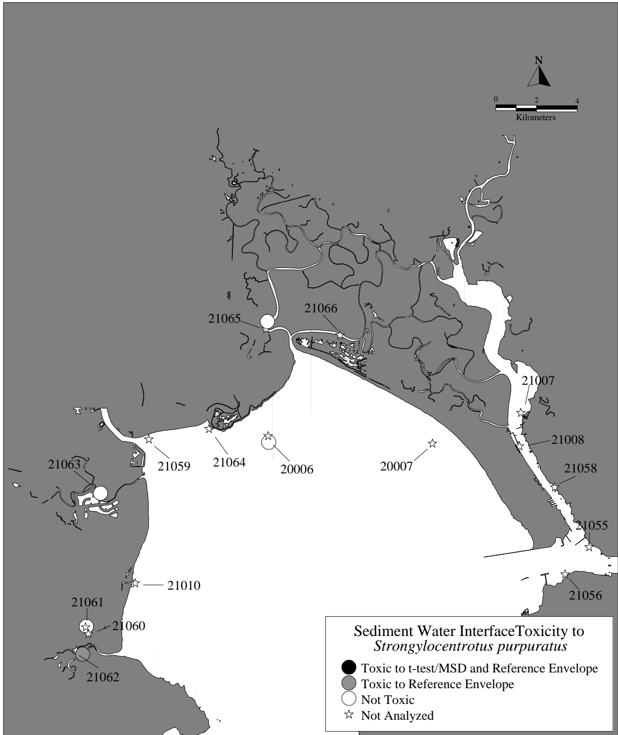
Figure 6b. Results of Sediment-Water Interface Toxicity Screening for Stations in San Pablo Bay.
