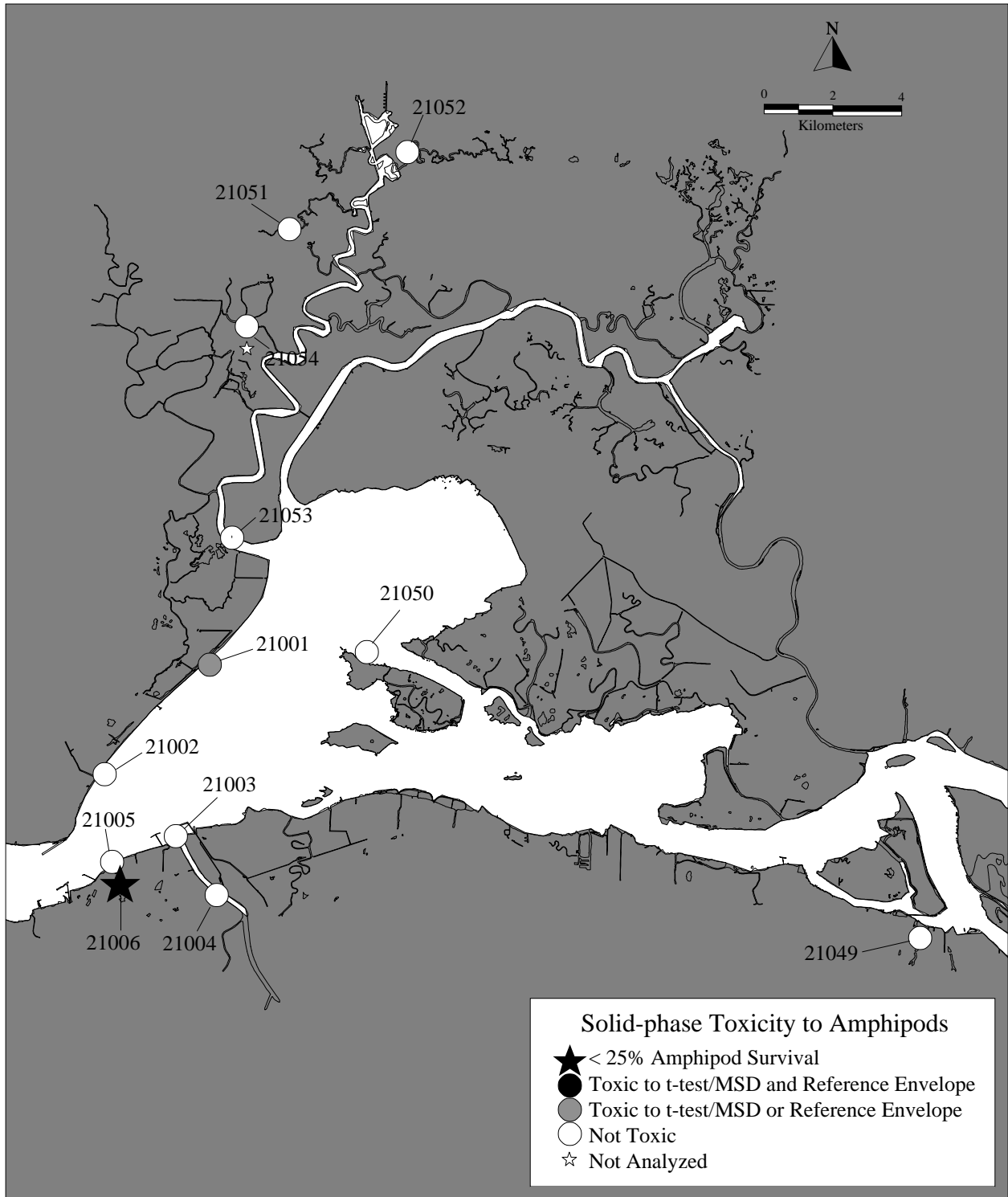
Figure 4a. Results of Amphipod Toxicity Screening for Stations in Suisun Bay.
