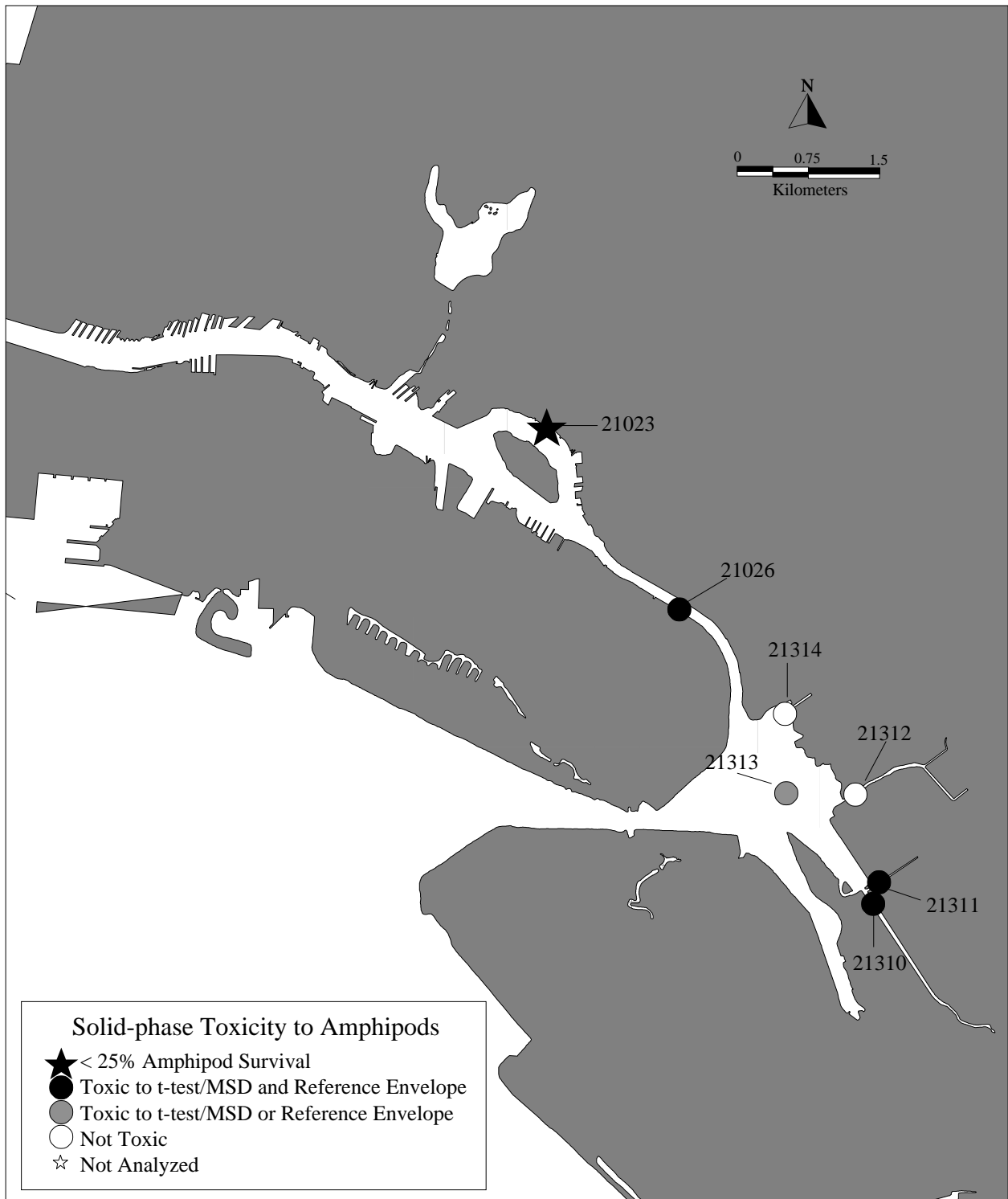
Figure 7e. Results of Amphipod Toxicity Confirmation for Stations in Oakland.
