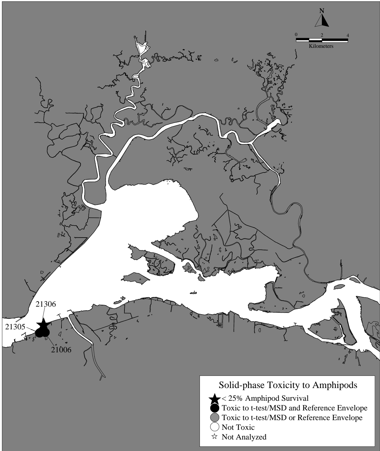
Figure 7a. Results of Amphipod Toxicity Confirmation for Stations in Suisun Bay.
