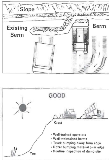
“Good” stockpiling method (top and side view).
