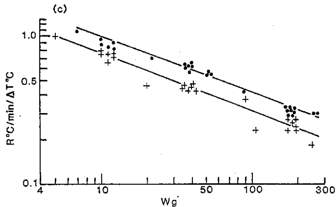
Fig. 7c Relationship between the exponential rate of change in body temperature ( R^\circ\text{C} per min per \Delta T^\circ\text{C} ) and the live weight of brown trout ( W\text{g} ) subjected to warming (●) and cooling (+).
