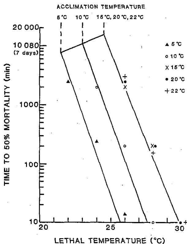
Fig. 2 Relationship between the time (min) for 50% mortality of brown trout, Salmo trutta , and the lethal temperature (°C) at different acclimation temperatures.
