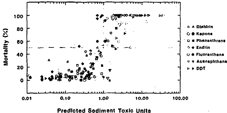
Figure 3.—Mortality versus predicted sediment toxic units. Predicted sediment toxic units are the ratio of the organic carbon-normalized sediment chemical concentration to the predicted sediment LC_{50} (Eqn. 8). Sediment types are indicated by the single hatching (lowest organic carbon content), cross-hatching (intermediate organic carbon content), and filled symbols (highest organic carbon content). See Tables 1 and 2 for data sources. K_{oc} values are computed from K_{ow} for DDT (5.84), endrin (4.84), fluoranthene (5.00), dieldrin (5.25), phenanthrene (4.46), and acenaphthene (3.76) with Equation 11. K_{ow} for DDT is the log average of the reported values in the Log P database [75]. The kepone K_{oc} is the log mean of the ratio of organic carbon-normalized kepone concentration to pore water-kepene concentration from the toxicity data set. K_{oc} s for the remaining compounds were computed by the U.S. EPA, Environmental Research Laboratory, Athens, Georgia. Methods are presented later in this document.
