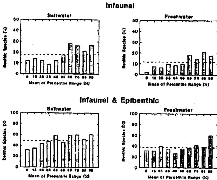
Figure 34.—Histograms of the proportion of saltwater and freshwater benthic organisms in 10 percentile groups of all normalized LC50s. If benthic organisms were as equally sensitive as water column organisms, the histograms should be of uniform height as indicated by the dashed line, the overall percentage of benthic species in the data set. Top panels include only infaunal organisms as benthic. The bottom panel includes infaunal and epibenthic as benthic organisms.
