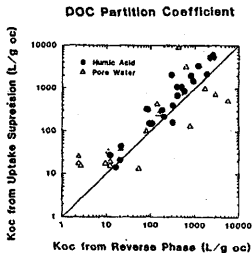
Figure 15.—Comparison of the DOC partition coefficient calculated from the suppression of chemical uptake versus the C_{18} reversed-phase HPLC column estimate. Circles are Aldrich humic acid; triangles are interstitial water DOC. Chemicals are listed in Figure 14 caption (also anthracene and benzo[a]anthracene).
