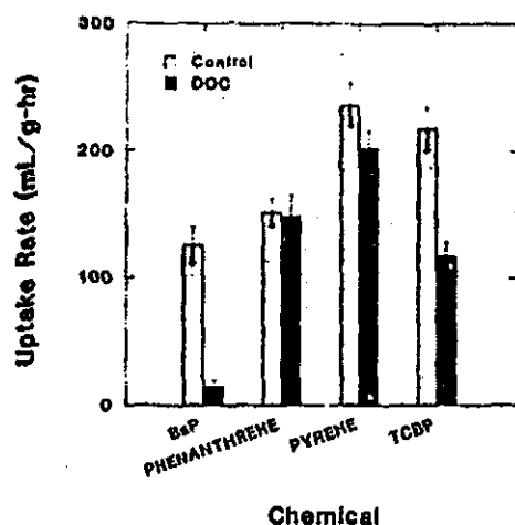
Figure 14.—Average uptake rate of chemicals by Pontoporeia hoyi with (filled) and without (hatched) DOC present. Benzo[a]pyrene (BaP); 2,2',4,4'-tetrachlorobiphenyl (TCDP); pyrene, phenanthrene. Data from Landrum et al. [42].
