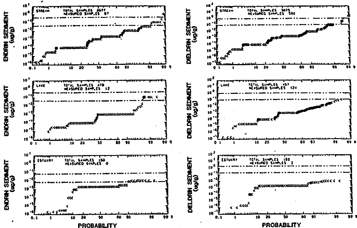
Figure 39.—Comparison of sediment quality criteria for sediments containing 1 percent and 10 percent organic carbon to the distributions of two sediment pesticide concentrations from the U.S. EPA STORET Database. Data are from 1986 to 1990. Samples above the detection limit (filled symbols) and samples less than the detection limit (less than symbols) are shown. Data from U.S. EPA [114].
