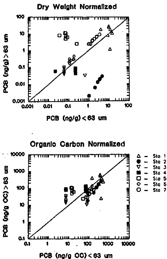
Figure 21.—Comparison of eight PCB congener concentrations of >63 \mu\text{m} sized particles, ordinate, to <63 \mu\text{m} sized particles, abscissa (Stations 1-7). Top panel is for dry weight normalization; bottom panel is for organic carbon normalization. PCB congeners are IUPAC Nos 28, 52, 101, 118, 138, 153, 179 and 180. Data from [47].
