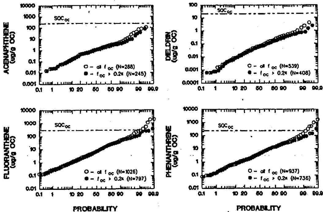
Figure 40.—Comparison of sediment quality criteria to the distributions of acenaphthene, fluoranthene, dieldrin, and phenanthrene organic carbon normalized sediment concentrations from NOAA's National Status and Trends Program. Data are from 1984 to 1989. Samples with organic carbon greater than 0.2 percent (filled symbols) and samples for all organic carbon contents (open symbols) are shown. Data from NOAA [47].
