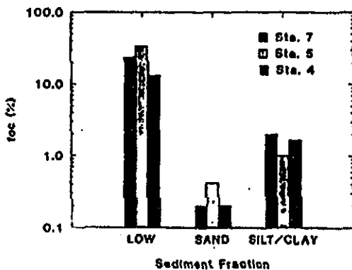
Figure 16.—The organic carbon fractions (% dry weight) in the low-density fraction ( 64 \mu\text{m} , <1.9 \text{ g/cm}^3 ); the sand-sized fraction ( >64 \mu\text{m} , >1.9 \text{ g/cm}^3 ); the silt/clay-sized fraction ( <64 \mu\text{m} ). Numbered stations as indicated. Data from [44].
