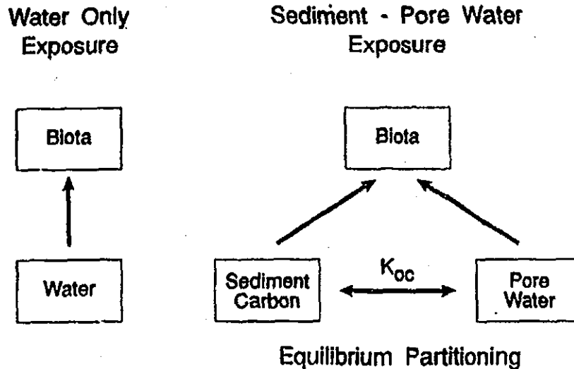
Figure 2.—Diagram of the organism exposure routes for a water-only exposure (left) and a sediment exposure (right). Equilibrium partitioning refers to the assumption that an equilibrium exists between the chemical sorbed to the particulate sediment organic carbon and the pore water. K_{oc} is the organic carbon partition coefficient.
