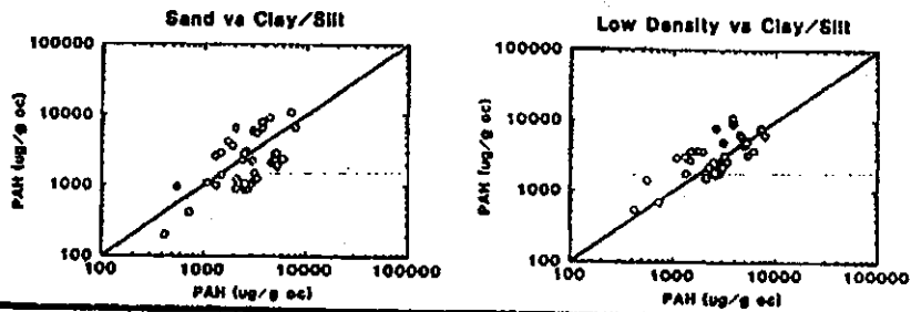
Figure 17.—Comparison of PAH concentrations of the sand-sized- and low-density-fraction sediment particles ordinate to the clay/silt fraction abscissa (Stations 4, 5, 7). Top panels are for dry weight normalization; bottom panels are for organic carbon normalization. Data from [44].
