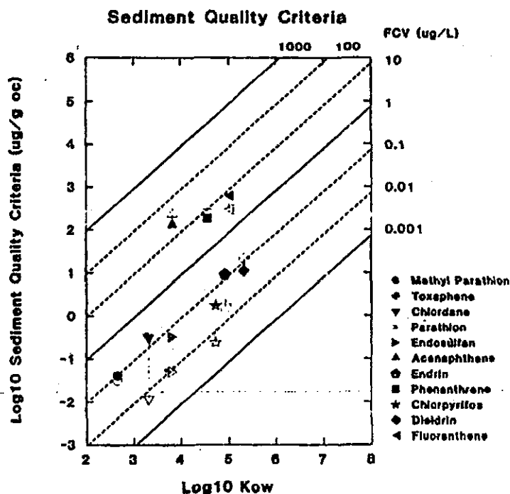
Figure 37.—Log 10 SQC versus log 10 K ow . The diagonal lines indicate the FCV values. The criteria are computed from Equation 34. K oc is obtained from K ow with Equation 11. The symbols indicate SQC oc for the freshwater (filled) and saltwater (hatched) criteria for the listed chemicals. The vertical line connects symbols for the same chemical. The FCVs for methyl parathion, toxaphene, chlordane, parathion are from WQC or draft documents, see Table 4. The FCVs for acenaphthene, endrin, phenanthrene, fluoranthene and dieldrin are computed as part of the development of SQC. The octanol/water partition coefficients for methyl parathion, toxaphene, chlordane, parathion, endosulfan and chlorpyrifos are the log mean of the values reported in the Log P database [75]. The K ows for acenaphthene, endrin, phenanthrene and dieldrin are those measured from the slow stir flask method.
