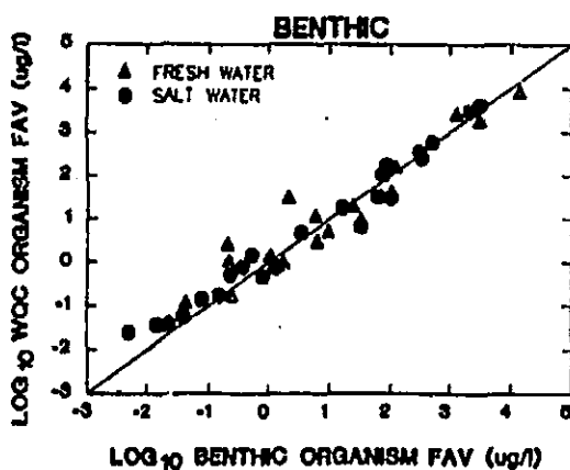
Figure 4.—A comparison of the final acute values (FAV) for water column versus benthic organisms. Each data point represents an FAV for a particular chemical in either a freshwater or a saltwater exposure. The data are from the WQC or draft criteria documents. See Table 4 for data sources.
