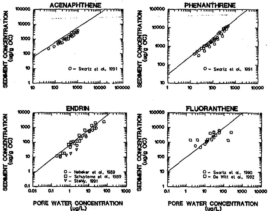
Figure 24.—Comparison of organic carbon partition coefficient ( K_{oc} ) observed in toxicity tests (symbols) to K_{oc} derived from laboratory K_{ow} and Equation 11 (solid line). Symbols are sediment concentration, ordinate, versus pore water concentration, abscissa. Solid line is C_{s,oc} = K_{oc} \cdot C_p , where \text{Log}_{10} K_{oc} is 3.76 for acenaphthene, 4.84 for endrin, 4.46 for phenanthrene, and 5.00 for fluoranthene. These \text{Log}_{10} K_{oc} values are estimated from \text{Log}_{10} K_{ow} values measured at the U.S. EPA Environmental Research Laboratory at Athens, Georgia. Data sources as indicated.
