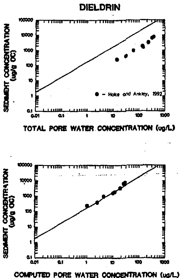
Figure 25.—Comparison of organic carbon partition coefficient ( K_{oc} ) observed in toxicity tests (symbols) to K_{oc} derived from laboratory K_{ow} and Equation 11 (solid line). Symbols are sediment concentration, ordinate, versus total (top panel) and free (bottom panel) pore water concentrations, abscissa. Solid line is C_{s,oc} = K_{oc} \cdot C_f , where \log_{10} K_{oc} is 5.25 for dieldrin. The \log_{10} K_{oc} value is estimated from \log_{10} K_{ow} value measured at the U.S. EPA Environmental Research Laboratory at Athens, Georgia. Data source as indicated.
