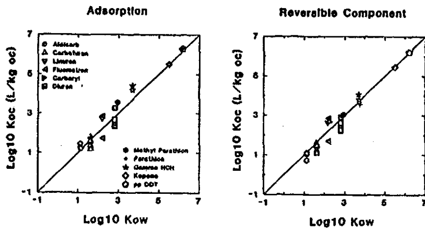
Figure 10.—Comparison of the adsorption (left) and reversible component (right) organic carbon-normalized partition coefficient, K_{oc} , to the octanol/water partition coefficient, K_{ow} , for experiments with low solids concentrations: m_{oc}K_{ow} < 1 . The line represents equality [27].
