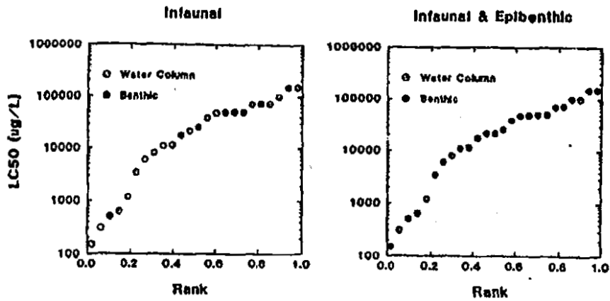
Figure 33.—LC50s versus rank for nickel in seawater. Infaunal organisms (left) and infaunal and epibenthic (right) are identified by the solid symbols. The plot illustrates the distribution of benthic organisms in the overall species sensitivity distribution.
