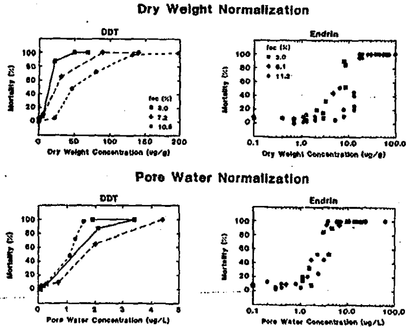
Figure 7.—Comparison of percent mortality of H. azteca to DDT (left) and endrin (right) concentrations in bulk sediment (top) and pore water (bottom) for sediments with varying organic carbon concentrations [20, 21].
