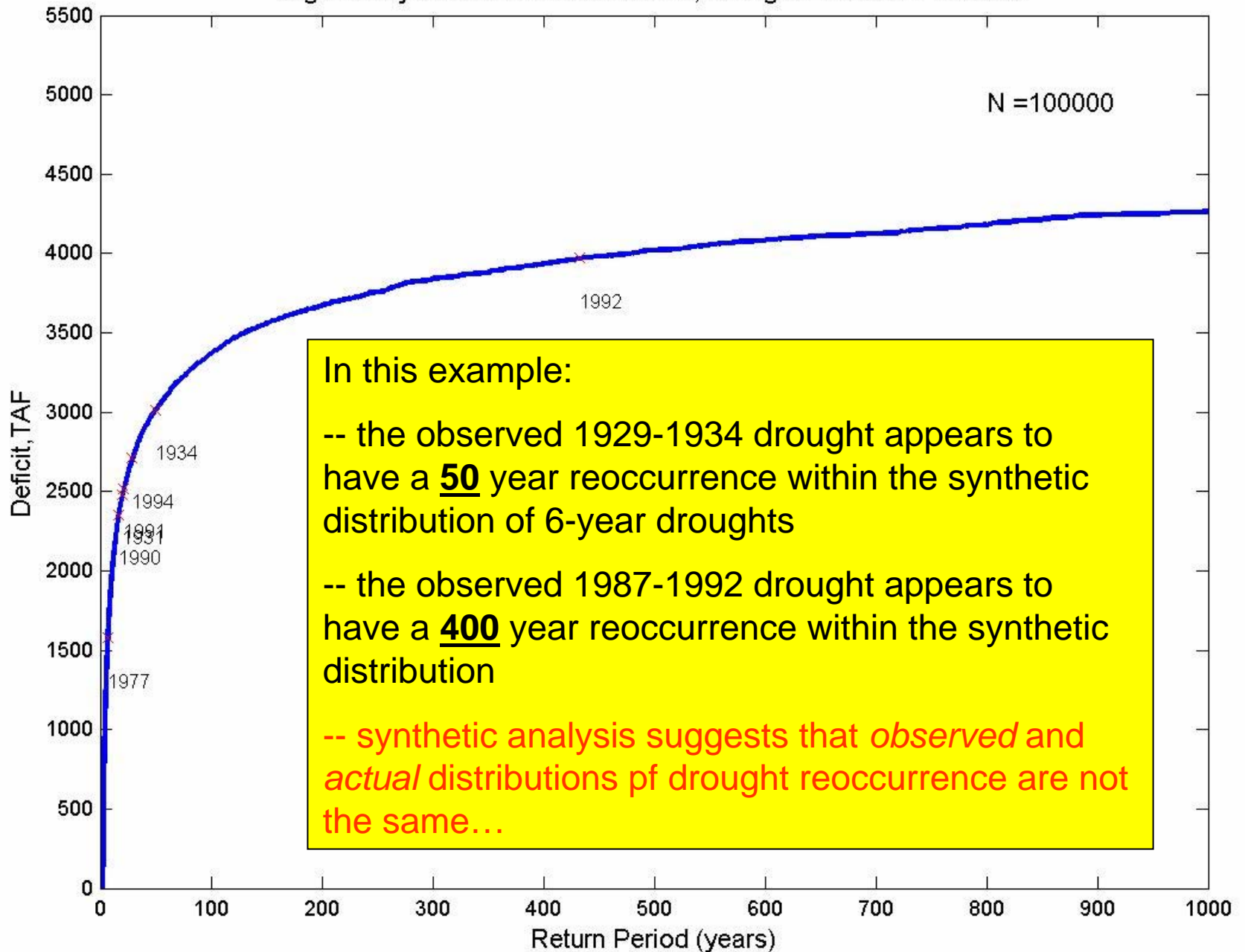
Fig.A19-Synthetic:Six-Year Duration, Drought End-Years Labeled
