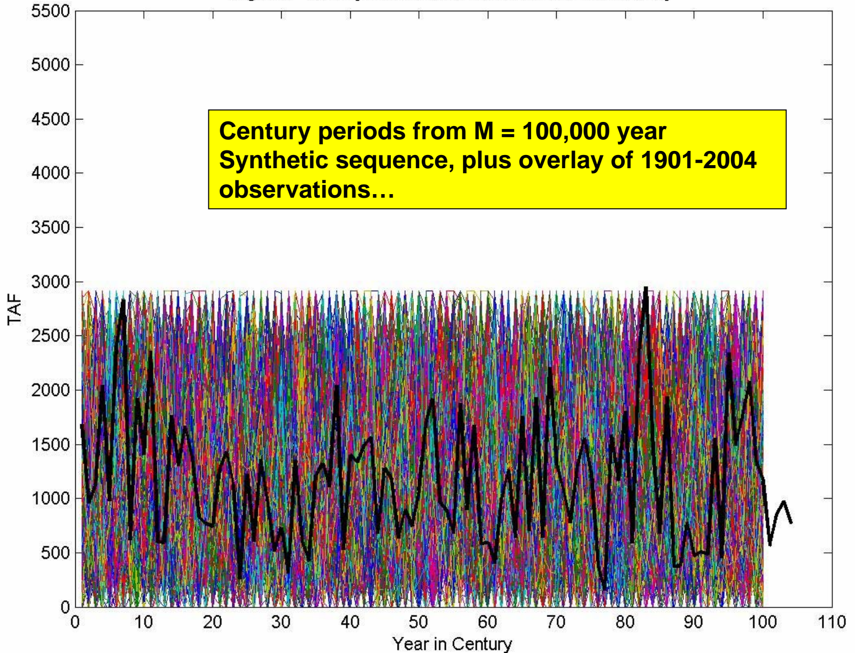
Fig.A12 - 200 Synthetic Centuries and Observed Overlay
