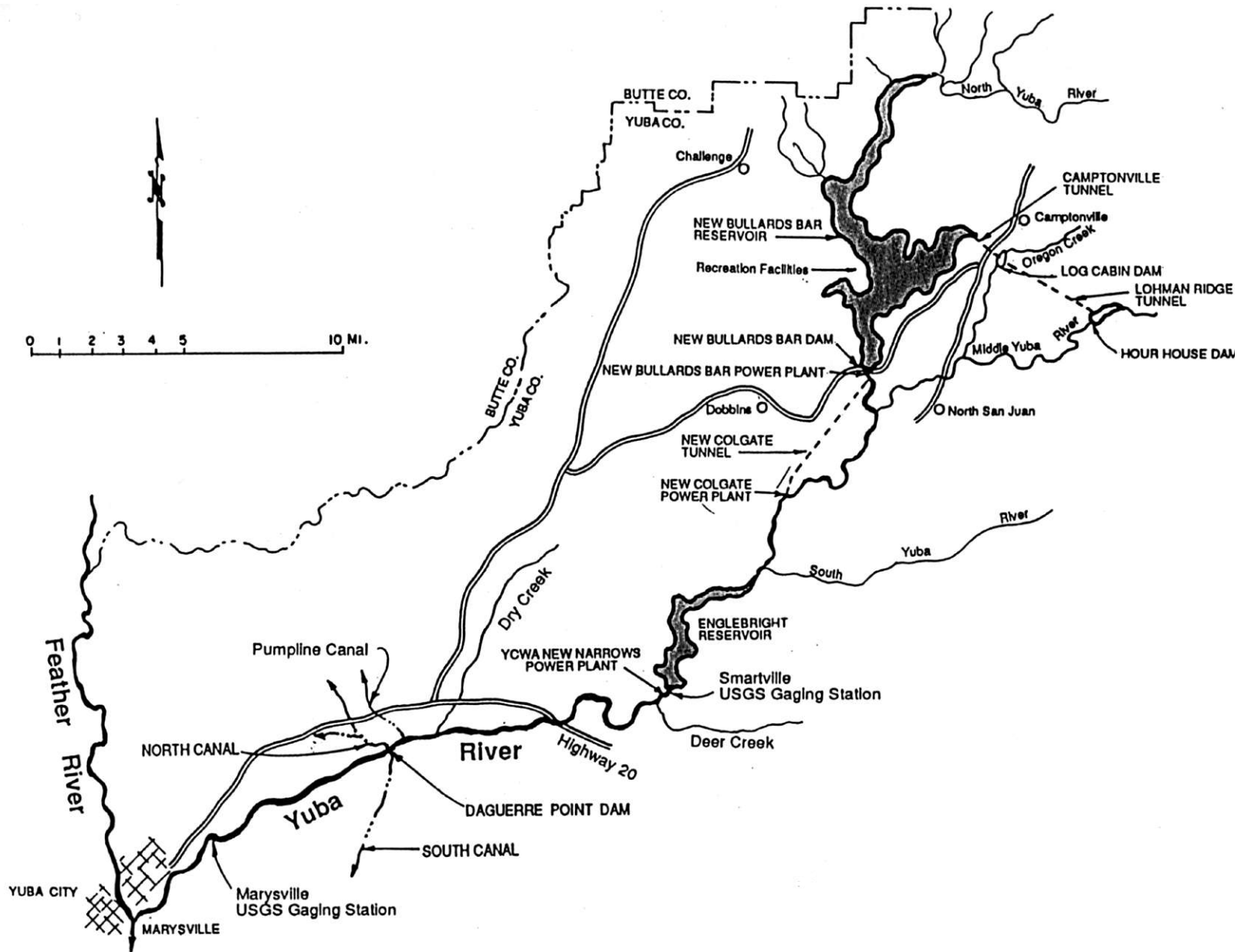
FIGURE 1 Yuba River Development Project
