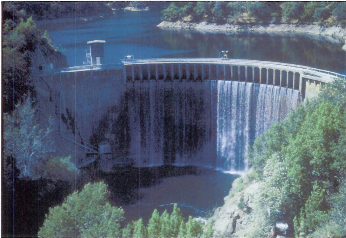
Looking upstream toward the downstream face of San Clemente Dam – outlet tower is to the left of the spillway (July 1982)
