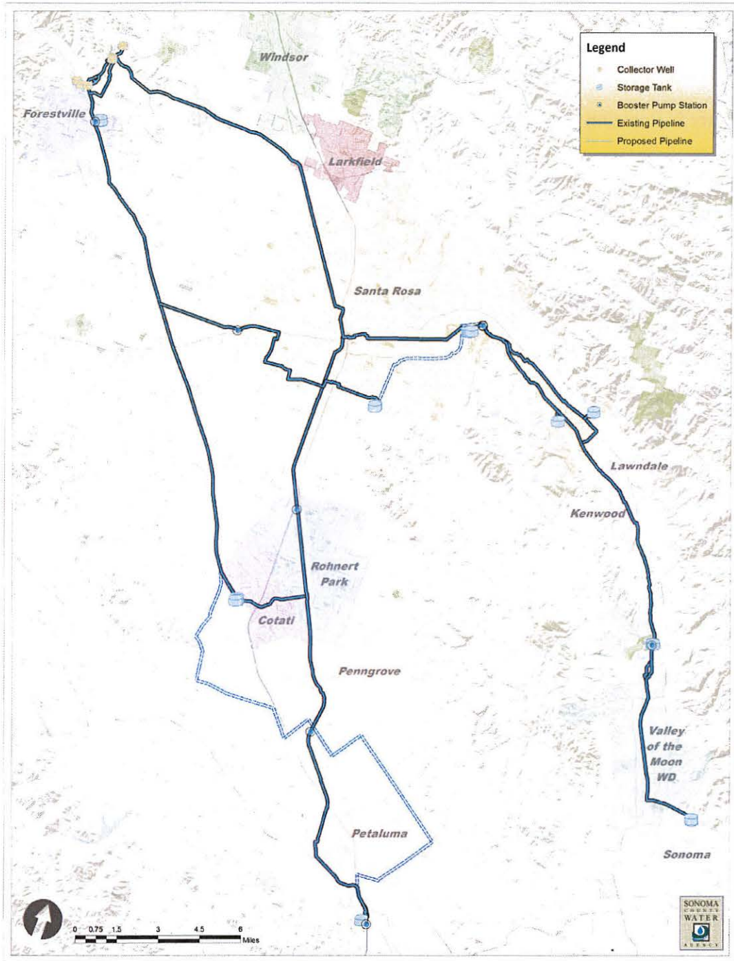
Figure 1. Water Transmission System – Existing and Proposed Facilities
