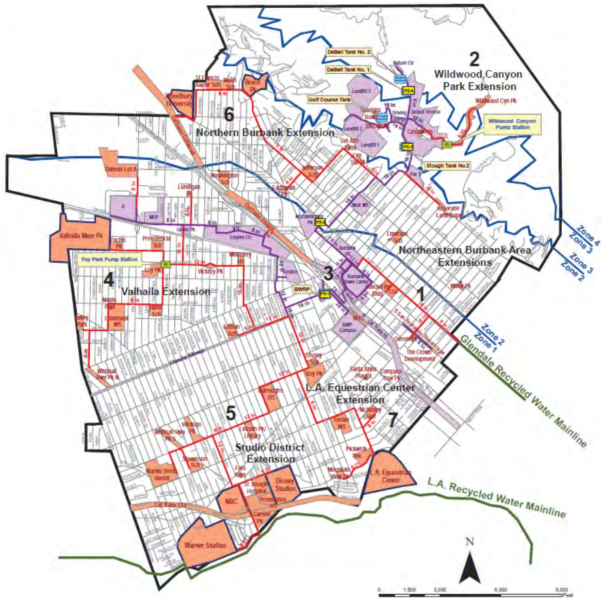
FIGURE 2 – EXISTING & POTENTIAL RECYCLED WATER USERS
