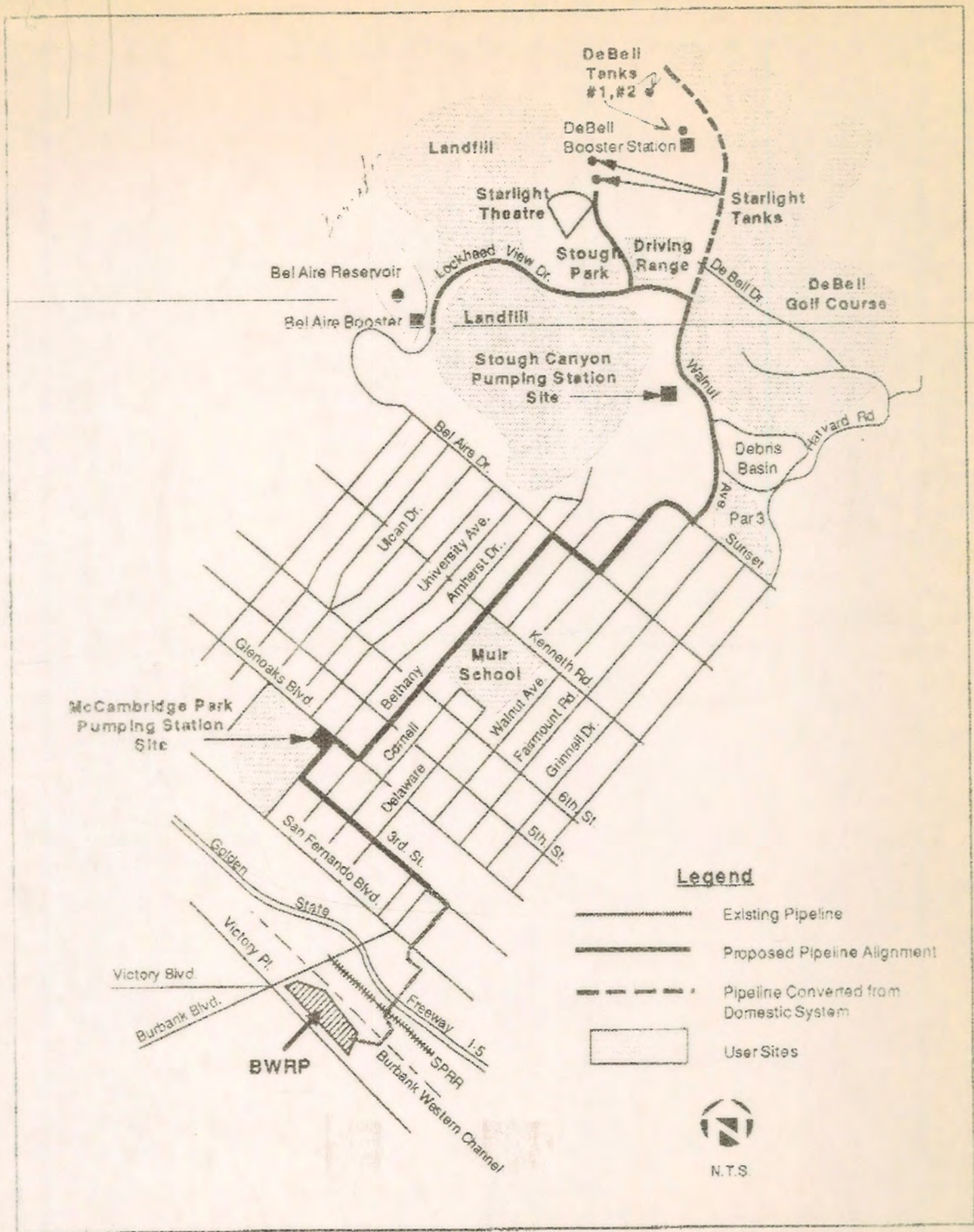
Proposed Project Facilities Figure 1-2
