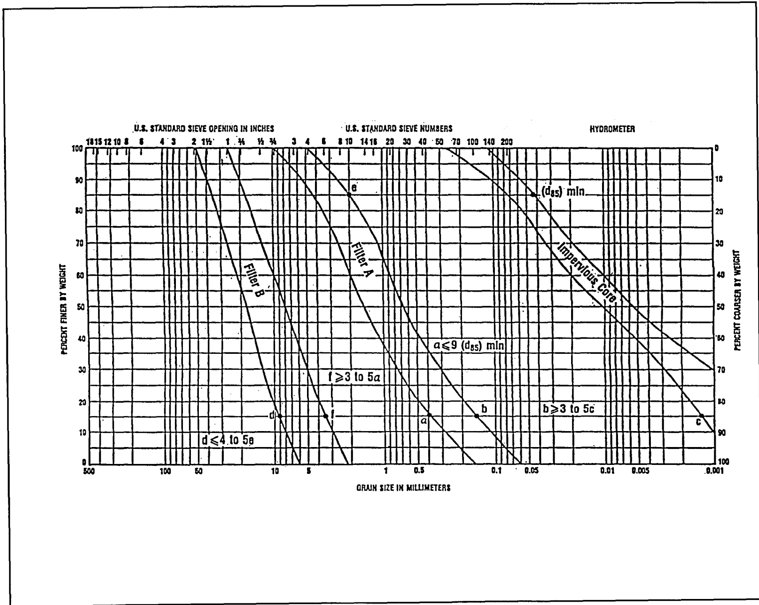
Figure D-2. Illustration of the design of a graded filter
