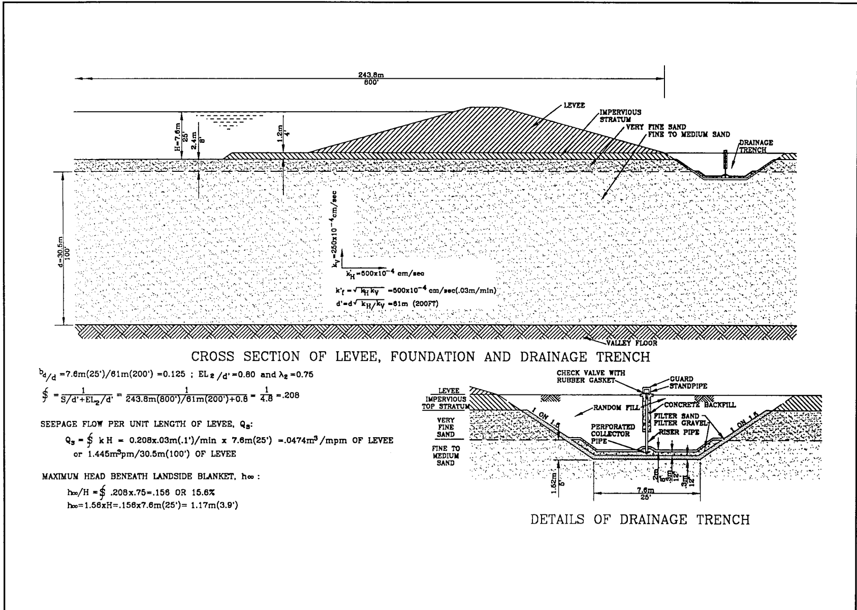
Figure E-2. Example of design of a drainage trench
