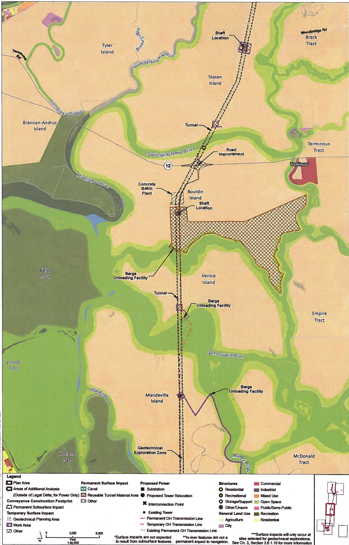
Figure M13-4: Sheet 4 of 8 General Plan Land Use Designations — Modified Pipeline/Tunnel Alignment (Alternative 4)
