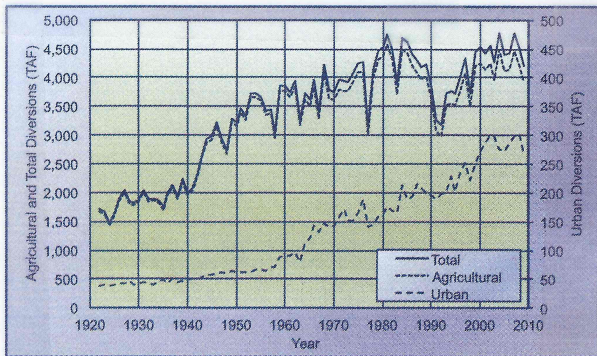
Figure 3-19 Estimated Annual Diversions in the Sacramento Valley
