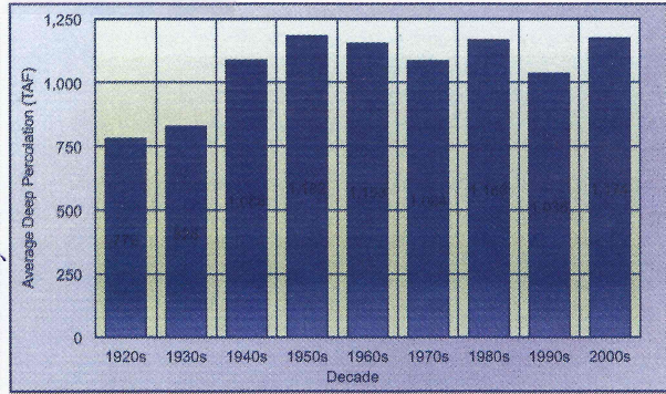
Figure 3-27 Estimated Average Annual Deep Percolation by Decade in the Sacramento Valley
