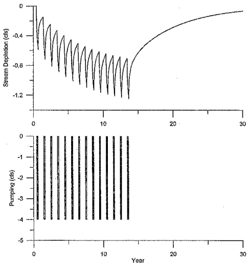
Figure 6. Stream depletion caused by an ensemble of wells (shown in Figure 5). The wells are pumping collectively 4.0 cfs for 3 months each year for 15 years and then pumping stops. (from Bredehoft, 2011)
