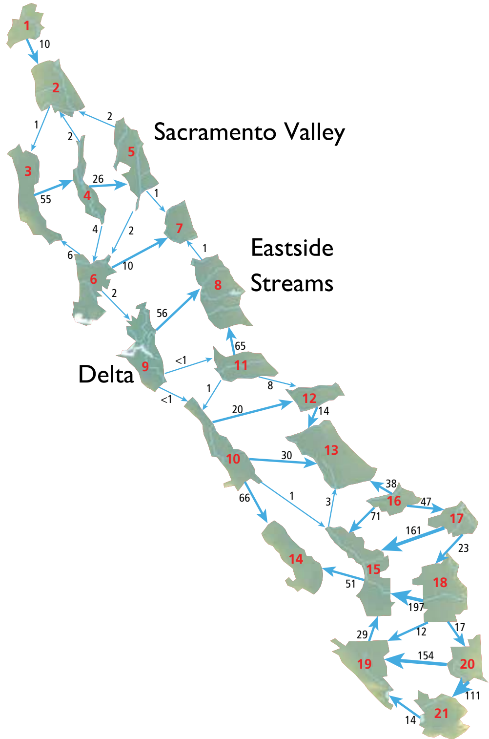
Figure 81B. Simulated average annual subsurface flows between subregions, 1960-1969.
