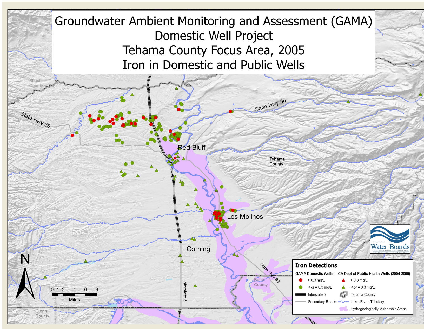
Figure 5: Iron Concentrations
