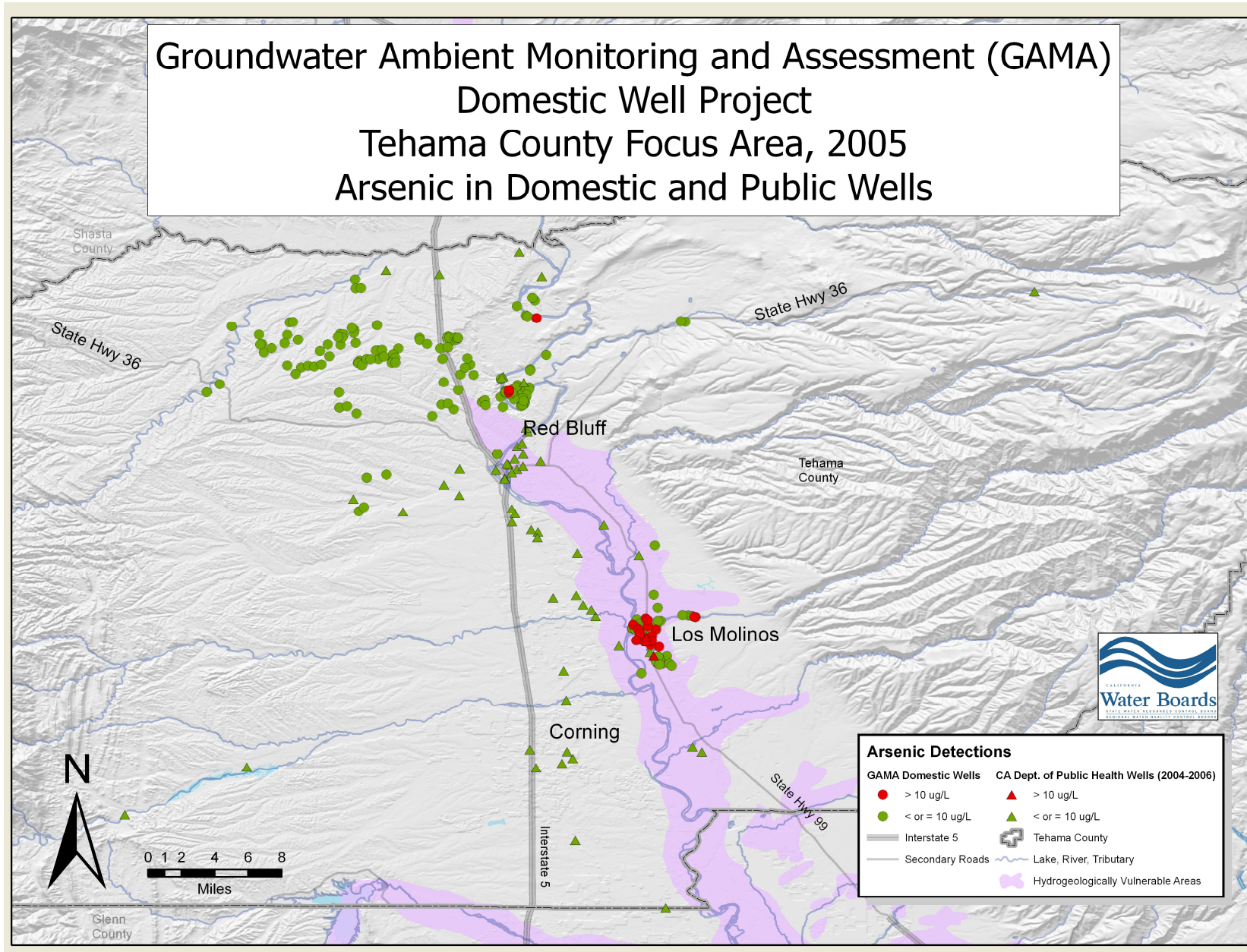
Figure 4: Arsenic Concentrations
