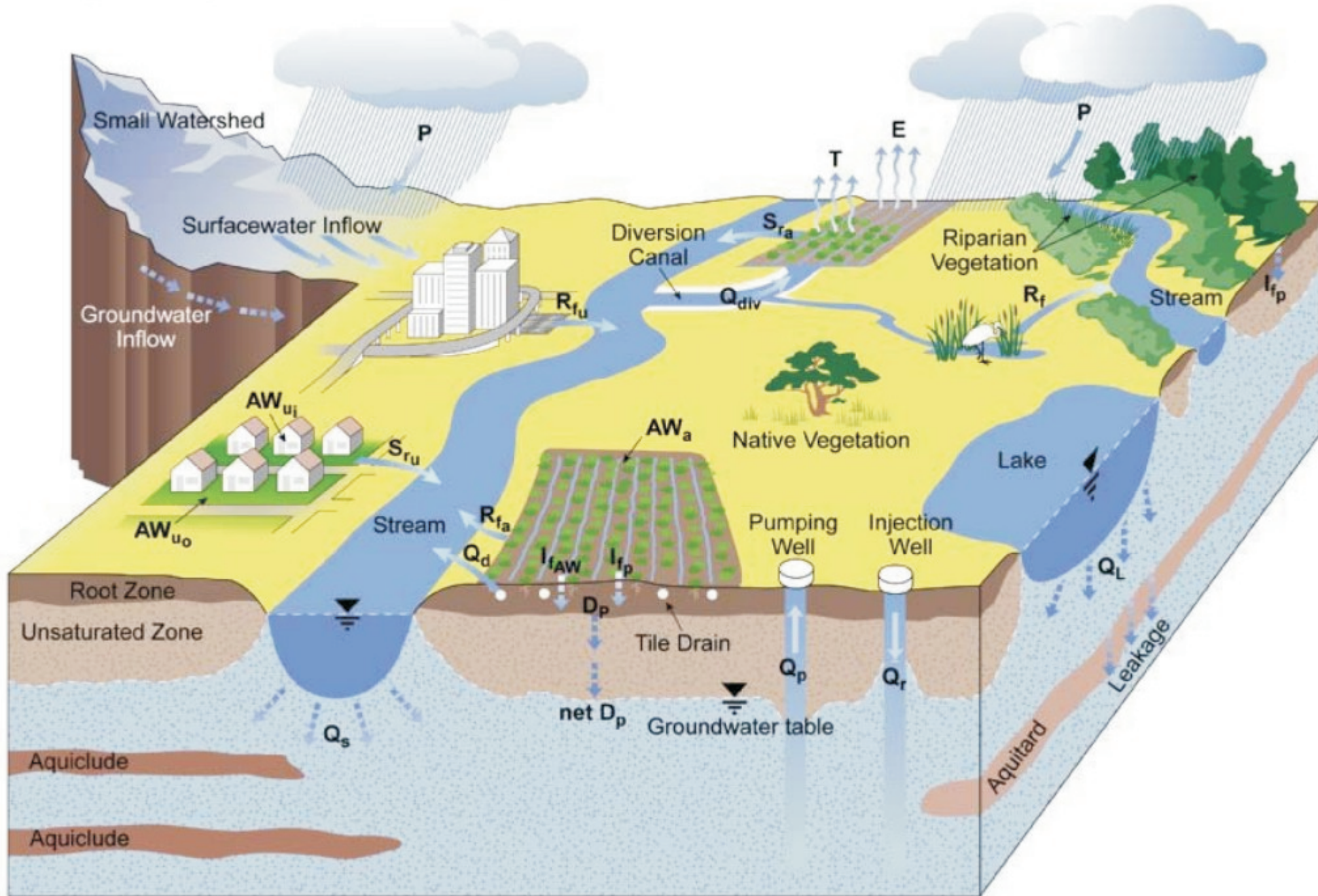
Figure 11. Integrated Water Flow Model components.
